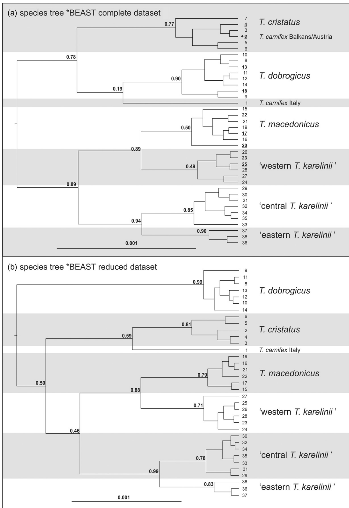
Fig. 4. Species tree resulting from the *BEAST multi-species coalescent analysis based on the three nuclear DNA markers using the complete dataset (a) and a reduced dataset (b) aiming to minimize the adverse effects of gene flow (see text for details). Only posterior probabilities for (candidate) species and the relationships among them are shown; posterior probabilities within (candidate) species are <0.50 . Note that *BEAST does not require an outgroup. The numbers at the tips refer to BAPS groups and correspond to Appendix S1; bold, underlined numbers (in Fig. 4 a only) reflect BAPS groups that contain newts belonging to another species (see text).
