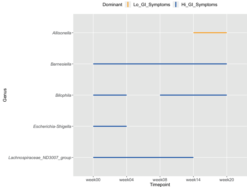
Figure 5: Time intervals of significantly different bacterial genera between GI symptoms groups. Each line interval represents a significant time interval, with significance being considered p<.05 . Orange lines indicate higher abundance in the “lo” GI symptoms group, while blue indicates higher abundance in the “hi” GI symptoms group.
