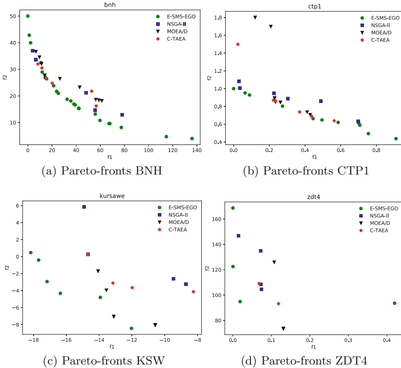
Fig. 1. Pareto frontiers obtained by the four algorithms on four of the test functions.
