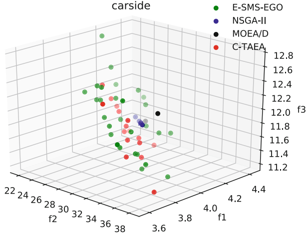
Fig. 2. Pareto frontiers obtained by the four algorithms on the three-objective CSI problem.
