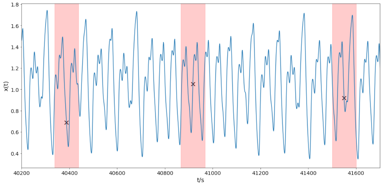
Figure 2.10: This graph shows the same section of a Mackey-Glass time series as Fig. 2.7, but now reveals the location of the anomalies in the time series. The anomalies are at t_1 = 40388 , t_2 = 40917 and t_3 = 41550 . The positions are indicated by the black crosses in the plot.
