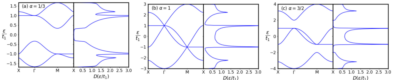
FIG. 3. The spectrum of T-graphene along the closed path X - \Gamma - M - X and DOS for \alpha = 1/3, 1 and \alpha = 3/2 . DOS is plotted on the right of each spectrum and is measured in units of \frac{1}{a^2 t_1} . DOS is regularized with finite broadening of levels, \Gamma = 0.01t_1 to make plots smooth.
