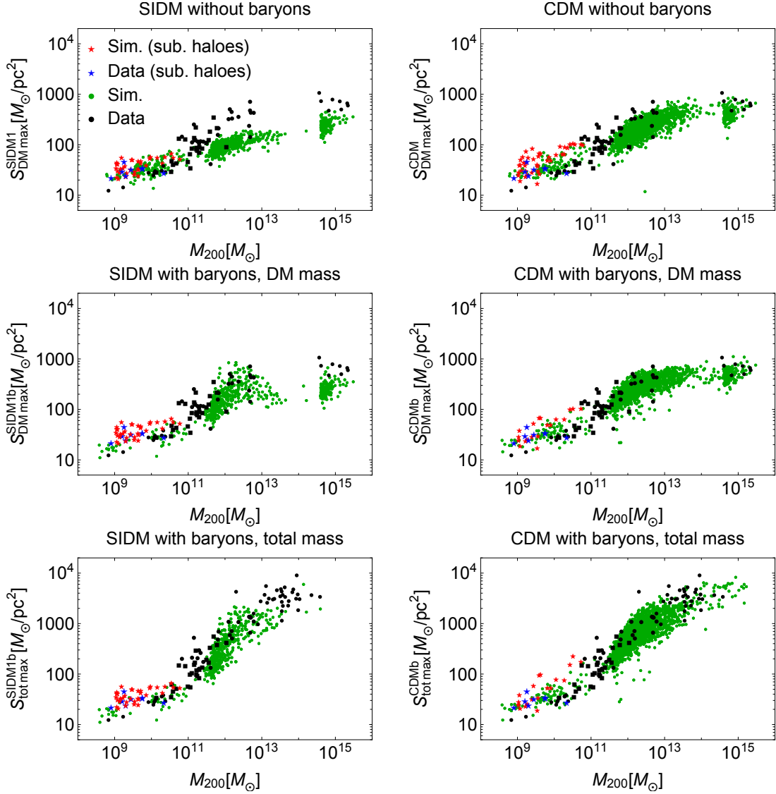
Figure 20. The maximal surface density of DM mass or total mass versus M_{200} for observed isolated haloes (black points), observed subhaloes (blue stars) and simulated isolated haloes (green points) and subhaloes (red stars). Three left panels represent SIDM, three right panels represent CDM. Top two panel are for dark matter only simulations, two middle are for DM surface density in the simulations with baryons, two lower panels are for the total mass surface density. Observed objects include galaxy clusters, elliptical galaxies, spiral galaxies, isolated dwarf galaxies and classical dwarf satellites of the Milky Way. Observed objects where the real local peak in S(r) was detected are represented by black squares rather than black circles (see section 4 for details). Simulation data is described in table 1. For the BAHAMAS simulations we choose only massive haloes, M_{200} > 4 \times 10^{14} M_{\odot} that correspond to the masses of the observed halos that we use. For SIDM1b we do not have simulated subhaloes and use SIDM1 DMO subhaloes.
