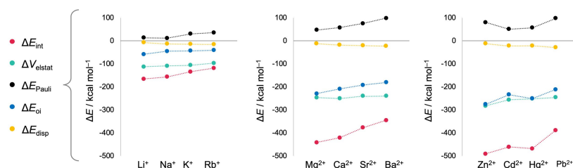
Figure 6. Energy decomposition analysis of the interaction energy ( \Delta E_{\text{int}} , in \text{kcal mol}^{-1} ) between the metal cations \text{M}^{n+} and the GQ scaffold in \text{GQ-M}^{n+} , calculated at ZORA-BLYP-D3(BJ)/TZ2P. The energies for \text{GQ-M}^{1+} are taken from Ref. [8]. The dotted lines between the data points are there to guide the reader.
