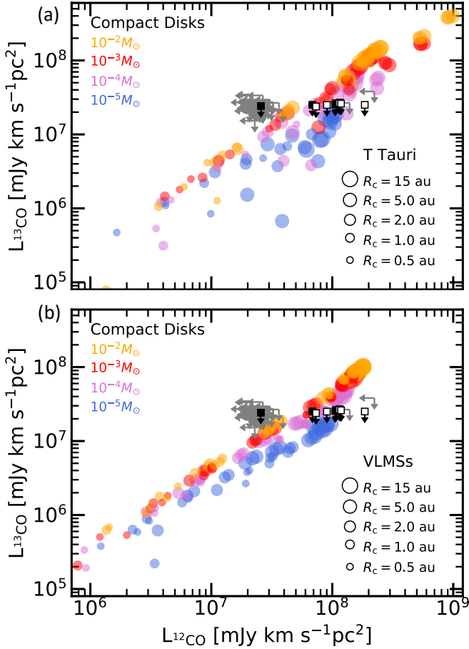
Fig. 2. Lupus ^{12}\text{CO} and ^{13}\text{CO} ( J = 2 - 1 ) line luminosity are presented with black squares (empty squares if the ^{12}\text{CO} line is partially absorbed by the cloud), where the ^{13}\text{CO} non detections are shown as upper limits by the black arrows and the ^{12}\text{CO} (and ^{13}\text{CO} ) non detections are shown as upper limits by the gray arrows. DALI model results for T Tauri disk models are shown in panel (a), and those for VLMS disk models in panel (b) with filled circles, color-coded by disk mass. Different symbol sizes represent different values of the critical radius R_c . Notice the different scale from Fig. 1.
