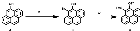
Scheme 2.6 Synthesis of propellerene 1 from 4-hydroxypyrene 4 . Reagents and conditions: a) \text{Br}_2 , \text{CS}_2 , -10^\circ\text{C} , 94%; b) i) HMDS, PhMe, reflux, 3 hrs; ii) n -BuLi, THF, -78^\circ\text{C} ; iii) \text{Tf}_2\text{O} , -78^\circ\text{C} , 47% over three steps.
