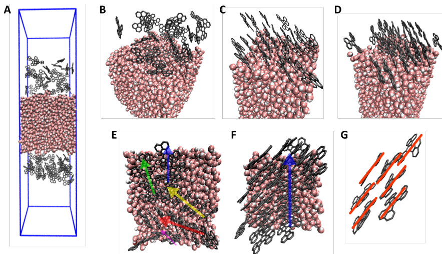
Figure 5.2 Molecular Dynamics (MD) simulation on decacycene thin films. (A), MD simulation box ( 5.0 \times 5.0 \times 20.0 \text{ nm}^3 ) containing water molecules represented by a space filling model, and the random, pre-equilibration position of decacycene molecules (30) on both sides thereof represented by a liquorice model in grey. Protons explicitly drawn on water but omitted from decacycene. (B) Top view of A. (C) Same system as B, after equilibration at 300 K. (D) Same system as C, after compression to a surface pressure of 30 \text{ mN m}^{-1} . (E) Top view of D after equilibration at 300 K. Differently colored arrows added to highlight different stacking domains. (F) Same system as in E after compression to a surface pressure of 30 \text{ mN m}^{-1} . (G) Highlight of molecules found in F showing the onset of roof-tiling.
