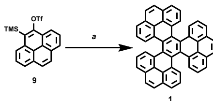
Scheme 2.9 Synthesis of tripyrenylene 1 . Reagents and conditions: a) CsF, \text{Pd}_2(\text{dba})_3 , MeCN:Et 2 O, rt, o/n, 47%.
