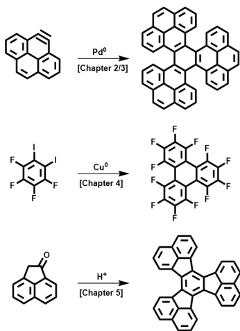
Figure 6.2 Schematic illustration of different ways in which trimeric PAHs can be obtained, as used in different Chapters in this Thesis. From top to bottom: tripyrenylene 1 (Ch. 2/3), perfluorotriphenylene (Ch. 4), and decacyclene (Ch. 5).
