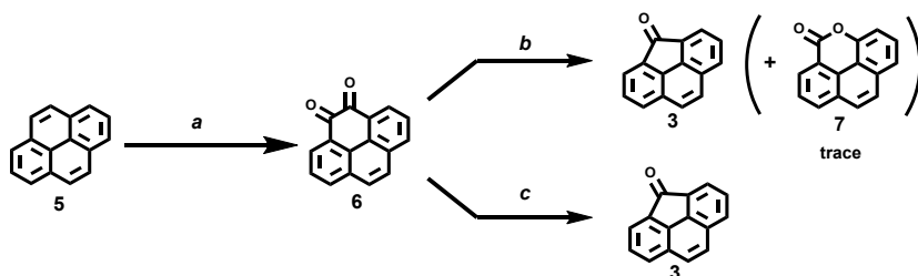
Scheme 2.3 Synthesis of oxoCPP. Reagents and conditions: a) \text{NaIO}_4 , \text{RuCl}_3 , DCM:MeCN:H 2 O, rt, 3 hrs (50%); b) \text{PbO} , 245 – 260 °C, vac., 3 hrs., 4 – 8%; c) 1M NaOH, reflux, 3 d., 30%.
