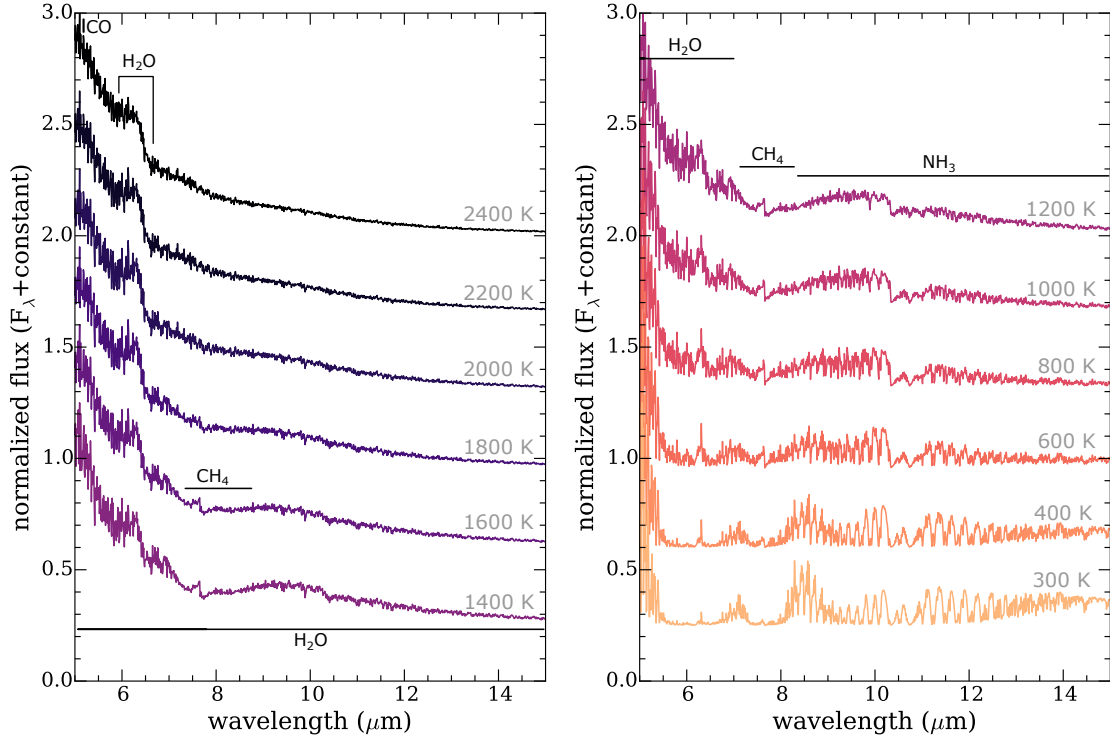
Figure 7. Same as Figure 3 but for mid-IR spectral range with R \sim 1,000 . Note how the arrival of \text{NH}_3 dramatically transforms this region below about 1200 K in these equilibrium chemistry models.
