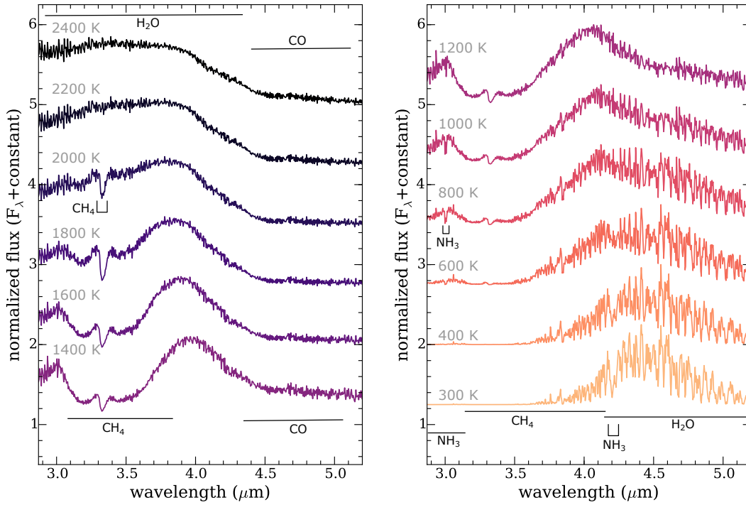
Figure 6. Same as Figure 3 but for 3 to 5 \mu\text{m} spectral region and R \sim 1,000 . Note how the peak in emission shifts from \sim 4 to \sim 4.5 \mu\text{m} through this sequence.
