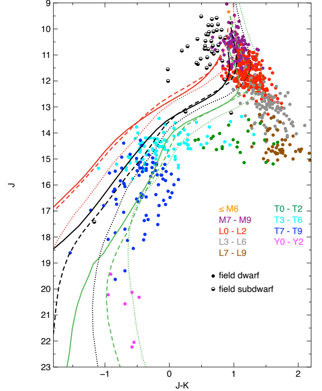
Figure 14. Cloudless Sonora Bobcat cloudless colors for different constant values of gravity and metallicity as compared to Mauna Kea Observatory J - and K -band photometry of nearby M, L, T, and Y dwarfs from (Best et al. 2020). The curves are coded by their line types (solid, dashed, dotted) for \log g(\text{cm s}^{-2}) = 5, 4 , and 3 respectively and line colors, from top to bottom groups [\text{M}/\text{H}] = -0.5, 0.0 , and +0.5 for red, black, and green. The near-infrared spectral types are denoted by the color of the dot. Half-filled circles are subdwarfs.
