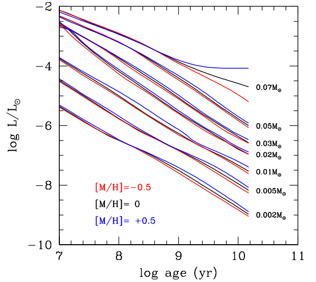
Figure 12. Comparison of brown dwarfs luminosity cooling tracks for three different metallicities. Each triplet of tracks is labeled with the mass in solar masses. For a given mass and age, a higher metallicity results in a slightly higher luminosity. The 0.07 M_{\odot} models are just below the hydrogen burning minimum mass and their fates diverge after 2 Gyr, depending on the metallicity. The [M/H]=+0.5 track approaches a stable equilibrium on the main sequence while the lower metallicity tracks for that mass fail to do so.
