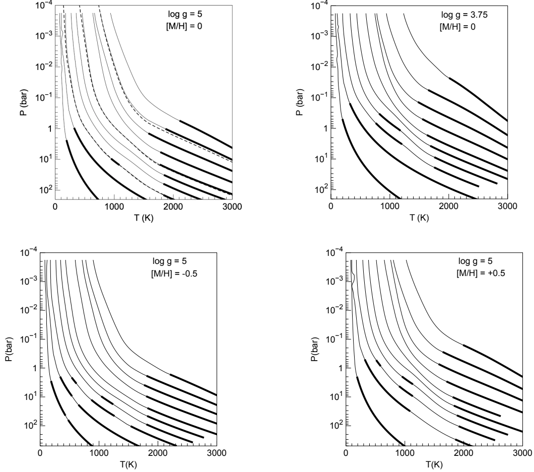
Figure 1. Converged radiative-convective equilibrium temperature profiles computed by our modeling approach for various parameters as noted in each panel. In all panels models are shown every 200 K from T_{\text{eff}} = 200 to 1200 K and then every 300 K to 2400 K. Thick lines show convective regions of the atmospheres. Note how at higher effective temperatures the boundary lies near 2000 K, then with falling T_{\text{eff}} , convection turns on in some portions of the radiative region, until finally these isolated zones merge and the boundary moves up to near 1 bar in the coolest models. Dashed curves show cloudless, chemical equilibrium profiles from Phillips et al. (2020) for \log g = 5 and T_{\text{eff}} 600, 1200, and 2100 K.
