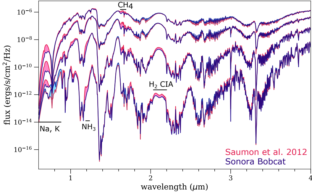
Figure 9. Comparison of the present Sonora Bobcat model spectra ( R \sim 1,000 ) with those of Saumon et al. (2012) at T_{\text{eff}} = 1300, 900, 500 , and 300 K (top to bottom). Absorbers responsible for notable differences are labeled.
