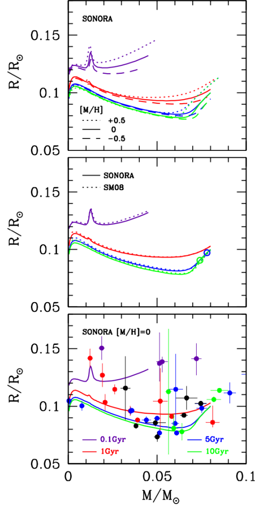
Figure 16. Mass-radius relation of evolution models of ultracool dwarfs. Each panel shows isochrones of the M - R relation: 0.1 Gyr (purple), 1 Gyr (red), 5 Gyr (blue) and 10 Gyr (green). Each isochrone is truncated at T_{\text{eff}} = 2400 K, the limit of our atmosphere model grid. Top panel: Dependence of the radius on the metallicity. Metal-rich objects have systematically larger radii because they cool more slowly. The sharp peak in the 100 Myr isochrone is caused by deuterium burning. Middle panel: Comparison with the cloudless, solar metallicity models of Saumon & Marley (2008) (SM08). Large open circles indicate the location of the hydrogen burning minimum mass for each isochrone. Bottom panel: Comparison of solar metallicity models with data. Data points are colored according to their age in bins corresponding to the model isochrones: 0.03 - 0.3 Gyr (purple), 0.3 - 2.2 Gyr (red), 2.2 - 7 Gyr (blue), > 7 Gyr (green), unknown (black). Data from Šubjak et al. (2020) ; David et al. (2019) ; Gillen et al. (2017) ; Carmichael et al. (2020) ; Benni et al. (2020) ; Zhou et al. (2019) ; Carmichael et al. (2019) ; von Boetticher et al. (2017) ; Hodžić et al. (2018) ; Nowak et al. (2017) ; Winn et al. (2007) ; Mireles et al. (2020) ; Cañas et al. (2018) ; Acton et al. (2020) ; Littlefair et al. (2014) ; Parsons et al. (2017) ; Casewell et al. (2020) , T.G. Beatty, pers. comm., S. L. Casewell, pers. comm.
