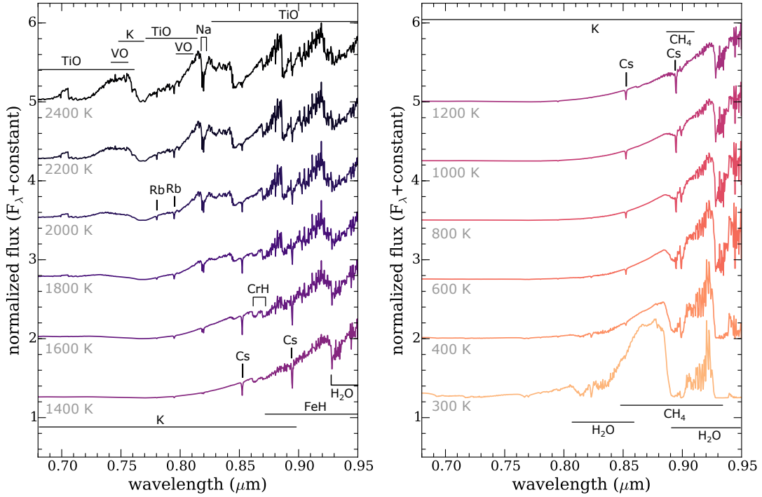
Figure 3. Red optical spectral sequence ( R \sim 2,000 ) of models for solar metallicity and C/O ratio at \log g = 5 , shifted vertically for clarity. Notable absorption features are labeled. Models are shifted for clarity.
