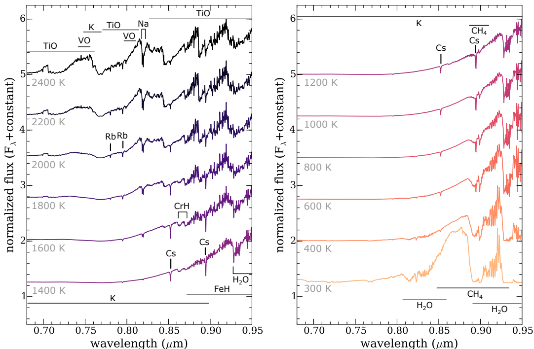
Figure 3. Red optical spectral sequence ( R \sim 2,000 ) of models for solar metallicity and C/O ratio at \log g = 5 , shifted vertically for clarity. Notable absorption features are labeled. Models are shifted for clarity.
