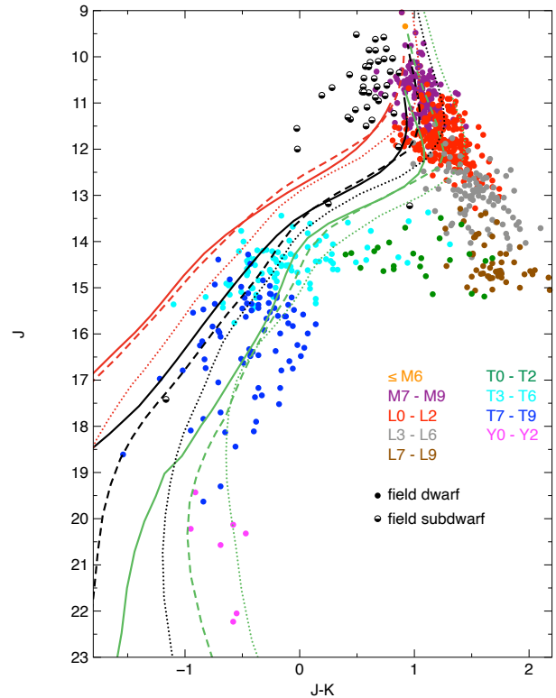
Figure 14. Cloudless Sonora Bobcat cloudless colors for different constant values of gravity and metallicity as compared to Mauna Kea Observatory J - and K -band photometry of nearby M, L, T, and Y dwarfs from (Best et al. 2020). The curves are coded by their line types (solid, dashed, dotted) for \log g(\text{cm s}^{-2}) = 5, 4, and 3 respectively and line colors, from top to bottom groups [\text{M}/\text{H}] = -0.5, 0.0, and +0.5 for red, black, and green. The near-infrared spectral types are denoted by the color of the dot. Half-filled circles are subdwarfs.
