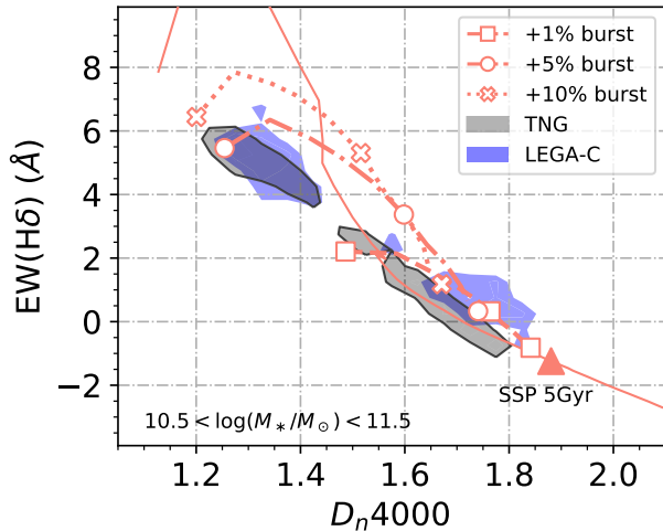
Figure 8. Model tracks with additional bursts on top of an old population (see text). Lines show the evolution from 0.1 Gyr to 1 Gyr after the burst happened. Markers label 0.1, 0.5, and 1.0 Gyr after the burst for the 1%, 5%, and 10% burst models. The solid line is the SSP, equivalent to a 100% burst event. Whereas the old galaxies in the TNG100 sample (gray) are overall consistent with the SSP model, the LEGA-C galaxies (blue) are more consistent with models with an additional burst that adds a few percent of stellar masses in the last \sim 1 Gyr. For clarity, only contours of 0.5 times of the peak densities of the simulation and observational galaxy samples are shown – see Fig. 5 for the full distributions.
