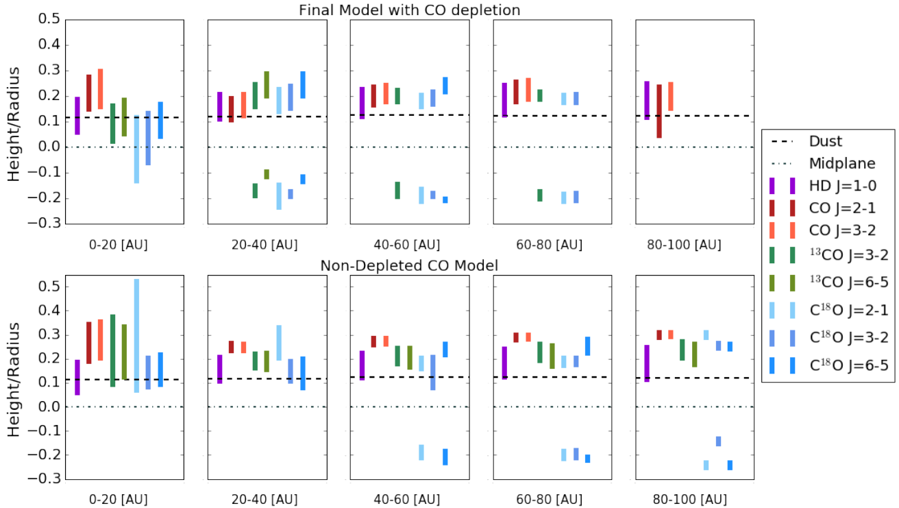
Figure 9. The average vertical emitting region of each line used in this study for our final model (top) and a version of that model without assuming CO depletion (bottom). For every 20 AU the average vertical emitting height was calculated. The top of each bar corresponds to the average surface which consists of 90% of the flux. The bottom of the bar and below is 10% of the total flux. Lines that have two emitting regions, one above the disk and below, are optically thin, thus observations of these molecules come from both the front and back of the disk. There is no emission in the midplane outside the CO snowline, thus for an optically thin emitter, their emitting regions were calculated twice. Once for above the midplane, then again but only from the back. The continuous \tau = 1 surface of the dust at the frequency of HD J=1-0 is shown via the dashed line. Examples of 2D contribution plots used to create this figure of 12 CO 2-1 and C 18 O 2-1 are shown in Figure 8.
