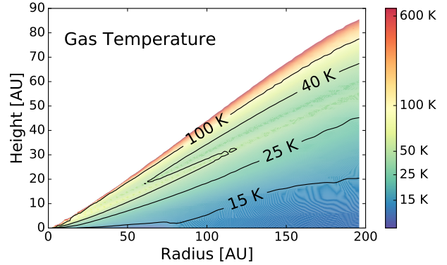
Figure 6. The final 2D thermal structure of the gas that reproduces seven resolved ALMA CO lines, HD flux, and the SED. The final temperature profile is supported up to scale heights from which ^{12}\text{CO} 2-1 emits from, since this transition has the highest optical depth
