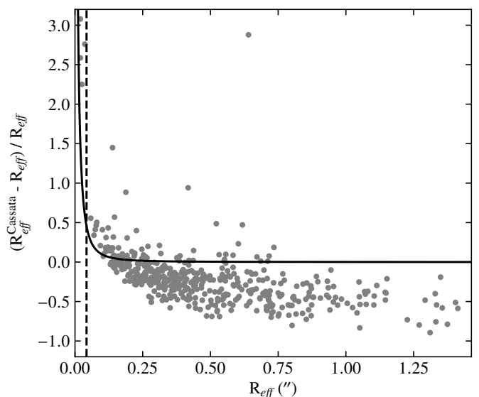
Fig. 2: Relative difference between the global effective radius inferred from our GALFIT models and the Cassata et al. (2007) morphological catalog as a function of the GALFIT effective radius. The black solid line represents the limiting effective radius measurable when not taking into account the PSF and the dashed vertical line marks the value of half the HST-ACS PSF FWHM.
