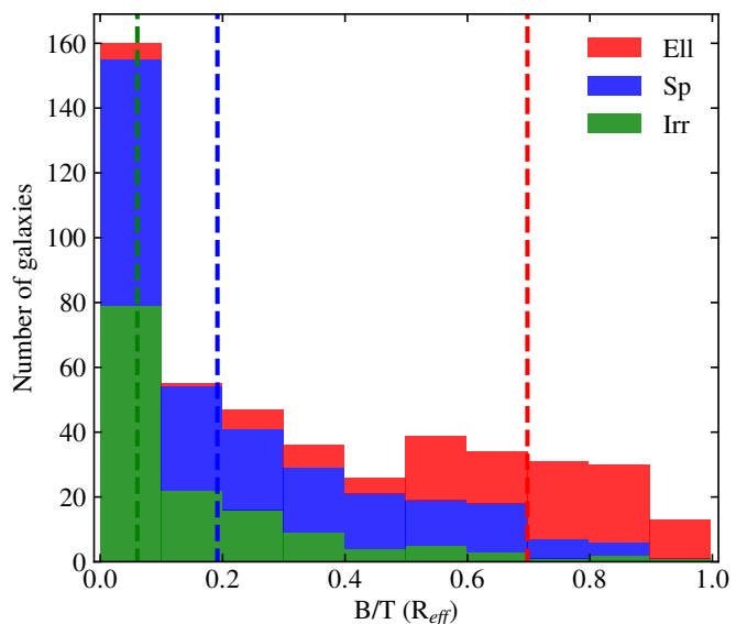
Fig. 3: Distribution of the three morphological classes defined in the Cassata et al. (2007) catalog as a function of the bulge to total flux ratio estimated at the effective radius. Green, blue and red stacked histograms correspond to galaxies classified respectively as irregular, spiral and elliptical. The median values for those three classes are 0.06, 0.19 and 0.70 respectively and are indicated by dashed colored vertical lines.
