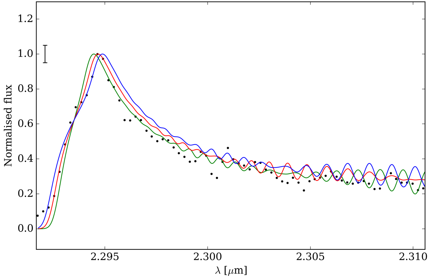
Fig. A.9. Continuum-subtracted first CO bandhead of 51 Oph normalised to the peak intensity (black dots). Coloured lines shown models with fixed values of T=2400 K, N_{\text{CO}}=4 \times 10^{21} \text{ cm}^{-2} , \Delta v=15 \text{ km s}^{-1} and v_{\text{rot}} \sin i values of 100 \text{ km s}^{-1} (solid green line), 130 \text{ km s}^{-1} (solid red line), and 160 \text{ km s}^{-1} (solid blue line). The black vertical line in the top left corner of the peak of the bandhead has a length of twice the rms value measured at the continuum.
