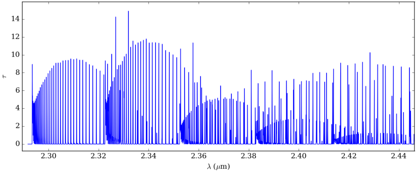
Fig. A.1. Optical depth vs. wavelength for the first five CO bandheads ( v=2-0 , 3-1 , 4-2 , 5-3 , and 6-4 ,) at R=100\,000 . The CO is modelled as a ring at T=2400 K, N_{\text{CO}}=4\times 10^{21} \text{cm}^{-2} , and v_{\text{rot}} \sin i=130 \text{km s}^{-1} . The intrinsic CO line width is \Delta v=15 \text{km s}^{-1} .
