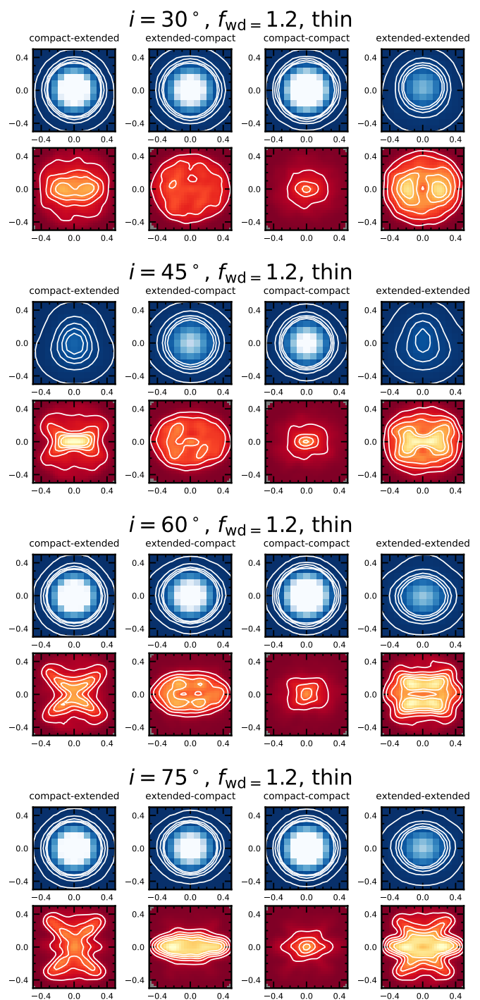
Fig. 14. Simulated CAT3D-WIND images matching for the GATOS Seyferts. Parameters are the same as in Fig. 13 but for a wind-to-disk ratio of f_{\text{wd}} = 1.2 . The image brightness scales and contour levels are as in Fig. 11.
