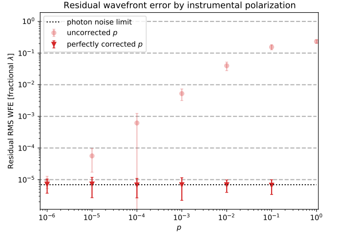
Fig. 9. Performance of the wavefront sensing with instrumental polarization effects. The error bars show the 1\sigma deviation over the 100 random wavefront aberration instances. The circles show that data points where the strength of instrumental polarization ( p ) was not corrected and the triangles show the data points where p was corrected. The dotted lines shows the photon noise limit, which was introduced to prevent the residual wavefront error reaching numerical noise.
