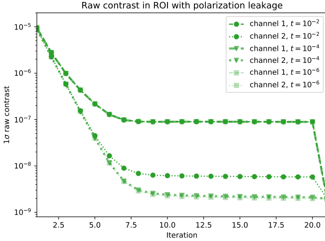
Fig. 17. Raw contrast as function of iterations for the system with polarizer leakage. The response matrix is acquired with the polarizer leakage. At iteration 21, RH is blocked to compare the raw contrast between the two channels.
