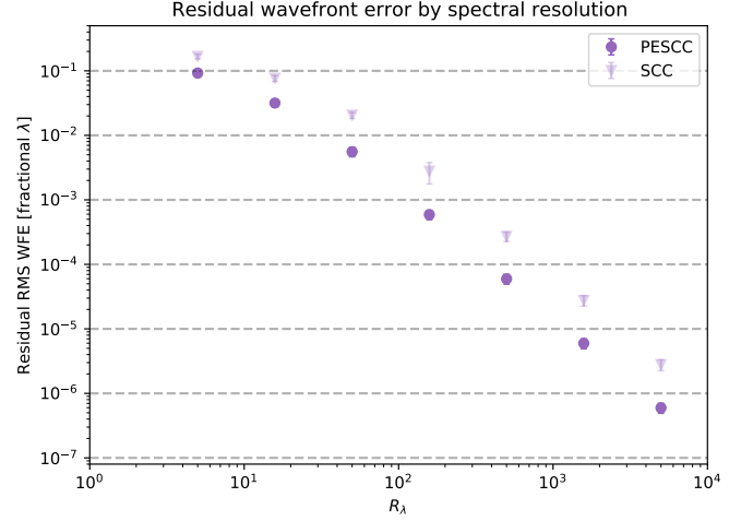
Fig. 11. Performance of the wavefront sensing with varying spectral resolution ( R_\lambda ). The error bars show the 1\sigma deviation over the 100 random wavefront aberration instances. The circles show the performance of the PESCC and the triangles the performance of the SCC.
