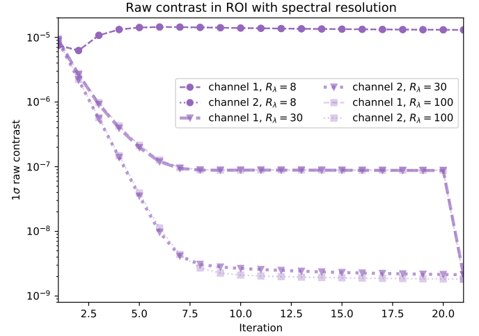
Fig. 18. Raw contrast as function of iterations for the system with broadband effects. The response matrix is acquired with the broadband effects included. At iteration 21, the RH is blocked to compare the raw contrast in the two channels.
