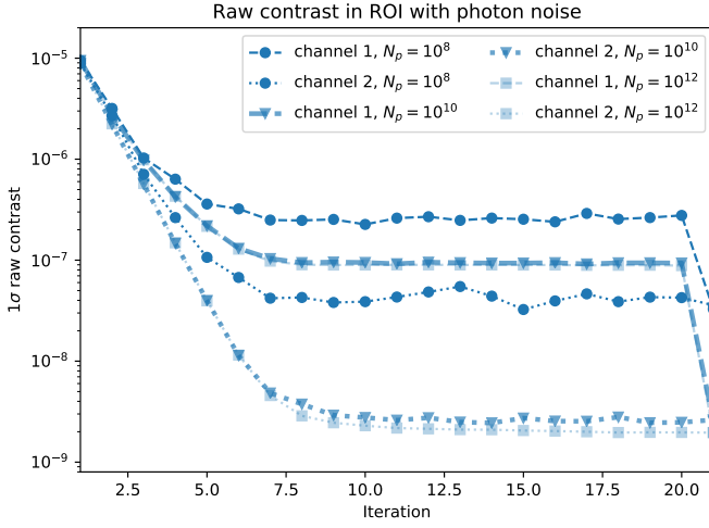
Fig. 14. Raw contrast as function of iterations for the system with photon noise. The response matrix is acquired without photon noise. At iteration 21, the RH is blocked to compare the raw contrasts in the two channels.
