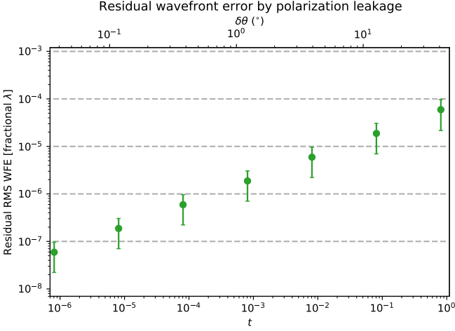
Fig. 10. Performance of the wavefront sensing with polarization leakage. The error bars show the 1\sigma deviation over the 100 random wavefront aberration instances. The bottom x-axis shows polarization leakage ( t ), and the upper x-axis shows the equivalent rotation offset ( \delta\theta ) between the RH polarizer and PBS. We note that the right most data point is sampled at t = 0.81 .
