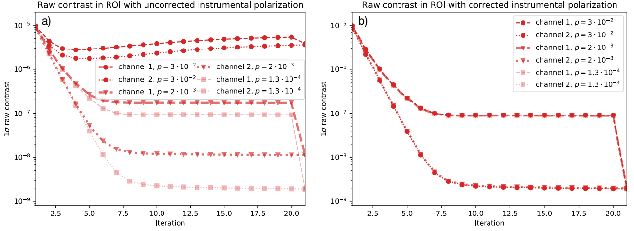
Fig. 16. Raw contrast as function of iterations for the perfect system with instrumental polarization ( p ) effects. At the last iteration, the RH is blocked to compare the raw contrast in the two channels. (a) During the acquisition of the response matrix and the closed loop tests the effects of p were not corrected. (b) During all steps of the response matrix acquisition and WFC tests, p was corrected. All three tested levels of p now overlap and reach the performance level of the benchmark tests.
