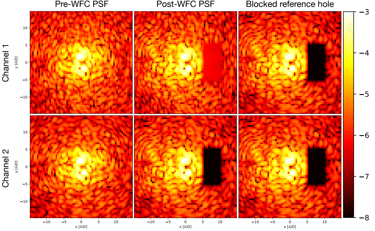
Fig. 12. WFC example with the PESCC without noise sources present. The subfigures in the two rows show the PSFs of the two channels. The columns show, respectively, the PSFs before WFC, the PSFs after twenty iterations of the WFC, and the PSFs after the WFC with the RH blocked. The colorbar shows the intensity in logarithmic scale and is equal for all subfigures.
