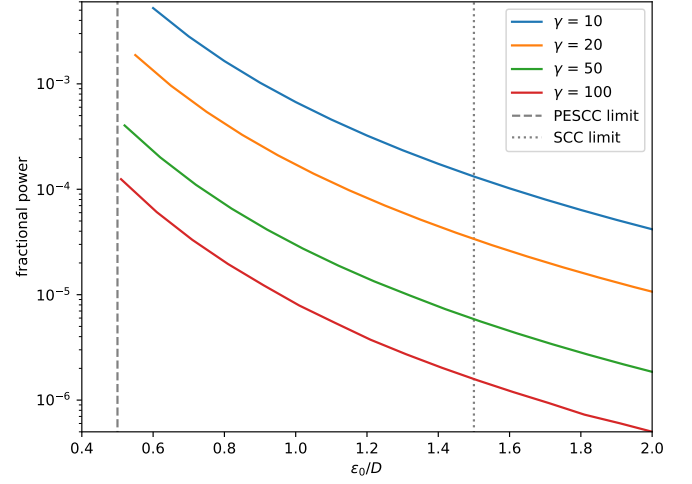
Fig. 6. Fractional power in the RH (ratio of the power in the RH and total power in pupil plane before Lyot stop) as function of distance from the center of the pupil. This was simulated using a charge two vortex coronagraph and does not include the polarizer in the RH for the PESCC to show the total power available.
