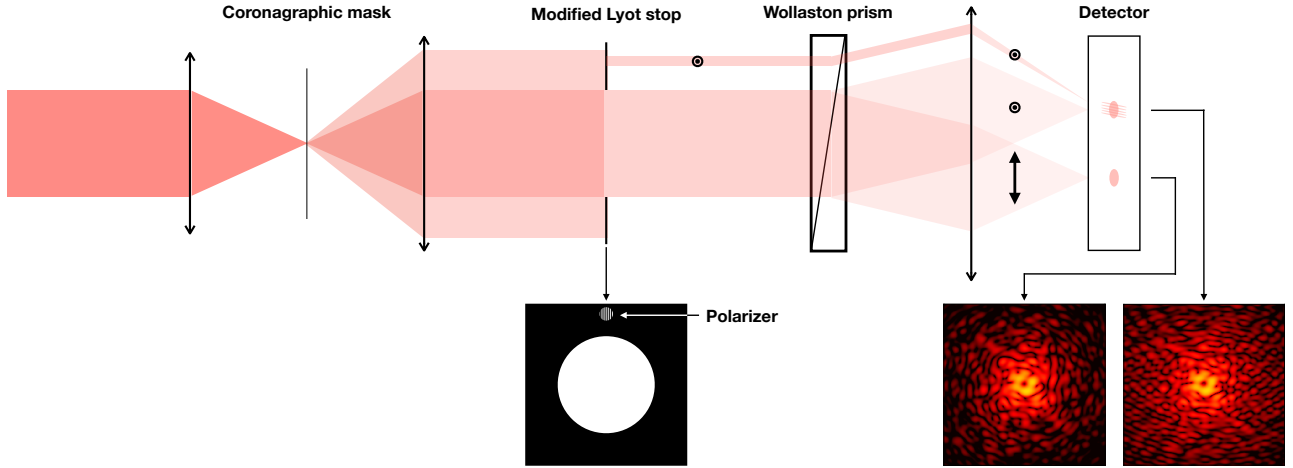
Fig. 1. Overview of the system architecture of the PESCC. A focal-plane coronagraph (in this example a charge two vortex mask) diffracts the starlight out of the geometric pupil. A reference hole (RH) with polarizer is placed in the Lyot stop and lets a polarized reference beam through. The polarization state of the reference beam is pointing away from the page. Prior to the focal-plane, a Wollaston prism (or any other polarizing beamsplitter) splits the two orthogonal polarization states. The image with a polarization state that matches the RH polarizer has fringes that encode the wavefront information, while the orthogonal polarization state remains unmodulated by fringes.
