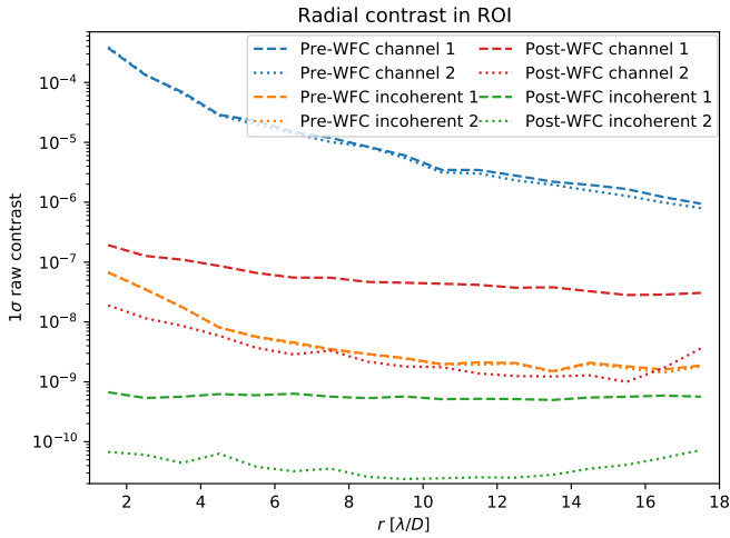
Fig. 21. Radial contrast in the ROI for the CDI simulation. Shown are the 1\sigma raw contrast curves before and after WFC and CDI.
