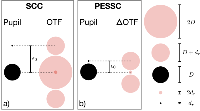
Fig. 3. Explanation of how the geometry of the pupil relates to the geometry of the OTF. This figure shows that the minimum distance of the RH of (a) the SCC is much larger than that of (b) the PESSC.
