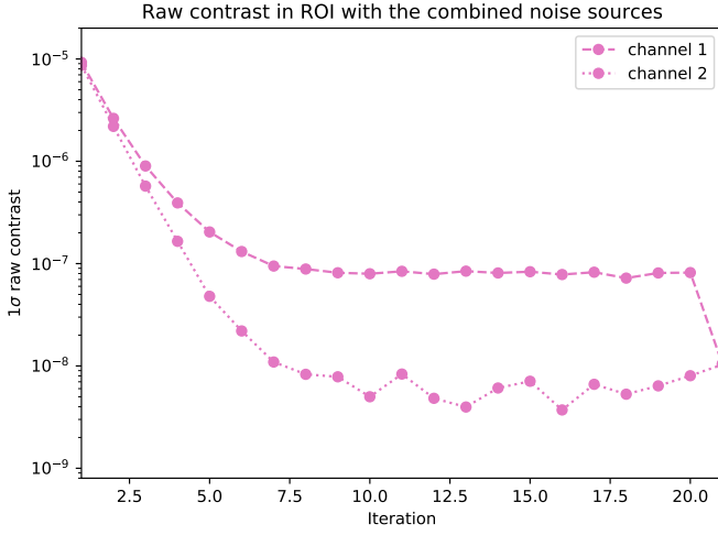
Fig. 19. Raw contrast as function of iterations for the system with all effects. The response matrix is acquired with all effects included. At iteration 21, the RH is blocked to compare the raw contrasts in the two channels.
