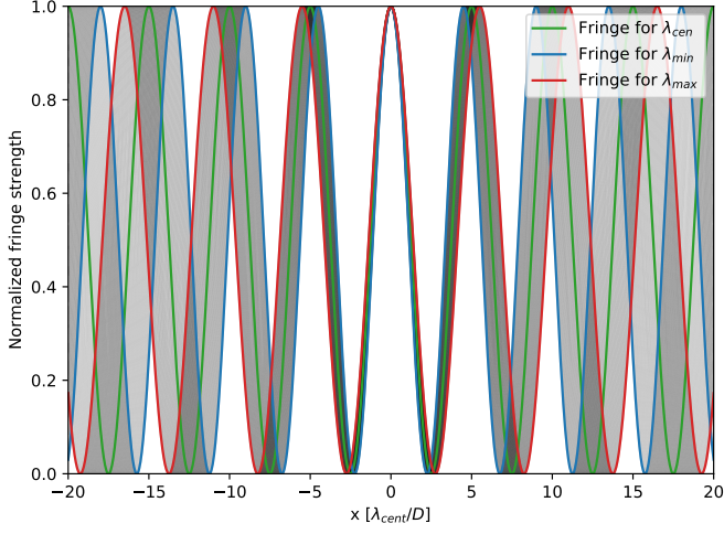
Fig. 4. Example of fringe smearing by spectral bandwidth. Fringes are plotted for many wavelengths within a broadband filter ( R_\lambda = 5 ). All are plotted with a period of 5 \lambda/D , but due to the changing wavelength the physical fringe periods in the focal plane change as well. This results in significant fringe blurring after only a few periods from the center.
