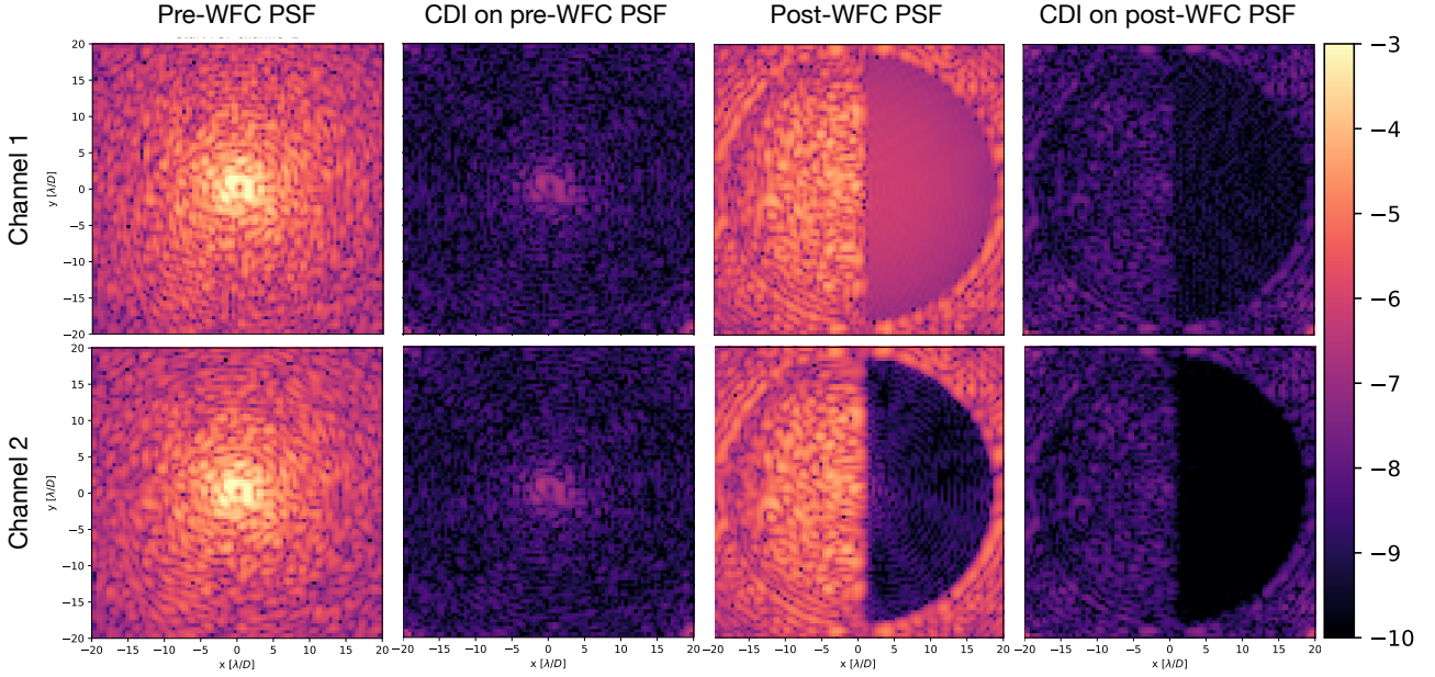
Fig. 20. WFC and CDI example with the PESCC for a system without noise source other than wavefront aberrations. The two rows show subfigures of the two channels. The columns show the PSFs before WFC, the PSFs before WFC and after CDI, the PSFs after WFC, and the PSFs after WFC and CDI. The colorbar shows the intensity in logarithmic scale and is equal for all subfigures.
