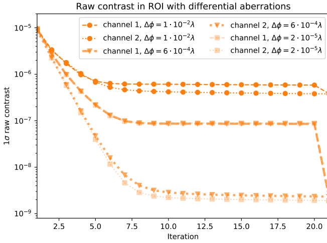
Fig. 15. Raw contrast as function of iterations for the system with different levels of RMS differential aberrations ( \Delta\phi ) between the beams. The response matrix is acquired with the differential aberrations present. At iteration the RH is blocked to compare the raw contrast in the two channels.
