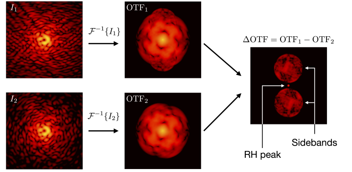
Fig. 2. Example of sideband extraction with the PESCC. For the images of channels 1 and 2 ( I_1 and I_2 ) in Figure 1, the OTFs are calculated. The OTF_1 contains the two sidebands with wavefront information and the RH peak, but these are overwhelmed by the central peak. When OTF_2 , which only contains the central peak, is subtracted from OTF_1 , the two sidebands and RH peak are revealed.
