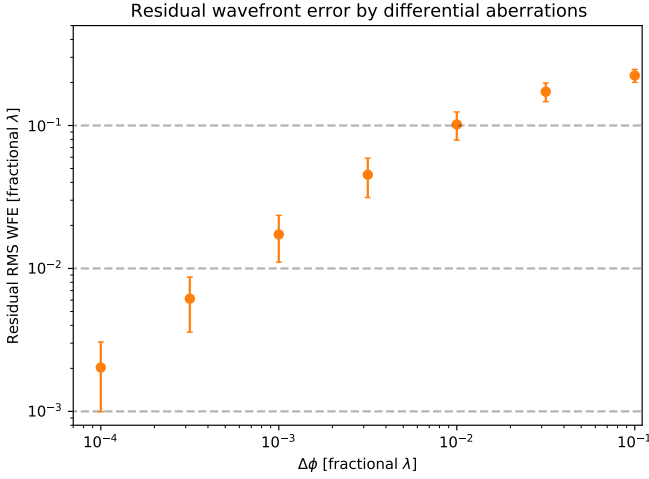
Fig. 8. RMS differential aberrations ( \Delta\phi ) between the two beams downstream of the polarizing beamsplitter, and their effect on the wavefront reconstruction. The error bars show the 1\sigma deviation over the 100 random wavefront aberration instances.
