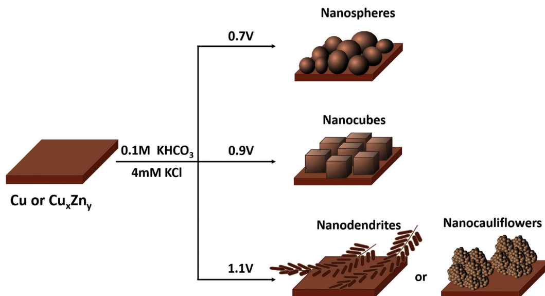
Scheme 1. Preparation of Cu, Cu 90 Zn 10 , and Cu 75 Zn 25 electrodes which expose nanospheres, nanocubes, or nanodendrites/nanocauliflowers by cycling from -1.2 V vs RHE to 0.7 V, 0.9 V, or 1.1 V vs. RHE, respectively. Electrolyte: 0.1 M KHCO 3 + 4 mM KCl.
