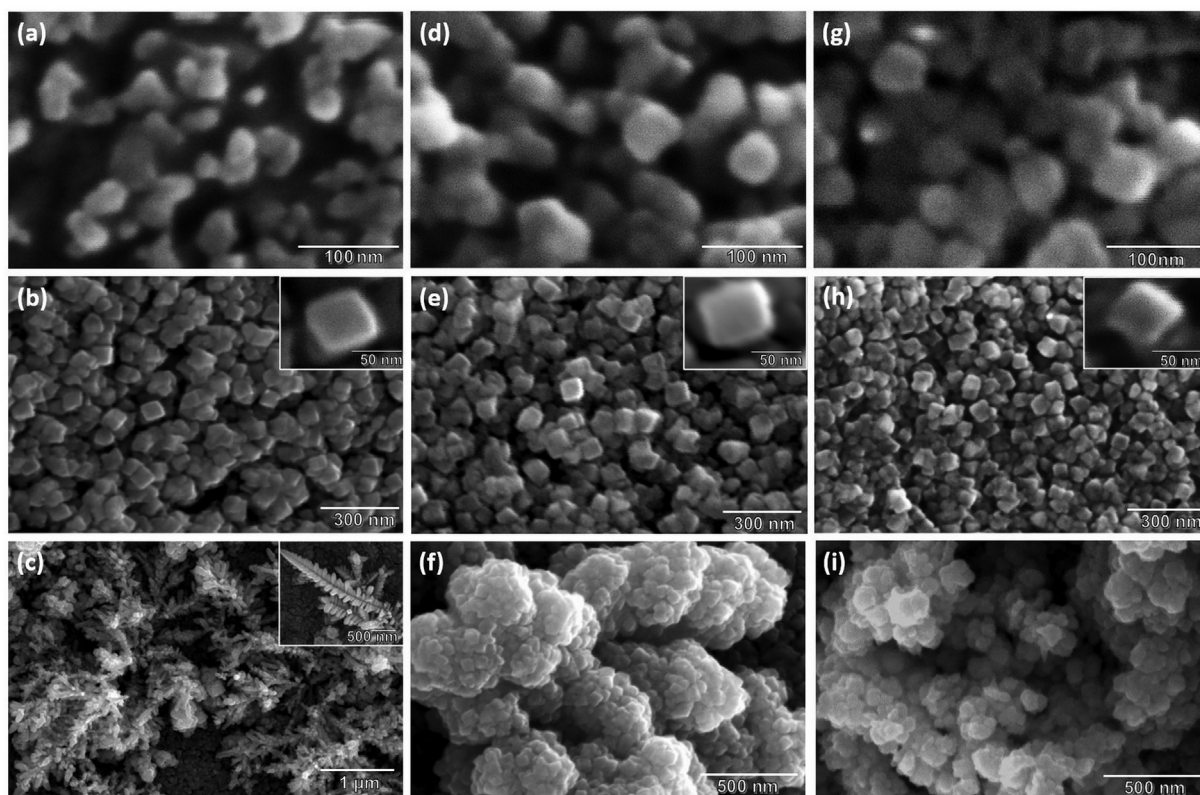
Fig. 1. SEM images of (a) OD-Cu (spheres) , (b) OD-Cu (cubes) , (c) OD-Cu (dendrites) , (d) OD-Cu 90 Zn 10(spheres) , (e) OD-Cu 90 Zn 10(cubes) , (f) OD-Cu 90 Zn 10(cauliflowers) , (g) OD-Cu 75 Zn 25(spheres) , (h) OD-Cu 75 Zn 25(cubes) , (i) OD-Cu 75 Zn 25(cauliflowers) .
