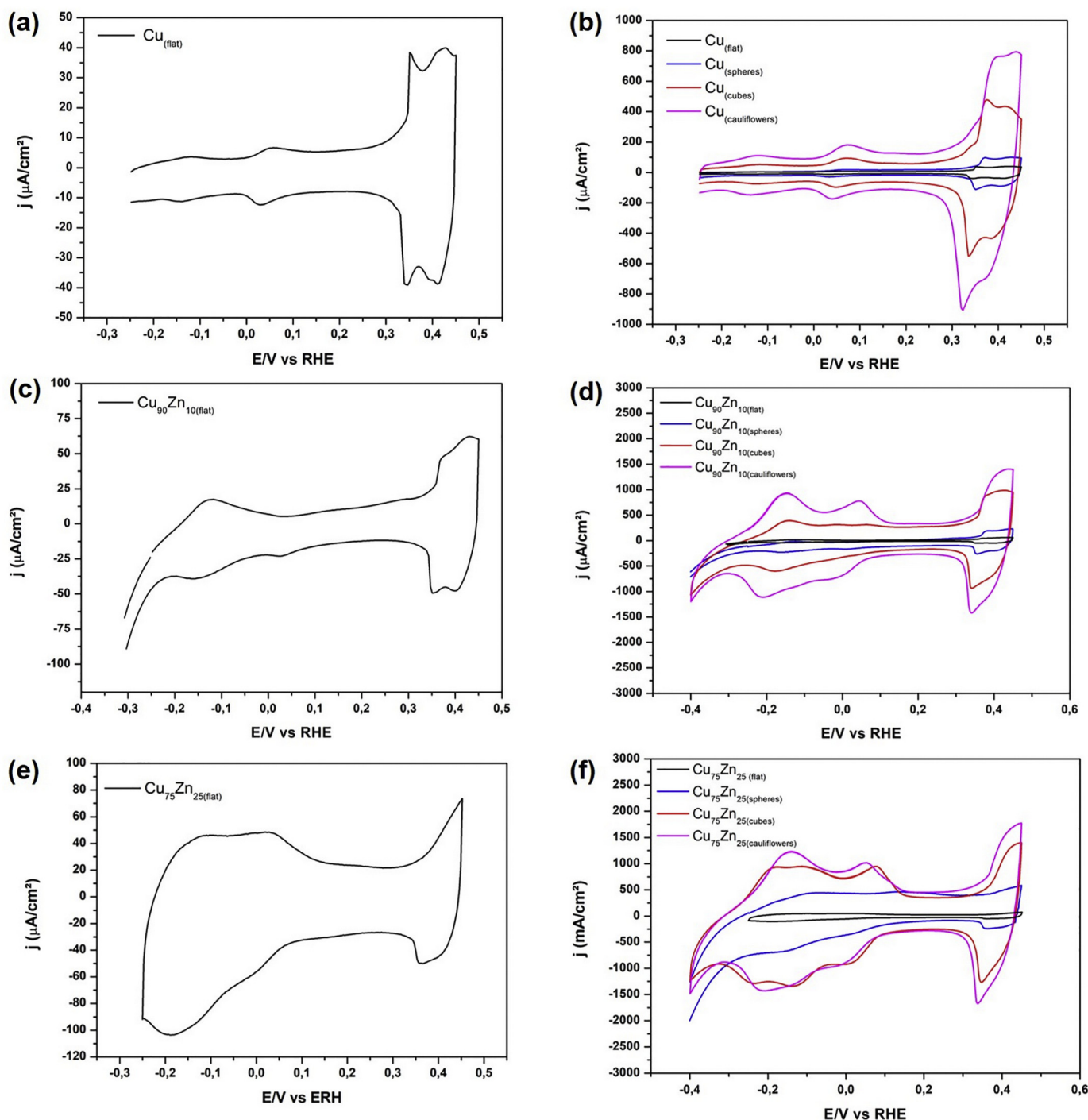
Fig. 2. Cyclic voltammograms of (a) \text{Cu}_{\text{flat}} ; (b) OD-Cu; (c) \text{Cu}_{90}\text{Zn}_{10}\text{flat} ; (d) OD- \text{Cu}_{90}\text{Zn}_{10} ; (e) \text{Cu}_{75}\text{Zn}_{25}\text{flat} ; and (f) OD- \text{Cu}_{75}\text{Zn}_{25} electrodes in 0.1 M NaOH at a scan rate of 50 \text{ mV s}^{-1} .
