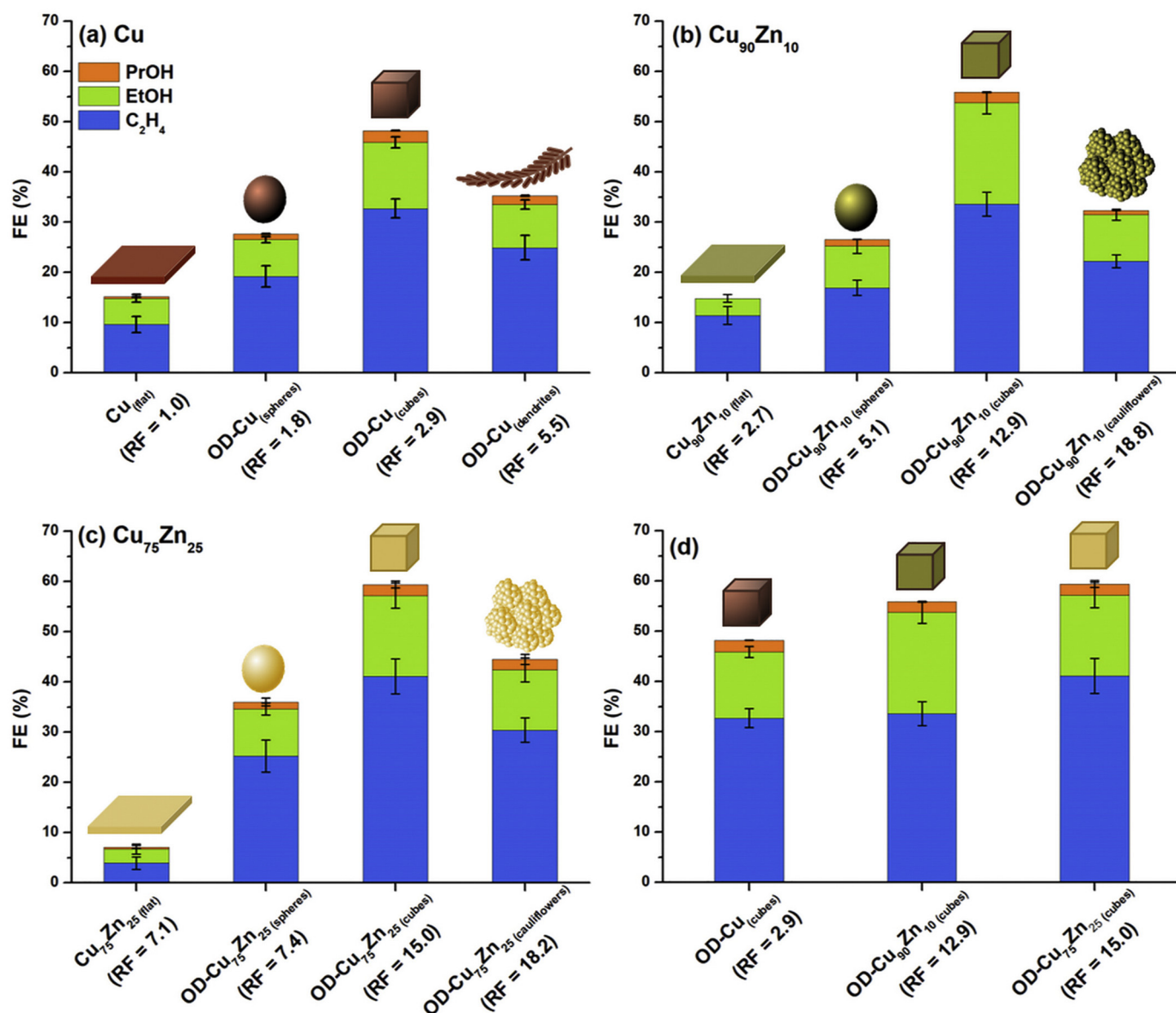
Fig. 3. Faradaic efficiency (FE) of the C_2H_4 (blue), EtOH (green), and PrOH (orange) production on (a) Cu (flat) , OD-Cu (spheres) , OD-Cu (cubes) , and OD-Cu (dendrites) , (b) Cu 90 Zn 10 (flat), OD-Cu 90 Zn 10 (spheres), OD-Cu 90 Zn 10 (cubes), and OD-Cu 90 Zn 10 (cauliflowers), (c) Cu 75 Zn 25 (flat), OD-Cu 75 Zn 25 (spheres), OD-Cu 75 Zn 25 (cubes), and OD-Cu 75 Zn 25 (cauliflowers), and (d) OD-Cu (cubes) , OD-Cu 90 Zn 10 (cubes), and OD-Cu 75 Zn 25 (cubes) at -1.1 V vs RHE. Roughness factor (RF) values were added below the name of each electrode to facilitate the discussion. (For interpretation of the references to color in this figure legend, the reader is referred to the web version of this article.)
