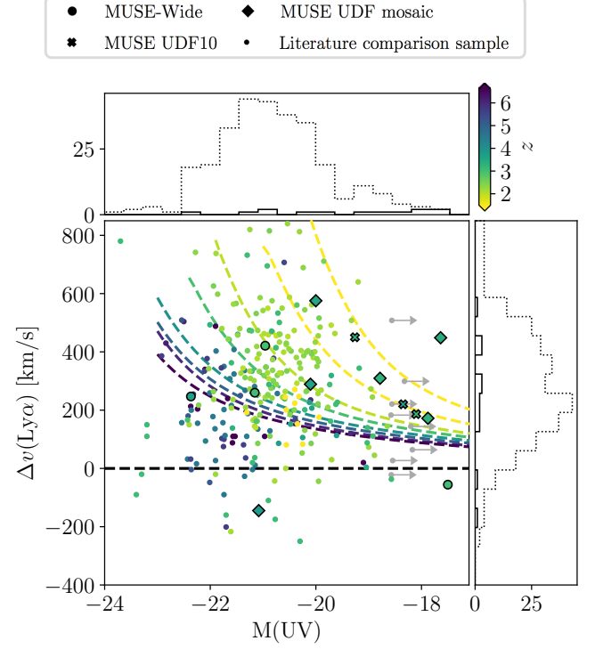
Fig. 13. Velocity offsets of \text{Ly}\alpha as a function of the absolute UV magnitude for the MUSE LAEs with \text{C III} detections studied here shown by the large symbols and a collection of measurements at redshifts from z \approx 2 to z = 7.73 collected from Kulas et al. (2012); Schenker et al. (2013); Erb et al. (2014); Stark et al. (2015a, 2017); Henry et al. (2015); Willott et al. (2015); Pentericci et al. (2016); Inoue et al. (2016); Bradač et al. (2017); Mainali et al. (2017); Verhamme et al. (2017); Sobral et al. (2018); Hutchison et al. (2019); Cassata et al. (2020); Matthee et al. (2020a), and Matthee et al. (2020b) shown by the small dots. To prevent cluttering the figure the estimated uncertainties are not shown. The median errors on the magnitudes and \Delta v_{\text{Ly}\alpha} are 0.2 mag and 50 \text{ km s}^{-1} . The dashed curves present the predicted median \Delta v_{\text{Ly}\alpha} as a function of UV magnitude for a range of redshifts (according to the color coding) from Mason et al. (2018b), corresponding to the black curve in their Figure 2 from their Equation 2). This is based on an abundance matching model relating the absolute UV magnitude to the galaxy halo mass (Mason et al. 2015). Points and curves are color-coded according to object redshift and the color gradient highlights the importance of halo mass, that is available gas reservoir, in producing and determining \Delta v_{\text{Ly}\alpha} . The solid histograms show the distribution of objects from our study, whereas the dotted histograms include the sample of measurements from the literature.
