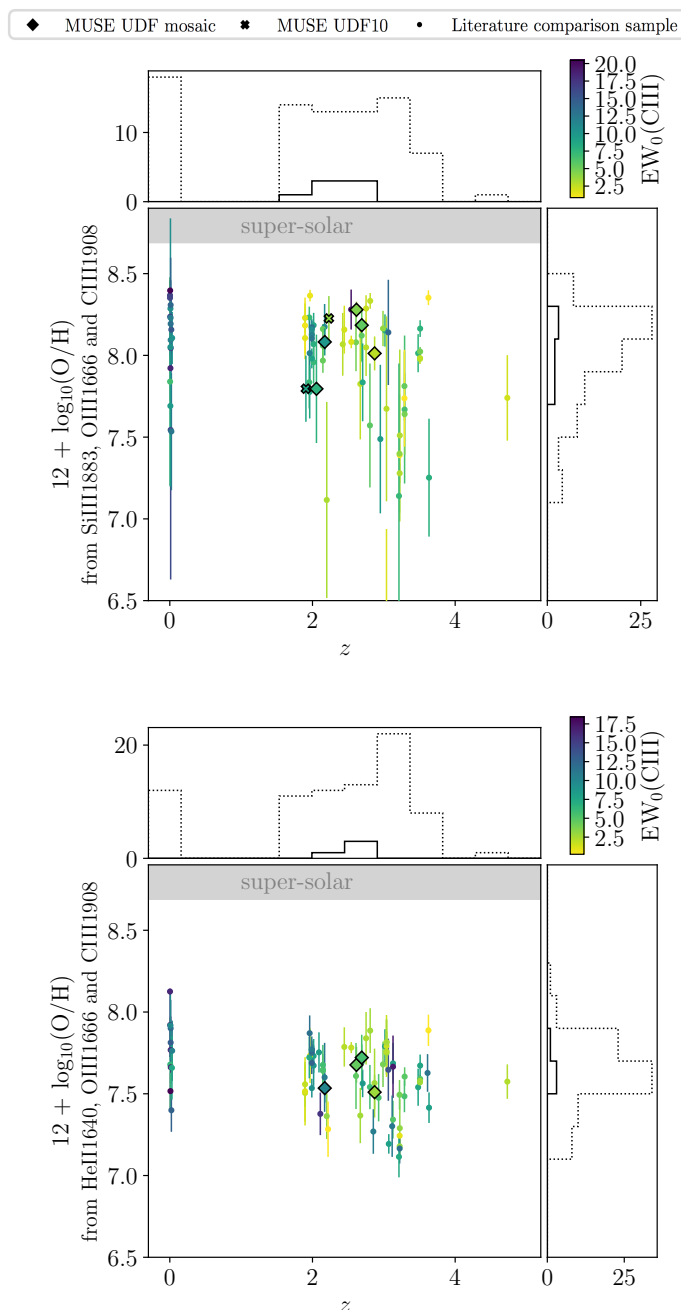
Fig. 18. Gas-phase abundances estimated using the third order polynomial fitting functions for the Si3-O3C3 (top panel) and He2-O3C3 (bottom panel) diagnostics from Byler et al. (2020) as a function of source redshift. The large symbols are MUSE sources from the UDF and small dots are from the literature collection described in Appendix C. The solid histograms show the subset of the objects from this work, whereas the dotted histograms also include the sources from the literature. All points are color coded according to \text{EW}_0(\text{CIII}) . The gray bands mark regions of super-solar gas-phase abundances at 12 + \log_{10}(\text{O}/\text{H}) > 8.69 .
