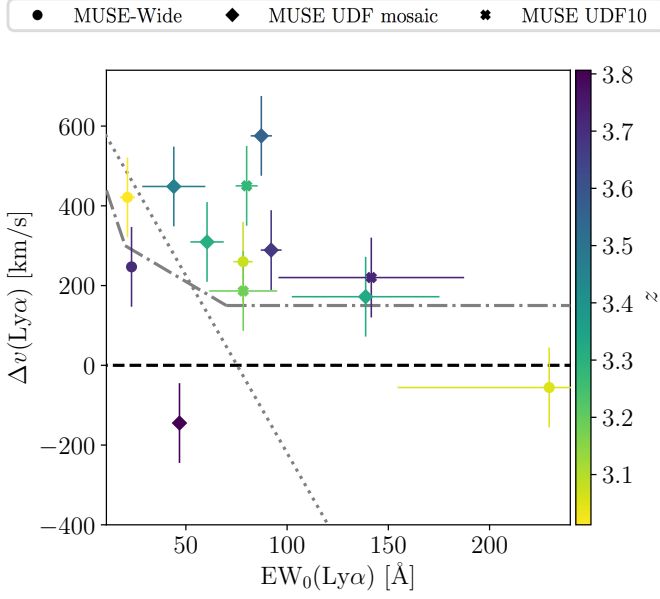
Fig. 12. Velocity offsets of \text{Ly}\alpha determined with respect to the \text{C III} detections as a function of the \text{Ly}\alpha rest-frame equivalent width estimated for a fixed UV slope of \beta = -1.97 . The gray dot-dashed and dotted lines show the empirical relationship between \Delta v_{\text{Ly}\alpha} and equivalent width for z \approx 3 objects presented by Nakajima et al. (2018) and Adelberger et al. (2003), respectively. The individual points are color coded according to redshift.
