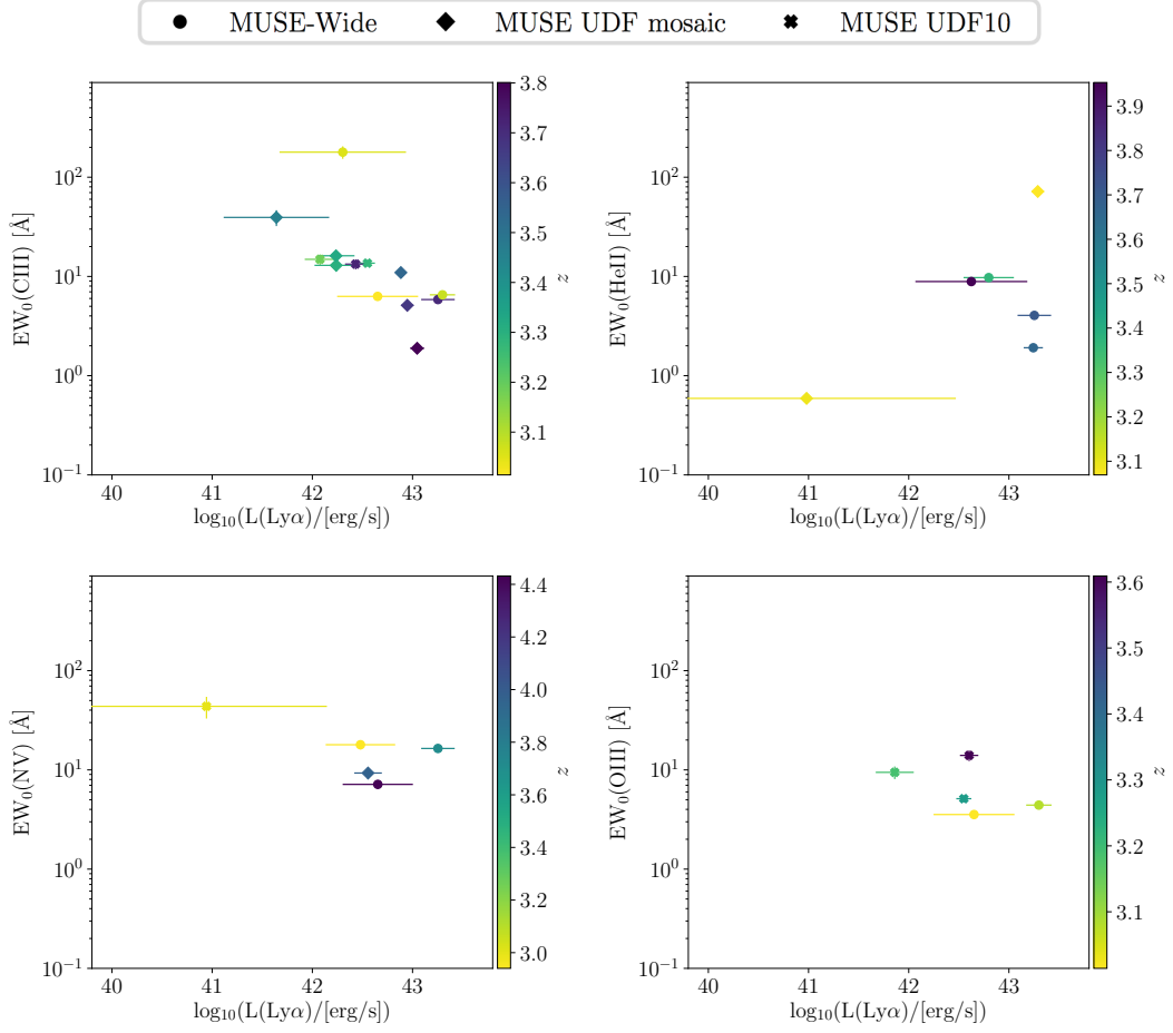
Fig. B.4. Potential correlations between \text{EW}_0(\text{C III}) , \text{EW}_0(\text{He II}) , \text{EW}_0(\text{N V}) , and \text{EW}_0(\text{O III}) and \log(L_{\text{Ly}\alpha}) described in Section 7.
