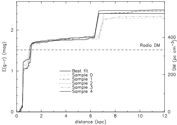
Figure 6. Colour-excess E(g-r) (left axis) and dispersion measure (DM, right axis) as a function of distance, derived from optical data, for the position of SGR J1935+2154, as extracted from the data of Green et al. (2019). Thin lines show the various sample data sets and the thick lines the best fit from Green et al. (2019). To calculate the dispersion measure Eq. 5 has been used.
