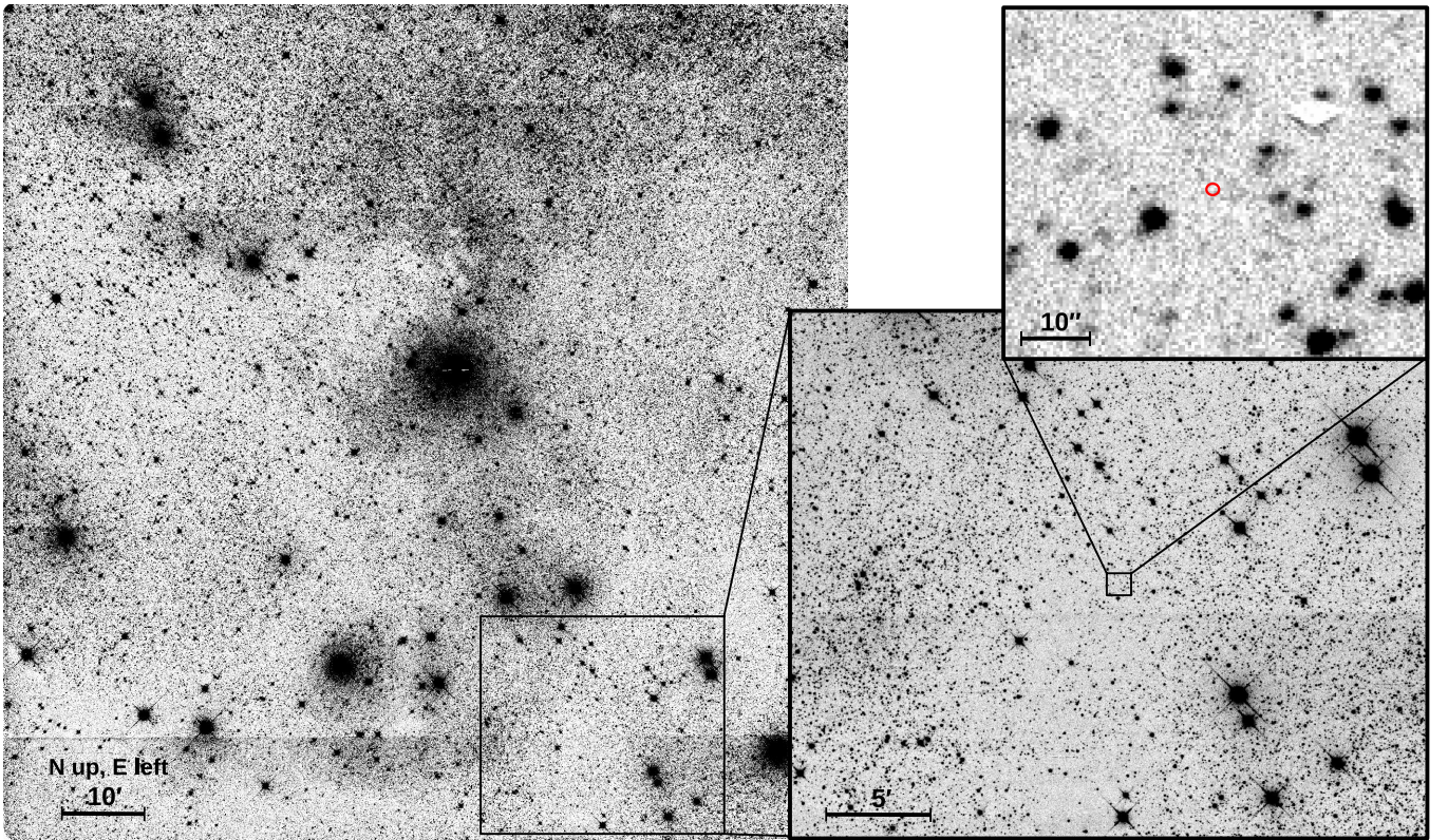
Figure 2. Co-added MeerLICHT q -band image of the field of SGR J1935+2154. Left, the full field with ID 11744, spanning 1.65^\circ \times 1.65^\circ . Darker regions, e.g. at the top, are the results of denser star field. Lighter regions show the effect of obscuring dust lanes. The horizontal stripe at the bottom is a low-level artefact of the border between two read-out channels. Bottom right, a 30' \times 30' zoom-in centered on the position of SGR J1935+2154 and matching the size and orientation of the MeerKAT supernova remnant image shown in Fig. 1. Top right, a 1' \times 1' close-up of the region centered on SGR J1935+2154. The red circle indicates the position of SGR J1935+2154. Faintest detected sources are at the level of AB_q=22.8 magnitude.
