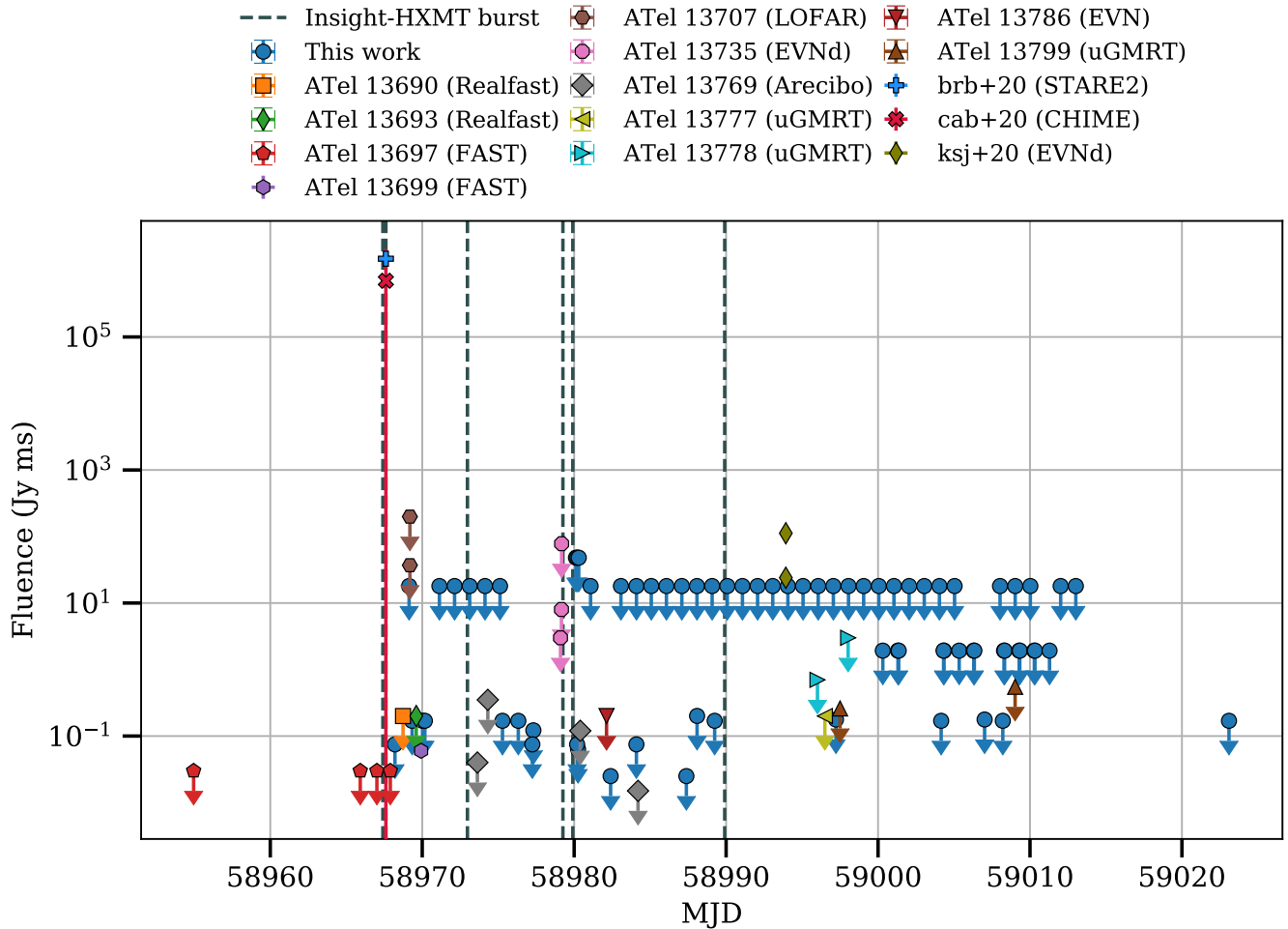
Figure 3. Timeline of the single-pulse fluence upper limits of SGR J1935+2145 at various radio frequencies as presented in this work, together with a selection of measurements from the literature. Fluences from this work are quoted for assumed burst widths of 1-ms (see Tables 2 and A1), except in the case of the low-frequency LOFAR observations, where pulse scatter-broadening effects likely dominate. Additionally, we mark the times of the brightest X-ray bursts with fluences > 10^{-7} erg cm ^{-2} reported by Insight-HXMT .
