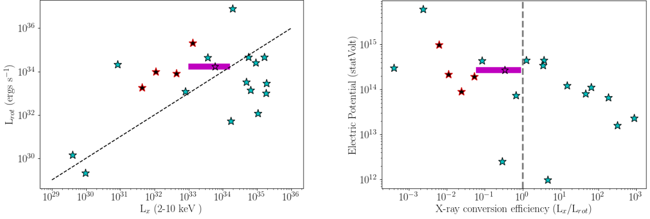
Figure 5. Left Panel: Spin-down Luminosity versus quiescent 2–10 keV X-ray luminosity of magnetars. The black dashed line represents the region where L_x = L_{rot} . Right Panel: Electric potential in the magnetosphere as a function of X-ray conversion efficiency. The grey dashed line corresponds to an efficiency of one. For both plots, cyan stars represent the magnetar population taken from the McGill Magnetar Catalog (Olausen & Kaspi 2014). The black stars with red outlines represent radio loud magnetars while SGR J1935+2154 is shown as the magenta star. The shaded region represents the range of values L_x and conversion efficiency based on the distance to the magnetar (see text for more details). The position of the magenta star corresponds to the distance of 6.6 kpc as used in Borghese et al. (2020a).
