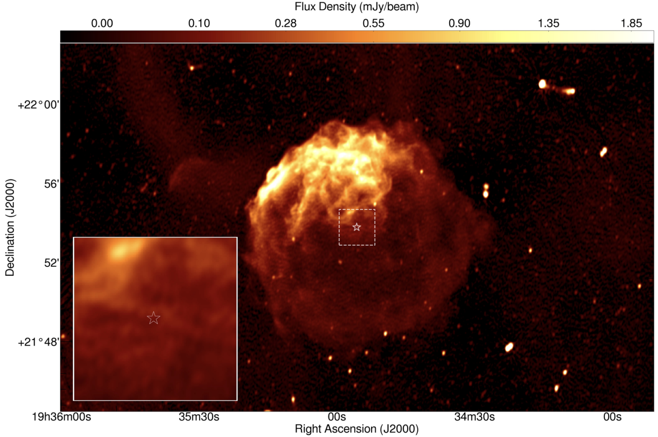
Figure 1. The inner 0.5^\circ \times 0.3^\circ of the target field, formed by combining the 11 May 2020 and 15 May 2020 MeerKAT observations. The position of SGR J1935+2154 is marked with a star, embedded in the emission from SNR G57.2+00.8 which dominates the field. The thermal noise in this image is approximately 5.2 \mu\text{Jy beam}^{-1} . The restoring beam in this image is a 2D Gaussian with an extent of 8.4'' \times 5.8'' (position angle 178 degrees, east of north). The inset panel shows a 1.8' \times 1.8' zoom on the location of SGR J1935+2154, as marked by the dashed box on the main panel. The colourmap has a square-root stretch function, and is the same for both panels. Pixel values in \text{mJy beam}^{-1} are indicated at the top of the figure.
