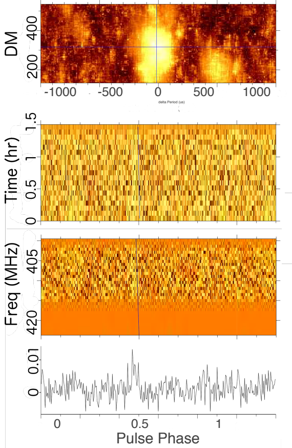
Figure 4. A radio pulse detected during observations of SGR J1935+2154 with the Northern Cross (obtained on 2020 May 30). Bottom to top the plots show: best integrated pulse profile (vertical axis is in arbitrary units); a waterfall plot of the frequency sub-bands versus pulse phase (the lighter the colour, the stronger the signal); a waterfall plot of time sub-integrations (5 minutes each) versus pulse phase; a color scale showing the S/N of the integrated pulse profile in function of the spin period and dispersion measure (brighter colors correspond to higher values). The values of P and DM maximising the S/N and corresponding to the bottom profiles are reported in the text. The optimised value of P is inconsistent with that derived from an ephemeris generated from NICER data.
