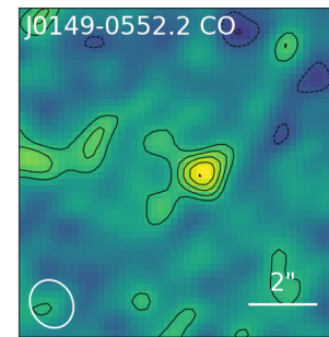
CO(4–3) maps
