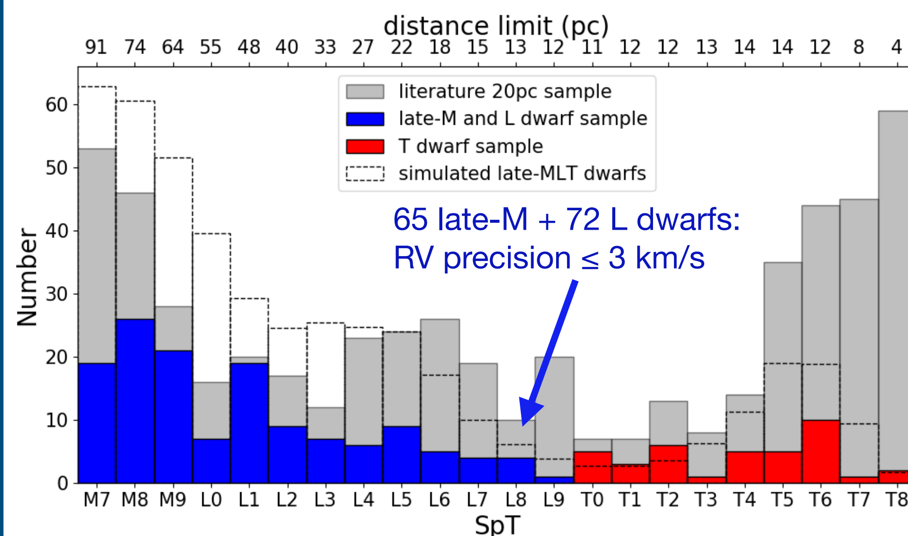
Figure 2. Spectral type distribution of our 20 pc late-M and L dwarf kinematic sample with RV uncertainty of \leq 3 km s -1 (blue histogram), and our NIRSPEC T dwarf sample (red histogram).
