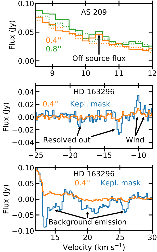
Figure 7. Zoom-in of the ^{12}\text{CO} J=2-1 spectra for the asymmetric features in AS 209 and HD 163296. Spectra in blue (HD 163296 only) are extracted by integrating over the cleaning mask in each channel, the orange spectra from a circular aperture of 0''.4 and the green spectra (AS 209 only) from a circular aperture of 0''.8 . The AS 209 spectrum also shows the mirror spectrum in green. All features have been labeled. The flux spike in AS 209 (top), most clearly seen in the 0''.8 spectrum, is assumed to be due to a noise spike. The excess emission on the blue size of HD 163296 (middle) is due to wind emission falling within the Keplerian mask, whereas the negative fluxes are due to the fringing caused by the strong and extended wind emission. On the red side of HD 163296 (bottom), strong negative fluxes are measured in the Keplerian mask as the disk is backlit by galactic CO emission at these velocities, creating negatives in the continuum subtracted images where there is dust emission.
