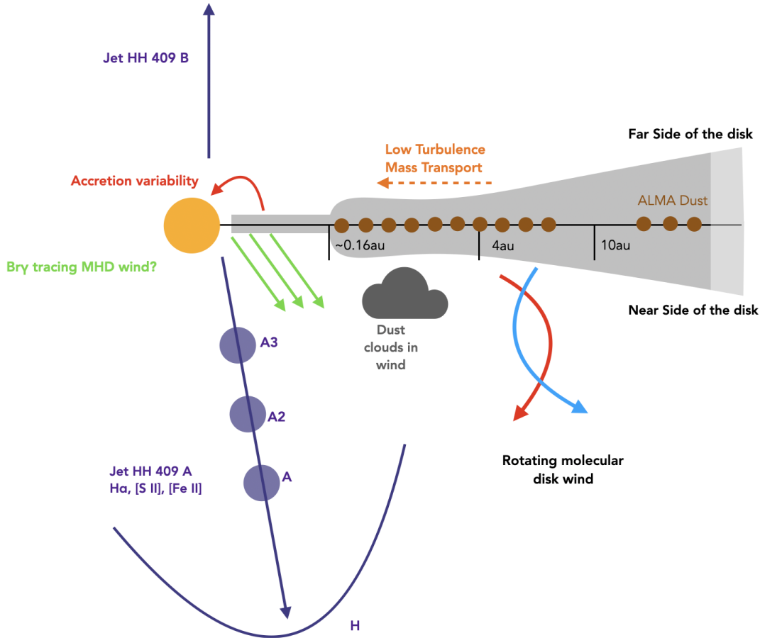
Figure 6. Cartoon summarizing the different mass-loss processes in the HD 163296 system. Note the ALMA observations presented here have a spatial resolution of 0''.3 ( \approx 30 au). These processes are not to scale and are for illustrative processes only.
