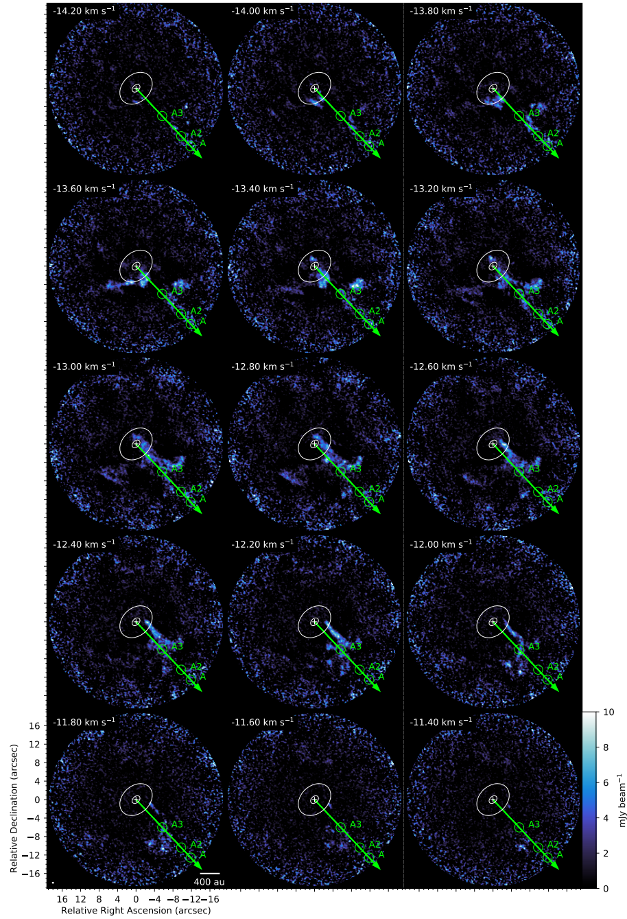
Figure 8. ^{12}\text{CO} J=2-1 channel maps with jet axis and knots labeled in green. Velocity axis is LSRK frame.
