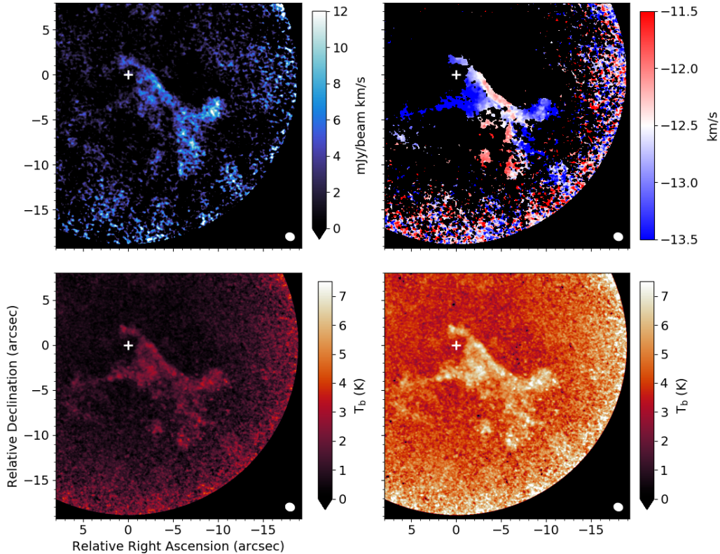
Figure 2. Top left: ^{12}\text{CO } J = 2 - 1 integrated intensity map. Top right: ^{12}\text{CO } J = 2 - 1 intensity-weighted velocity map in LSRK frame with a 4\sigma noise clip. Bottom: Peak brightness temperature maps made with the Rayleigh-Jeans approximation (left) and without (right). In all panels the beam size is shown by the ellipse in the bottom right corner.
