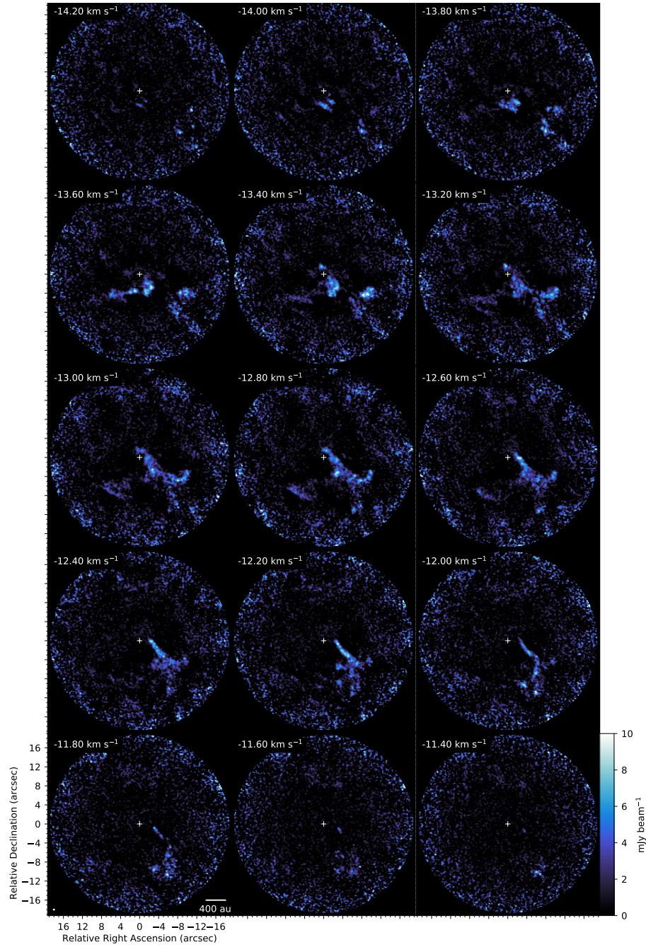
Figure 7. ^{12}\text{CO} J=2-1 channel maps. Velocity axis is LSRK frame.
