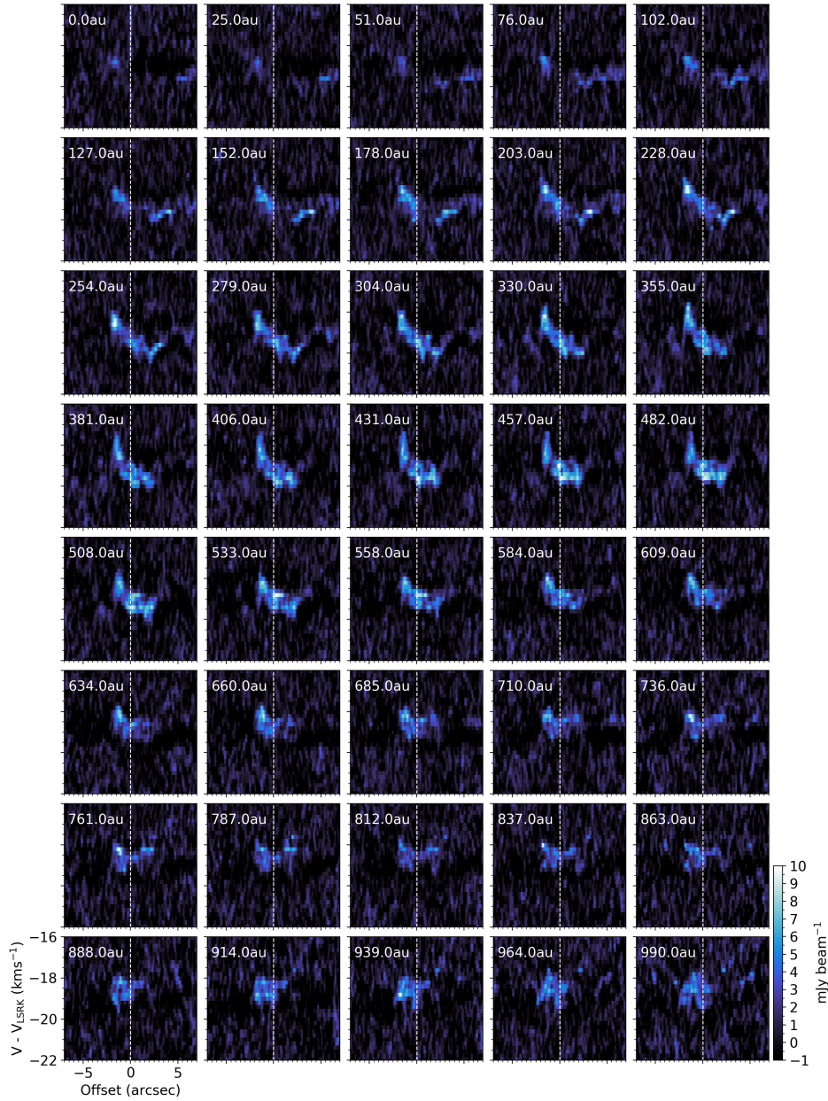
Figure 11. PV diagrams from the ^{12}\text{CO} J=2-1 channel maps. Cuts are taken perpendicular to the jet axis and each PV diagram is averaged over a strip the width of the beam major axis with the center of the cut in au noted in the top left of each panel. The velocity axis has been corrected for the velocity of the source.
