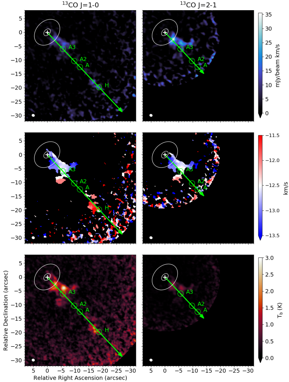
Figure 3. Integrated intensity (top), intensity-weighted velocity in LSRK frame (middle), and peak brightness temperature (bottom) maps for the ^{13}\text{CO } J = 1 - 0 and J = 2 - 1 lines. Ellipses are disk radii of 100 and 400 au. The green arrow highlights the axis of the jet and the circles highlight the position of the knots (A, A2, A3) and the bow shock (H) with corrections for proper motions. The beam size is shown by the ellipse in the bottom-left corner of each image and the star position is marked with a cross. A figure without annotations are shown in the Appendix in Figure 10
