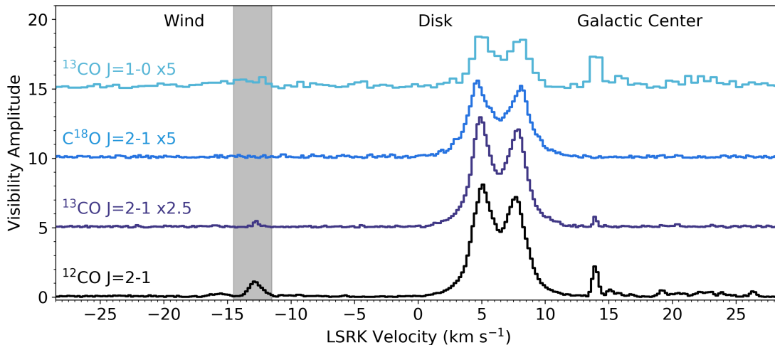
Figure 1. Average visibility spectra over the four shortest baselines for four CO isotopologues and transitions. The ^{13}\text{CO } J = 2 - 1 , \text{C}^{18}\text{O } J = 2 - 1 and ^{13}\text{CO } J = 1 - 0 data are offset by values of 5, 10, and 15 respectively, and multiplied by a factor noted on the figure for clarity. The velocity resolution for each line is noted in Table 1. The shaded regions highlight the CO tracing the blue-shifted disk wind (left) and CO from the Galactic center (right).
