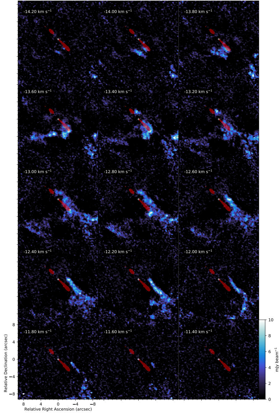
Figure 9. ^{12}\text{CO} J=2-1 channel maps with the jet traced in [SII] 673nm and \text{H}\alpha from Xie et al. (2020) overlaid in red. Velocity axis is LSRK frame.
