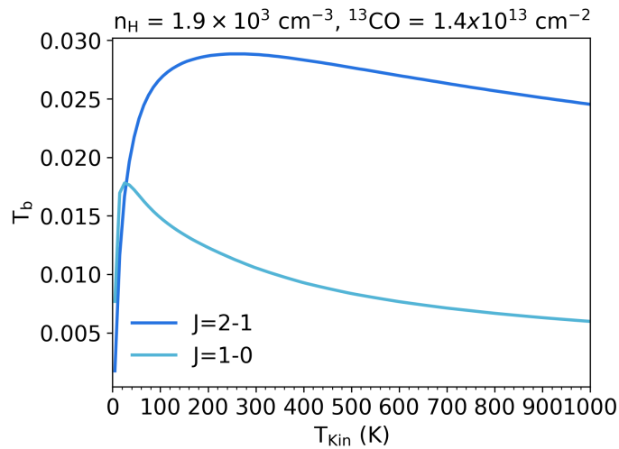
Figure 12. RADEX model brightness temperature ( T_b ) with a ^{13}\text{CO} column density of 10^{15}/70 \text{ cm}^{-2} to match values reported in Klaassen et al. (2013).
