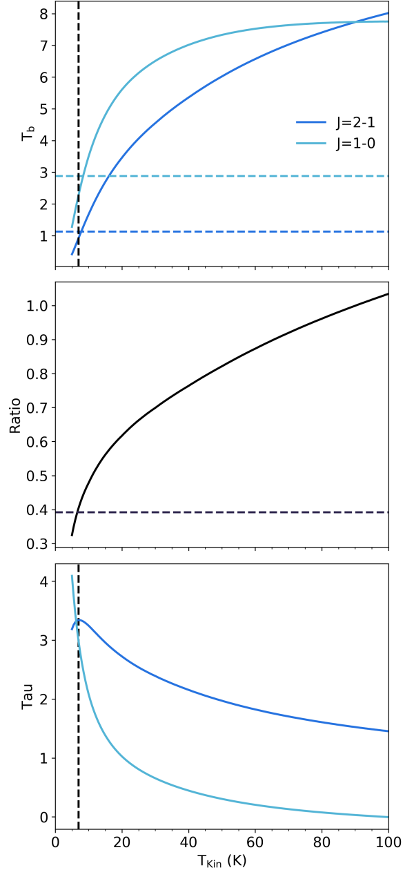
Figure 5. RADEX model results as a function of kinetic temperature T_{\text{Kin}} for the ^{13}\text{CO } J = 1 - 0 and J = 2 - 1 transitions assuming a line width of 1 \text{ km s}^{-1} , n_{\text{H}} of 10^3 \text{ cm}^{-3} and \Sigma(^{13}\text{CO}) of 4.7 \times 10^{15} \text{ cm}^{-2} . Top: brightness temperatures, T_{\text{b}} , from the model (solid lines), peak value from the observations (dashed horizontal lines) and best-fit kinetic temperature (dashed vertical line). Middle: J = 2 - 1 / J = 1 - 0 ratio from the model (solid line) and observations (dashed line). Bottom: optical depth, \tau , of both lines (solid lines) and best-fit kinetic temperature (dashed line).
