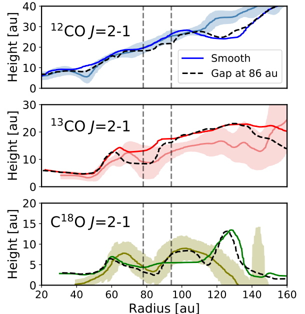
Figure 11. Emitting surface of ^{12}CO , ^{13}CO , and C^{18}O J=2-1 in a model that uses a depletion of CO (solid line), and a model that has a gap in the gas surface density at 86 au (dashed black line) as compared to observations (thick line).
