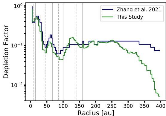
Figure 1. Multiplicative depletion factor for the initial CO abundance ( \text{CO}/\text{H}=1.4 \times 10^{-4} ) as shown in Table 2. Light gray lines indicate the location of the dust rings (solid) and gaps (dashed). The line in blue shows the CO depletion as derived by Z21 and is determined after an initial thermochemical model of the HD 163296 disk and is based on the \text{C}^{18}\text{O } J=2-1 observation, and acts as a starting point for our CO depletion determination. The green represents the final CO depletion, also motivated by the \text{C}^{18}\text{O } J=2-1 flux but is taken into account at the beginning of the chemical and thermal calculations.
