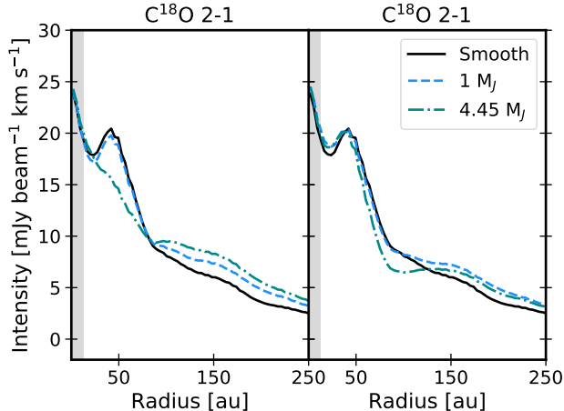
Figure 8. \text{C}^{18}\text{O} J = 2-1 radial profiles for a smooth model (black), a model with a gap in the small dust and gas population that corresponds to a 1 M_J planet (blue dashed), and 4.45 M_J planet (teal dashed). The left plot shows the results for a gap centered at 48 au, and the right a gap at 86 au.
