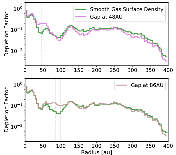
Figure 9. The calculated CO depletion for a smooth surface density model (green), and for a models with a gap at 48 au (top, pink) and 86 au (bottom, dark pink). The dashed grey lines correspond to the center of a gap, and the solid grey link corresponds to a ring. When imposing a gap in the total surface density, the CO depletion is flat or enhanced as opposed to being a local minimum at the location of the gap.
