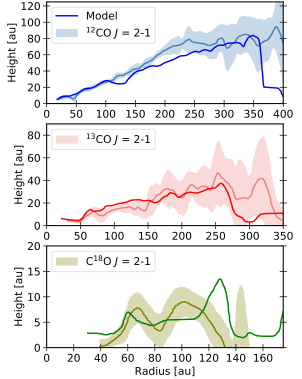
Figure 6. Derived emitting surfaces and calculated uncertainties of the 2-1 transitions of ^{12}\text{CO} , ^{13}\text{CO} , and \text{C}^{18}\text{O} . Observed emitting surfaces with calculated error is shown in blue, red, and green from Law & MAPS team (2021b) while the model emitting surfaces are in the brighter blue, red, and green without accompanied error.
