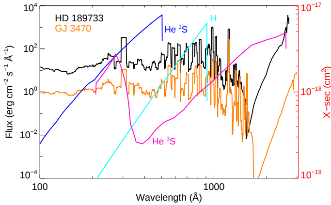
Fig. 2. Flux density (left y -axis) for HD 189733 (black) and GJ 3470 (orange) at 0.0332 and 0.0348 au plotted at a resolution of 10 Å, respectively. The H, He singlet, and He triplet ionisation cross sections (right y -axis) are also shown.
