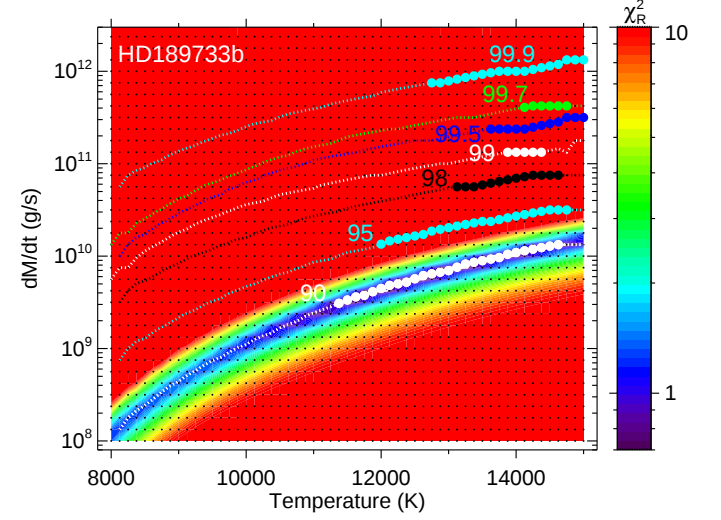
Fig. C.1. Contour maps of the reduced \chi^2 of the model of the helium triplet absorption for HD 189733 b for several H/He ratios (as in Fig. 4, left panel) when the turbulence broadening is not considered. The filled circles highlight the best fits (constrained ranges). The black dots represent the grid of the models.
