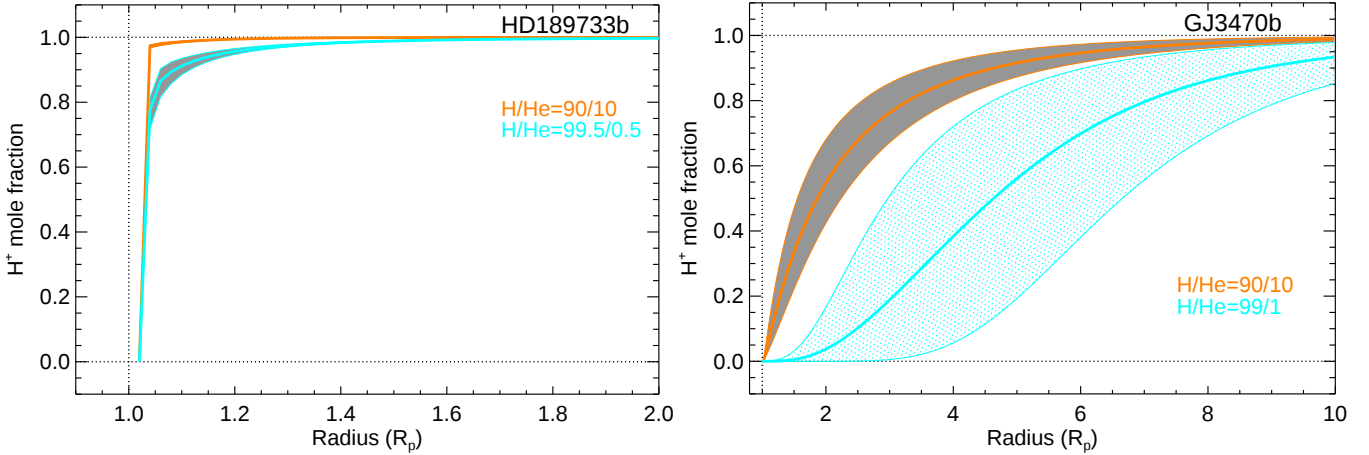
Fig. 8. H^+ mole fraction profiles resulting from the fit of the measured absorption (filled circles in Fig. 4) for H/He = 90/10 and 99.5/0.5 for HD 189733 b (left panel) and 90/10 and 99/1 for GJ 3470 b (right panel). We note the different x-axis range. The solid thicker lines are the mean profiles.
