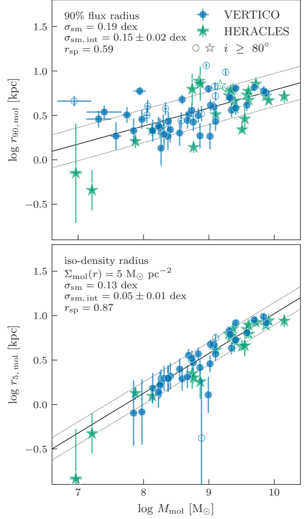
Figure 10. The molecular gas size–mass relation for 90% flux radii ( r_{90, \text{mol}} , upper panel) and inclination-corrected iso-density radii ( r_{5, \text{mol}} , lower panel). The former enclose 90% of the molecular gas flux (and thus mass for a fixed \alpha_{\text{CO}} ), while the latter are defined as the radius where \Sigma_{\text{mol}}(r) = 5 \text{ M}_{\odot} \text{ pc}^{-2} . Galaxies from the VERTICO and HERACLES surveys are denoted by blue and green points, respectively. The rms scatter ( \sigma_{\text{sm}} ), intrinsic scatter accounting for errors ( \sigma_{\text{sm, int}} ), and Spearman rank coefficient ( r_{\text{sp}} ) for the combined VERTICO–HERACLES relation are given in the upper left of each panel. The best-fitting relation for all galaxies is shown by the black solid line with \pm 1\sigma_{\text{sm}} denoted by the black dashed lines (see text for fit parameters). Galaxies with inclination \geq 80^\circ are denoted by open markers and not included in the fits to the data.
