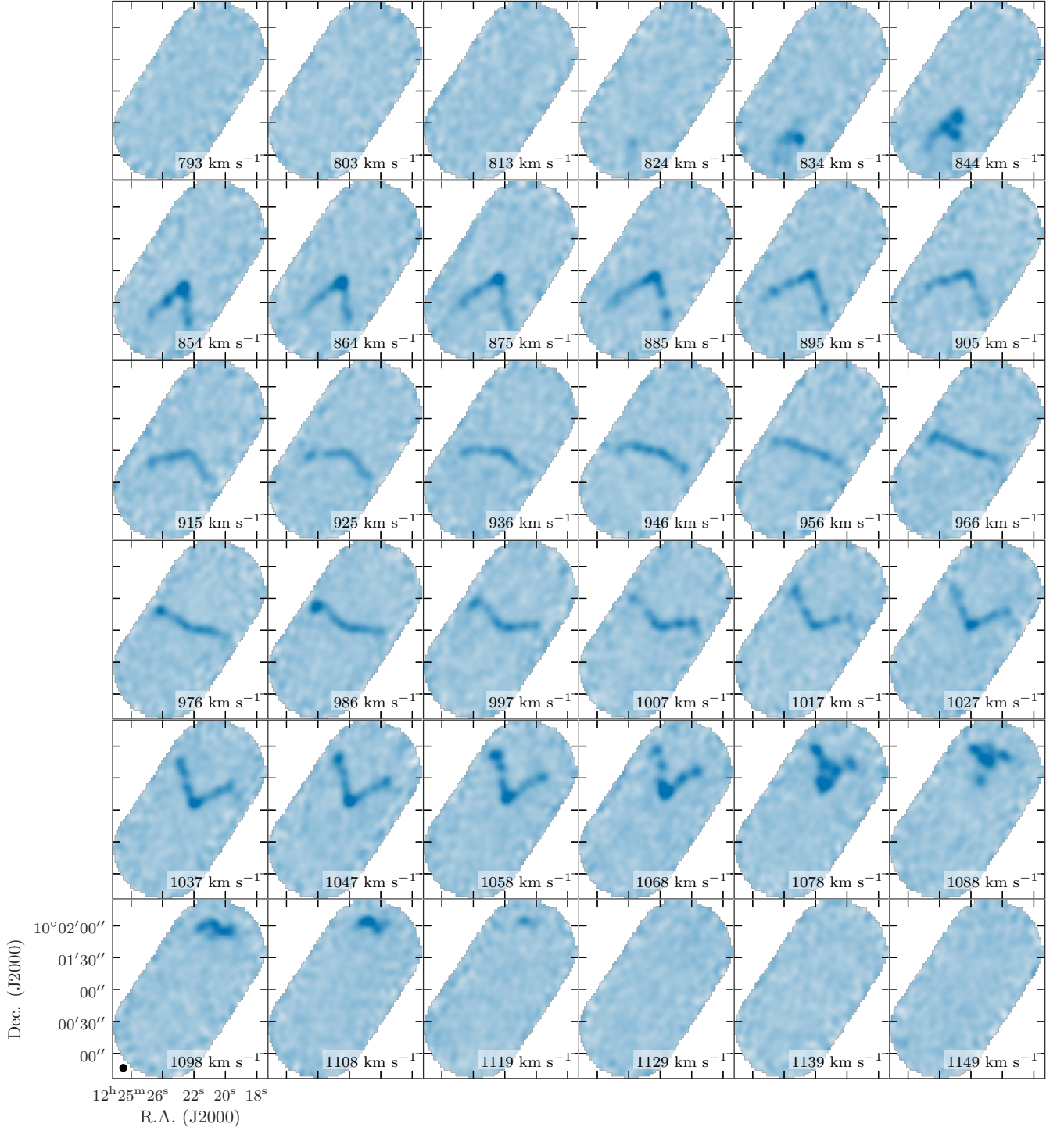
Figure 3. Channel maps for NGC4380. The circular beam size illustrated in the lower left panel is 7.5'', the channel width is 10.6 km s -1 , and the rms intensity in one channel is 3.5 mK. The systemic velocity of each channel is given in the lower right-hand corner. The color scale is fixed between channels.
