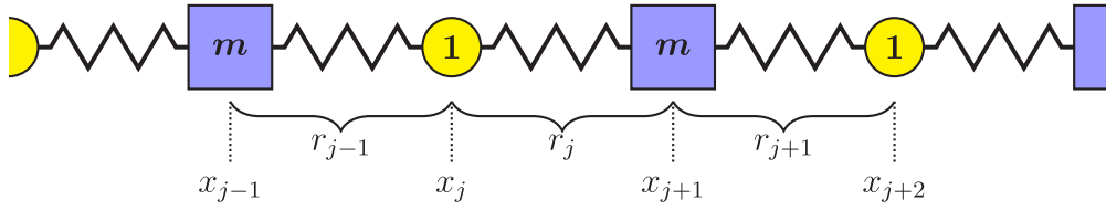
Fig. 1. The diatomic FPUT lattice, featuring alternating masses m and 1 connected by identical springs.
