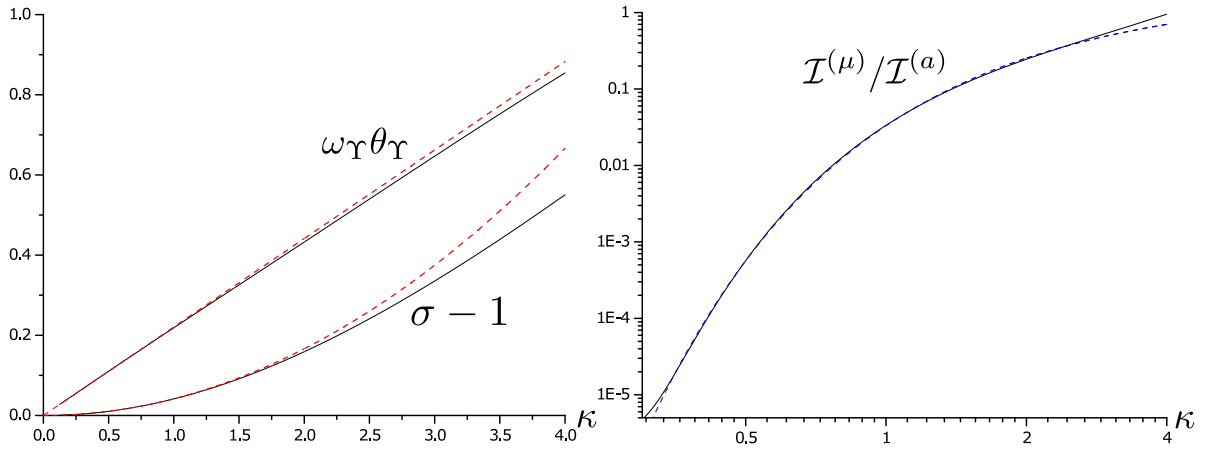
Fig. 4. The left graph visualizes the computed values for the asymptotic phase-shift of the Jost solution and the monatomic wave speed (solid black), together with their leading-order predictions (3.17) (dashed red). The right graph contains our computed values for -K_\sigma (solid black), together with the fit (3.18) (dashed blue). (For interpretation of the references to color in this figure legend, the reader is referred to the web version of this article.)
