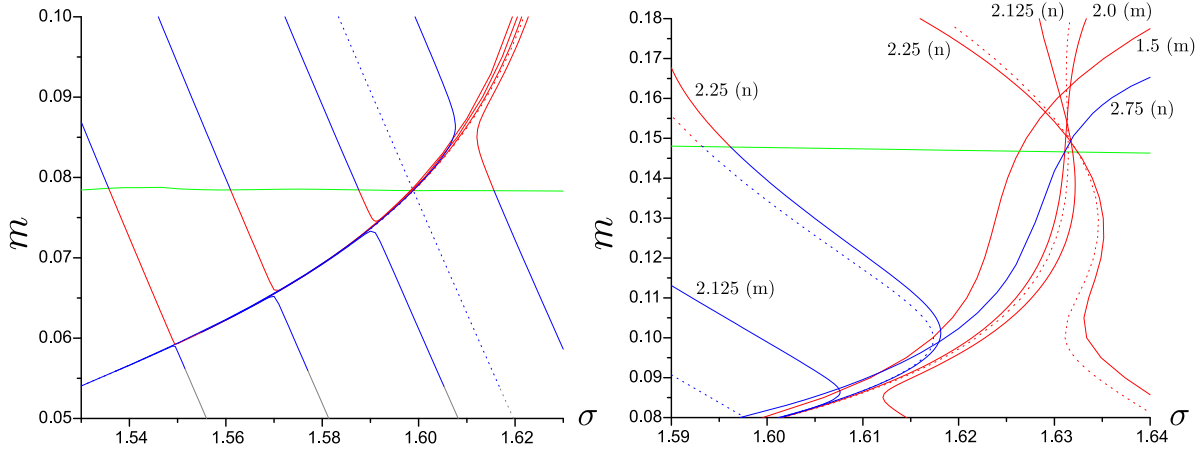
Fig. 6. Two zoomed views of interesting regions in Fig. 5. For presentation purposes, we only plot a subset of the iso- \kappa curves. The small numbers next to the curves in the right panel correspond to \kappa , while (n) and (m) stand for the nanopterons respectively micropterons branch. (For interpretation of the references to color in this figure legend, the reader is referred to the web version of this article.)
