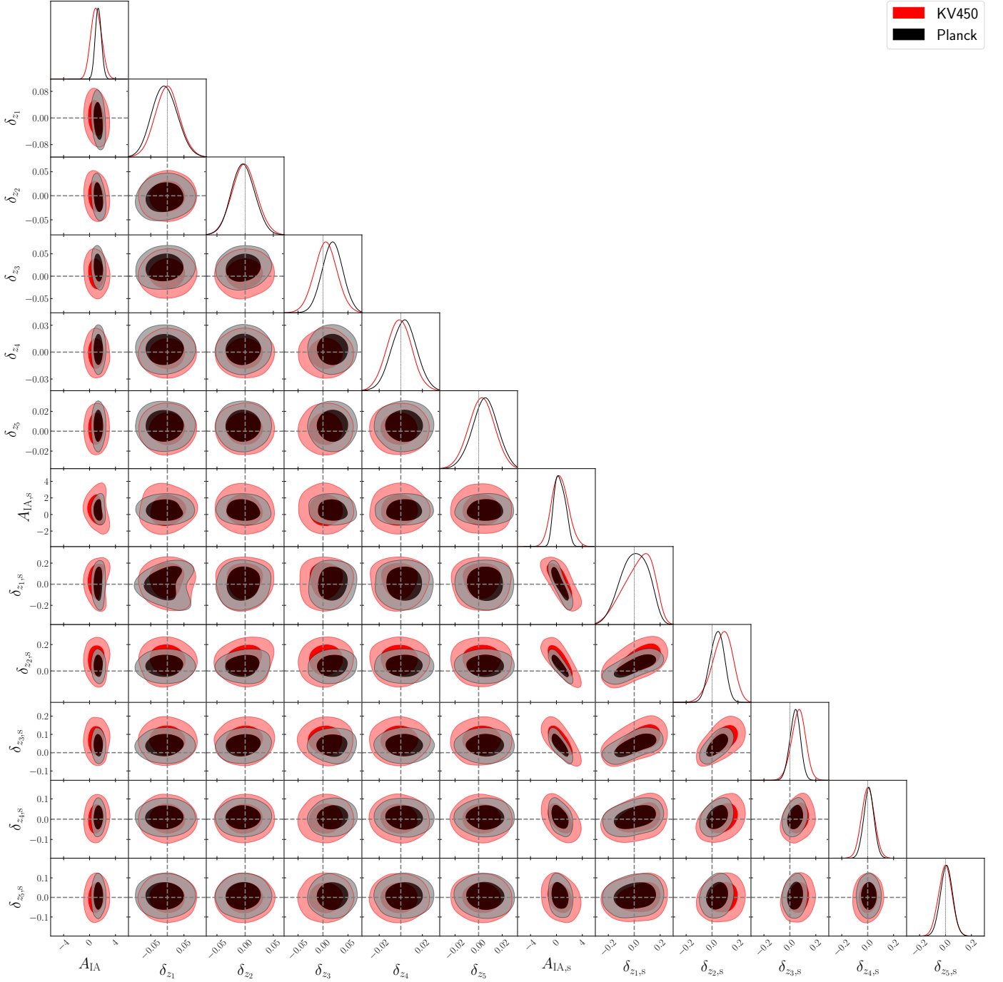
Fig. 8. Contour plots of the 68% and 95% credible regions for all the free parameters in \mathcal{H}_1 model. Plotting ranges are the same as the prior ranges. Dashed lines indicate the ideal case. Two different colours correspond to the two sets of results from KV450 and Planck cosmological values. The slight degeneracy between \delta_{z_i,s} in the low redshift bins is an effect from the high degeneracy between A_{IA,s} and \delta_{z_i,s} . It vanishes in the test setting \mathcal{T}_1 , where A_{IA,s} is fixed to zero.
