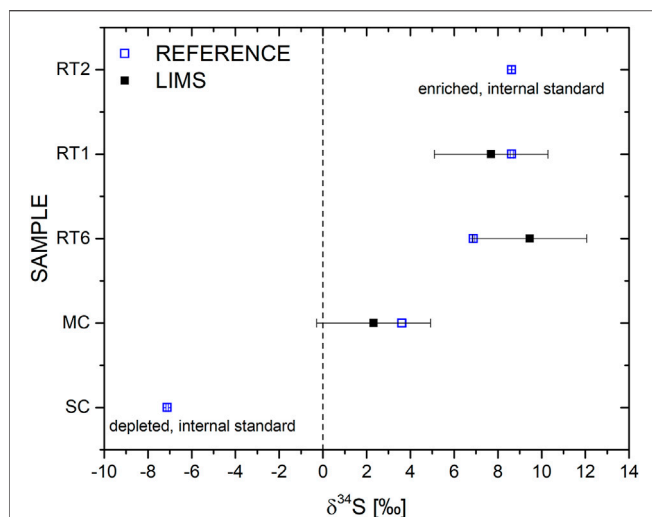
FIGURE 7 | Comparison between measured and reference values for \delta^{34}\text{S} . The LIMS measurements agree well with the reference values measured with state-of-the-art sulphur isotope analysis technique. The measurement accuracy is sufficiently high to provide valuable information on geochemical processes or to indicate life in case of the presence of sulphate-reducing bacteria, which may fractionate sulphur isotopes clearly above \delta^{34}\text{S} = -20\text{‰} .
