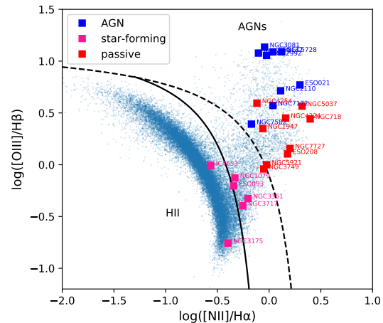
Fig. 11: BPT plot with [N II]/H\alpha vs. [O III]/H\beta . Galaxies from the AGN as well as the control sample of star-forming and passive galaxies are shown in blue, deep pink, and red, respectively. The empirical (Kauffmann et al. 2003) and theoretical (Kewley et al. 2001) boundaries between starburst and AGN galaxies are marked with black straight and dashed lines, respectively. The underlying blue cloud of points is from the MPA-JHU emission line analysis of SDSS DR7 galaxies (Brinchmann et al. 2004).
