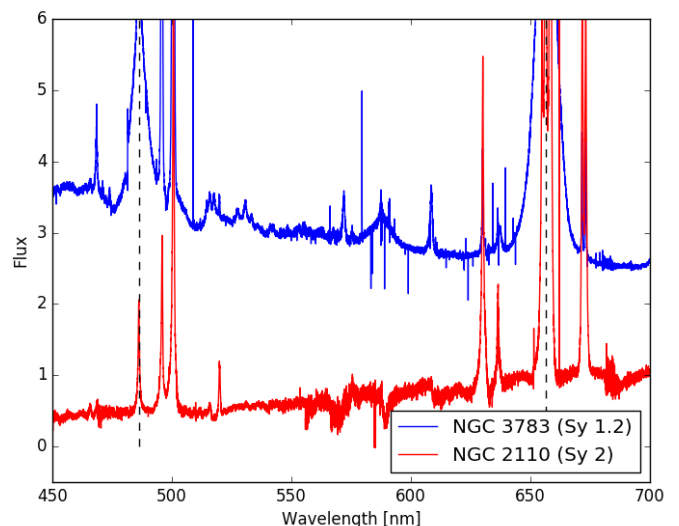
Fig. 1: Comparison of spectra for a Seyfert 1 and a Seyfert 2 galaxy from the LLAMA sample. A number of very broad emission features can be seen in the Seyfert 1 galaxy that outshine any underlying stellar absorption lines. The Balmer emission lines H\alpha and H\beta at 6562.8 Å and 4861.3 Å, respectively, are indicated with dashed lines.
