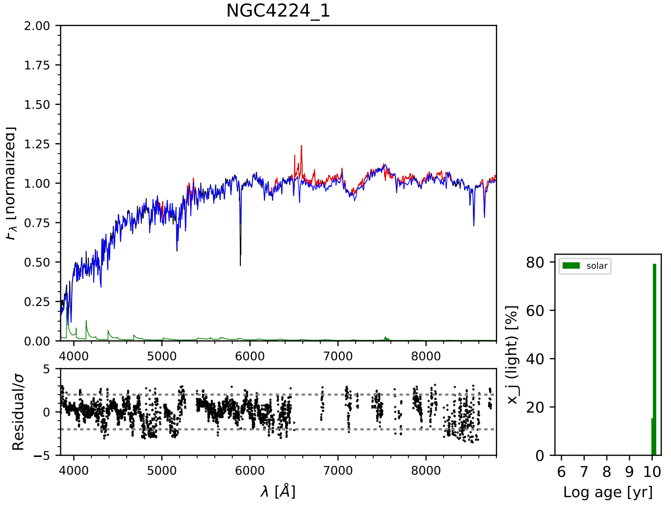
Fig. A.12: As Fig. 6, but for NGC 4224
