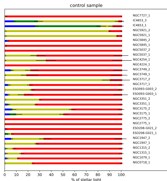
Fig. 5: Same as Fig. 4, but for the control sample.
