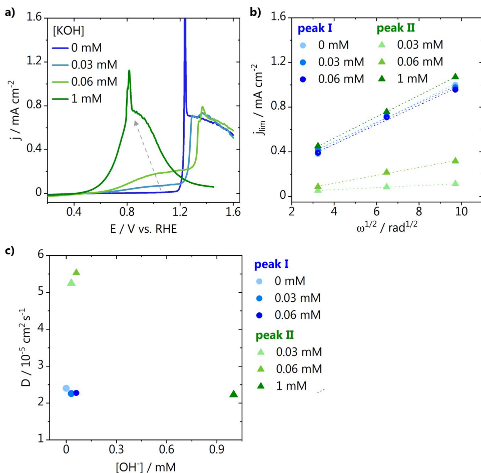
Fig. 5.5. RDE CO oxidation measurements on a polycrystalline Pt disc in \text{Cs}_2\text{SO}_4 (pH = 7.2) performed at 400 rpm with 25 \text{mV s}^{-1} scan rate. a) Reaction performed in the presence of different concentrations of KOH, b) Levich plot and c) derivation of the diffusion coefficients for peak I (blue circles) and peak II (green triangles).
