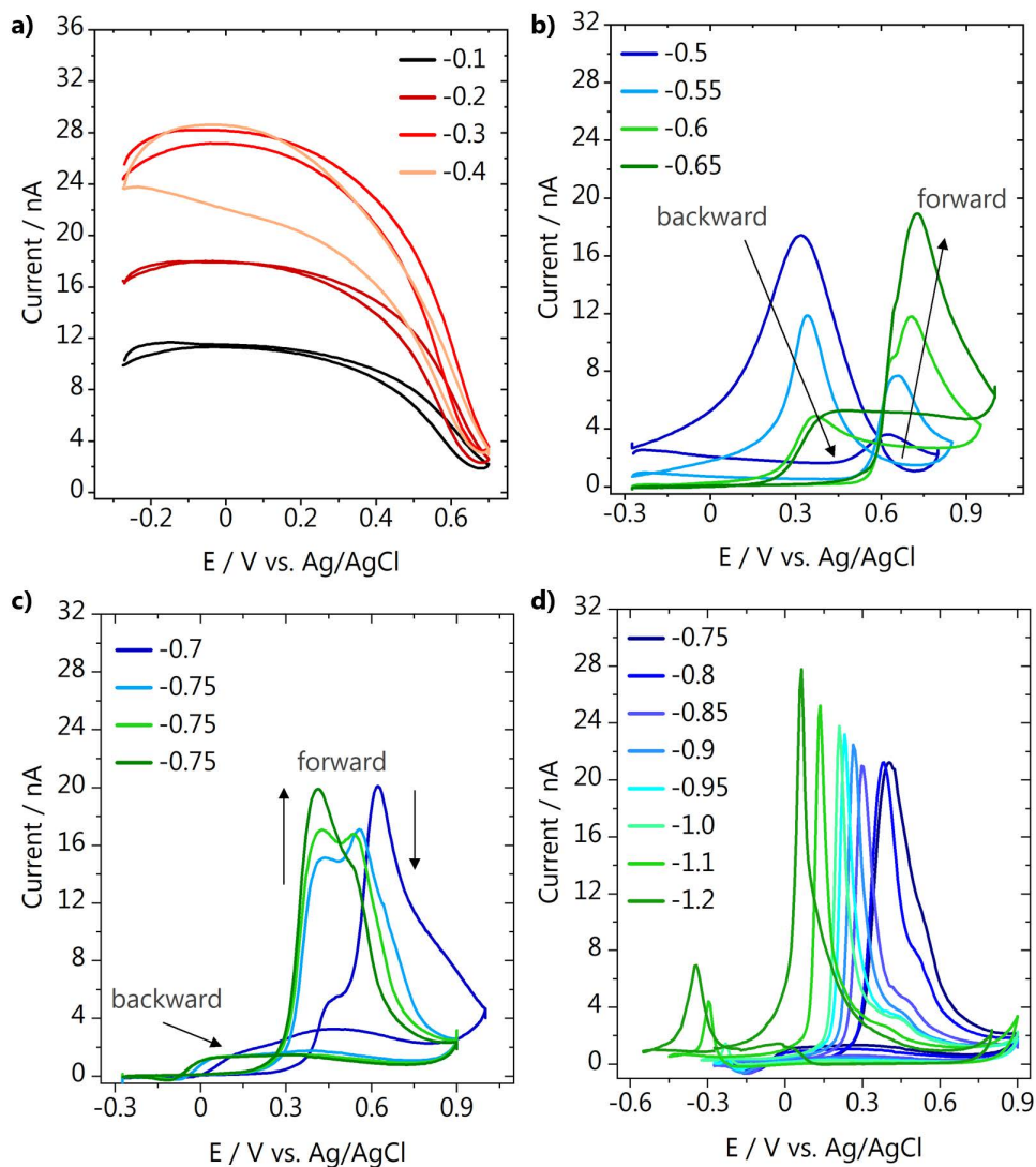
Fig. 5.2. Pt-UME voltammetry recorded in 0.1 M \text{Cs}_2\text{SO}_4 (200 \text{mV s}^{-1} , pH = 3) while \text{CO}_2\text{RR} and/or HER take place at the gold sample at potentials a) from -0.1 to -0.4 V, b) from -0.5 to -0.65 V, c) from -0.7 to -0.75 V and d) from -0.75 to -1.2 V. The gold sample potentials shown in the legend are reported versus the reversible hydrogen electrode.
