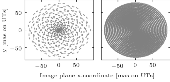
Fig. 3. Examples of the scanning pattern applied in the Calibration Unit measurements. SC aberration maps were obtained with a slow modulation frequency (left). For the corresponding FT measurement, a faster scanning was used, and the right panel only shows a single iteration of in- and out-spiral.
