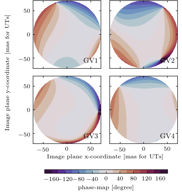
Fig. 5. Science channel phase maps obtained from fits to the differential SC-FT maps, measured on 03/03/20 for all four GRAVITY beams.
