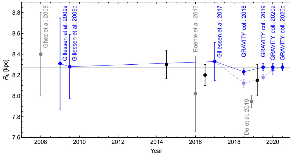
Fig. 11. Measurements of the Galactic Center distance over time with a focus on studies of the S2 orbit. Blue points show results obtained with the SINFONI, NACO and GRAVITY data with (dark blue) and without (light blue) application of the aberration corrections. Gray R_0 determinations are based on data from the Keck observatory. For comparison, we show in black results based on the statistical parallax of the nuclear star cluster (Chatzopoulos et al. 2015) and from modeling the Milky Way dynamics based on observations of molecular masers (Reid et al. 2019). Bland-Hawthorn & Gerhard (2016), finally, give the GC distance based on a combination of various methods.
