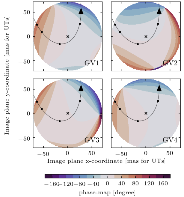
Fig. 9. The orbit of S2 relative to the phase maps as applied for the GC analysis (measurement from 03/03/20, \sigma_i = 10 mas). Dots indicate the position of S2 on 2017.2, 2017.6, 2018.2 and 2018.7, respectively, while the cross marks Sgr A*.
