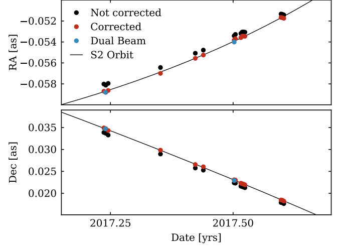
Fig. 12. Detailed view of the S2 orbit in 2017. Dual-beam points do not suffer from aberration-related systematic errors and agree very well with our corrected data points.
