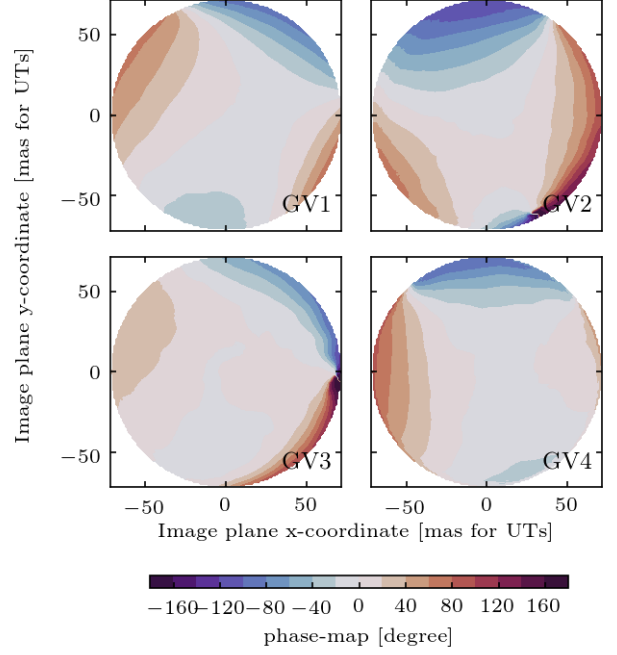
Fig. 4. Science channel phase maps reconstructed by the procedure of Sec. 3.1 from the Calibration Unit measurement on 03/03/20 for all four GRAVITY beams.
