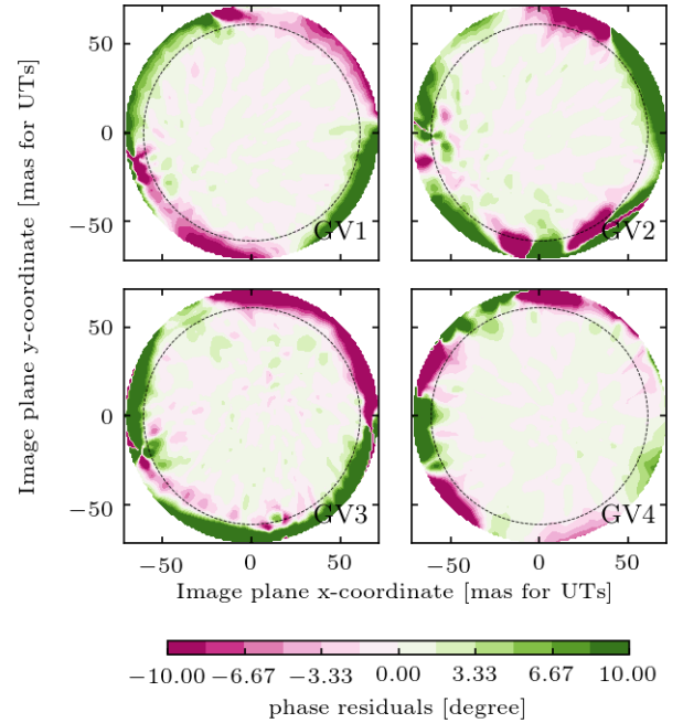
Fig. 6. Phase residuals of the fit to the differential SC-FT map measured on 03/03/20 for all four GRAVITY beams. Only the data within the dashed circle is considered in the fit; at larger radii the cancellation of wavelength-dependent scaling errors is not guaranteed.
