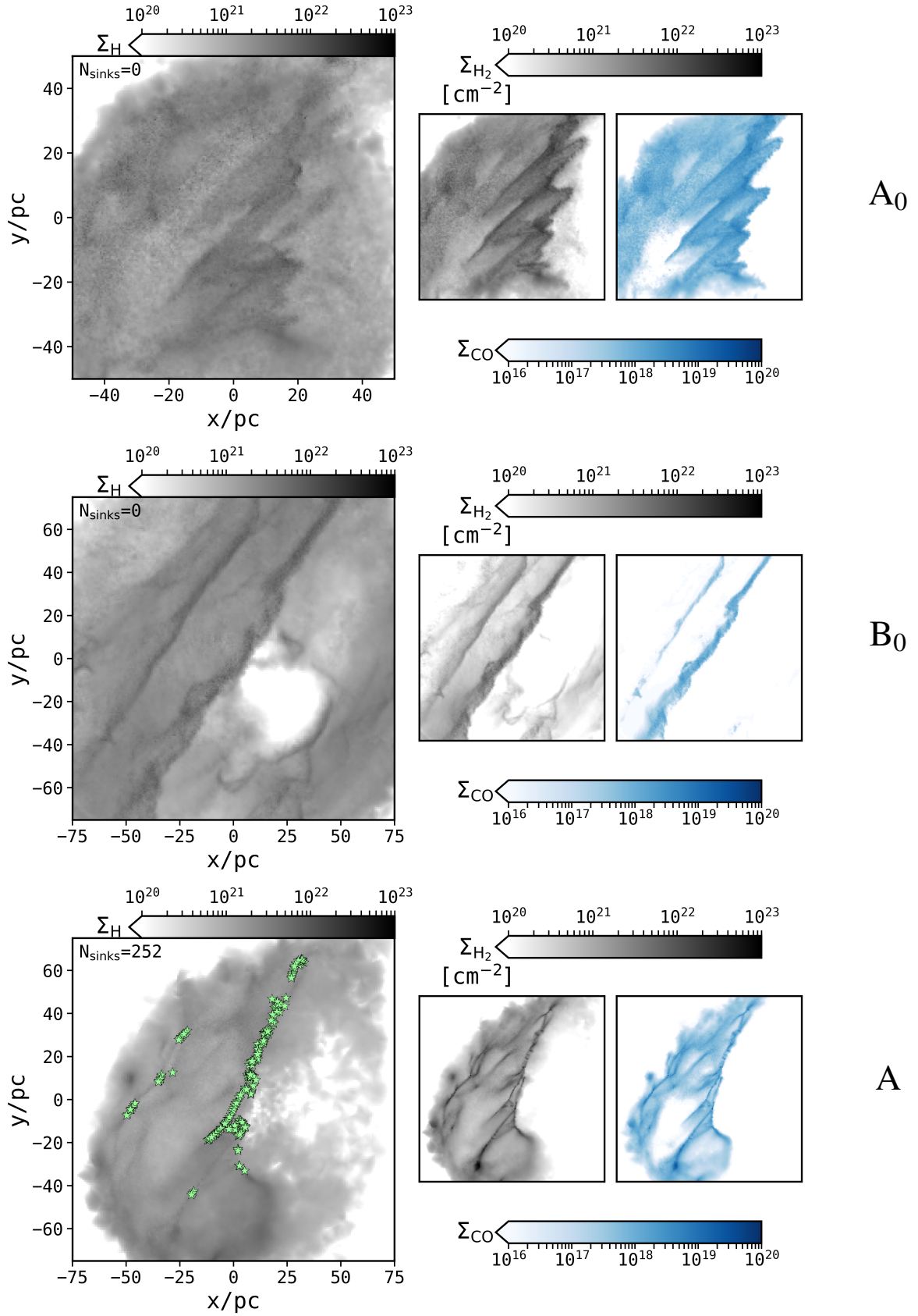
Figure 1. Face-on projections of \text{H} , \text{H}_2 and ^{12}\text{CO} column densities ( \Sigma ) from cloud complexes (labeled on the right) extracted 2 Myr after injecting tracer particles in the simulations. If any, sink particles are overlaid on \text{H} maps as star markers.
