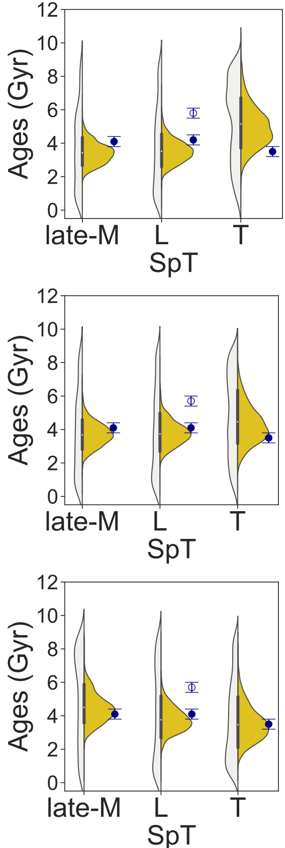
Figure 26. Same as Figure 21 comparing three simulations with baseline parameters and mass functions that evolve over time: (Top) \alpha = 1.5 \rightarrow -0.5 (bottom-heavy to top-heavy; same model as Burgasser et al. 2015b); (Middle) \alpha = 1 \rightarrow 0 (bottom-heavy to top-heavy); and (Bottom) \alpha = 0 \rightarrow 1 (top-heavy to bottom-heavy).
