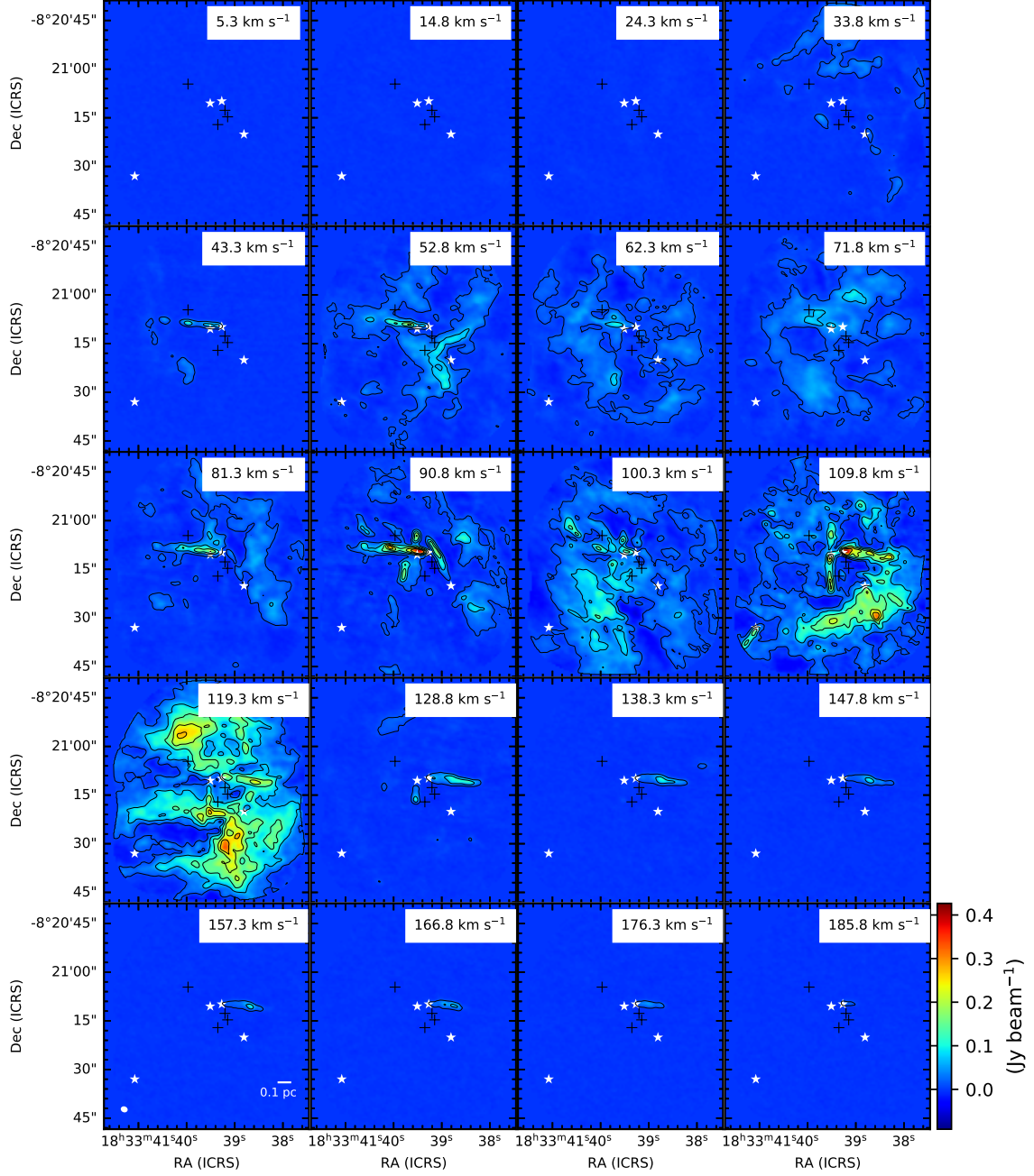
Figure 18. Channel maps of CO ( J=2-1 ). The contour levels are 10, 50, 100, 150, and 200\sigma ( 1\sigma=1.35 \text{ mJy beam}^{-1} ). The white star symbols represent the continuum peak positions of cores (ALMA2, 3, 4, and 8) associated with outflows. The plus symbols represent the continuum peak position of ALMA1, 5, 6, and 7 (no outflow). The spatial scale and the beam size are shown at the bottom.
