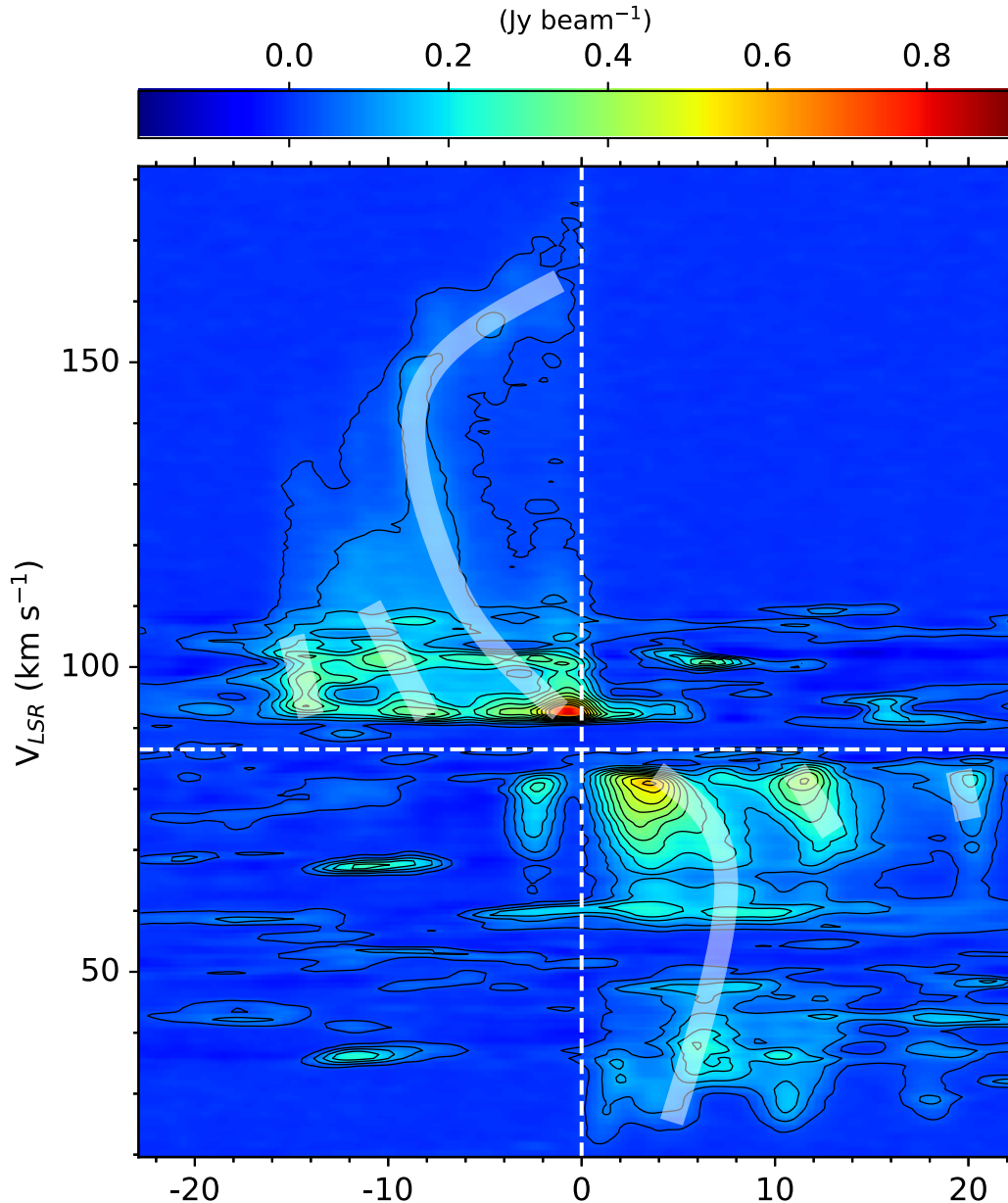
Figure 10. Position-Velocity (PV) diagram of CO emission for ALMA3. The cut of the PV diagrams is along the CO outflow (P.A. = \sim 81^\circ ) with width=3 pix (1 pix=0.2"). The contour levels are 3\sigma , 10\sigma to 230\sigma by 20\sigma steps ( 1\sigma=2.64 \text{ mJy beam}^{-1} ). The white curved lines shows the S-shape structure, and white lines show the knotting structure called Hubble wedges. The vertical white dashed line is the position offset=0, and the horizontal one corresponds to the systemic velocity of this region.
