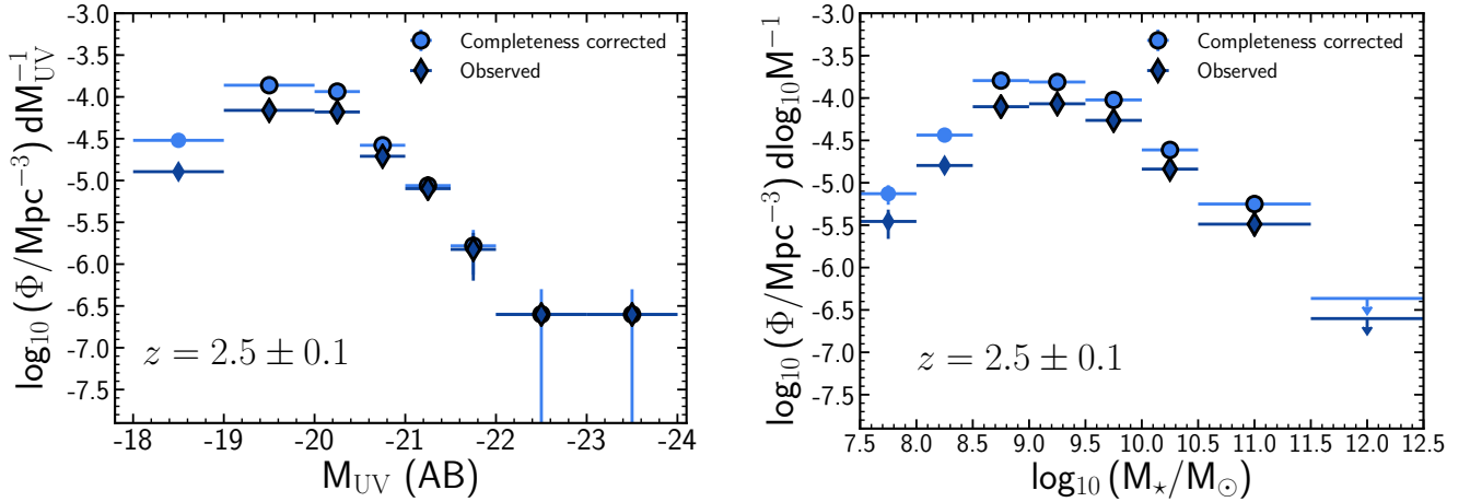
Figure 2. Left: The rest-frame UV LF for the z = 2.5 (IA427) sample of LAEs. We show the luminosity values before (dark blue diamonds) and after (blue circles) applying the completeness correction. The completeness correction is based on Ly \alpha flux (selection criteria). Since M_{\text{UV}} and L_{\text{Ly}\alpha} typically correlate (see Fig. 1, left panel), the completeness corrections are larger for the faintest M_{\text{UV}} bins. Right: Same but for the SMF. As the correlation between L_{\text{Ly}\alpha} and M_{*} is shallower (see Fig. 1, right panel), completeness corrections are not a strong function of stellar mass for a specific Ly \alpha cut.
