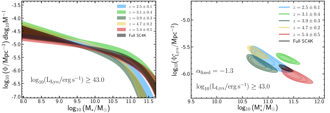
Figure 10. Left: Evolution of the SMF with redshift, with a luminosity cut of \log_{10}(L_{\text{Ly}\alpha}/\text{erg s}^{-1}) \geq 43.0 . Right: \Phi^*-M_* 1\sigma , 2\sigma and 3\sigma contours. With a uniform cut for the entire sample, we do not observe clear evidence of evolution with redshift of the SMF of LAEs. We find little M_* and \Phi^* evolution with redshift, remaining constant at \log_{10}(M_*/M_\odot) \sim 11 and \log_{10}(\Phi^*/\text{Mpc}^{-3}) \sim 5.8 .
