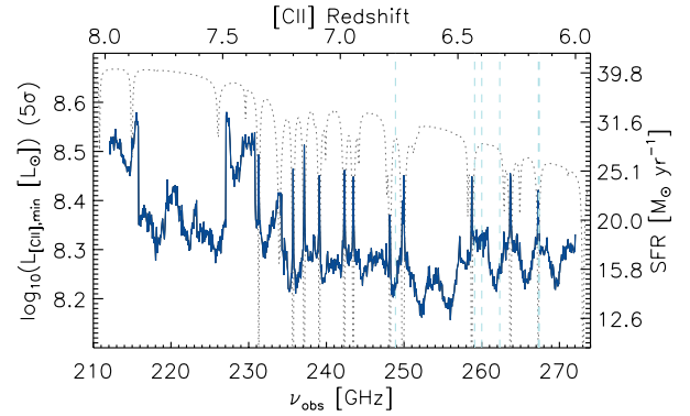
Figure 1. [CII] luminosity depth ( 5\sigma ), assuming 200 \text{ km s}^{-1} line width, across the survey bandwidth. The corresponding limit in SFR (right ordinate) is derived using a locally calibrated L_{\text{[CII]}} -SFR relation for star-forming galaxies (De Looze et al. 2014). Dashed (light blue) vertical lines indicate the expected \nu_{\text{obs}} for the [CII] line based on the Ly \alpha redshift for the MUSE LAEs in the sample defined in Section 2.2: MUSE 852, 6332, 6312, 6524, 802, 560, in order of decreasing redshift. (Note that the vertical lines for MUSE 802 and 560 at the far right are nearly overlapping due to the proximity in redshift.) For illustrative purposes only, we have also plotted the atmospheric transmission (assuming PWV = 1 mm; dark gray, dotted curve) to show the effect of the atmospheric absorption features on the survey depth.
