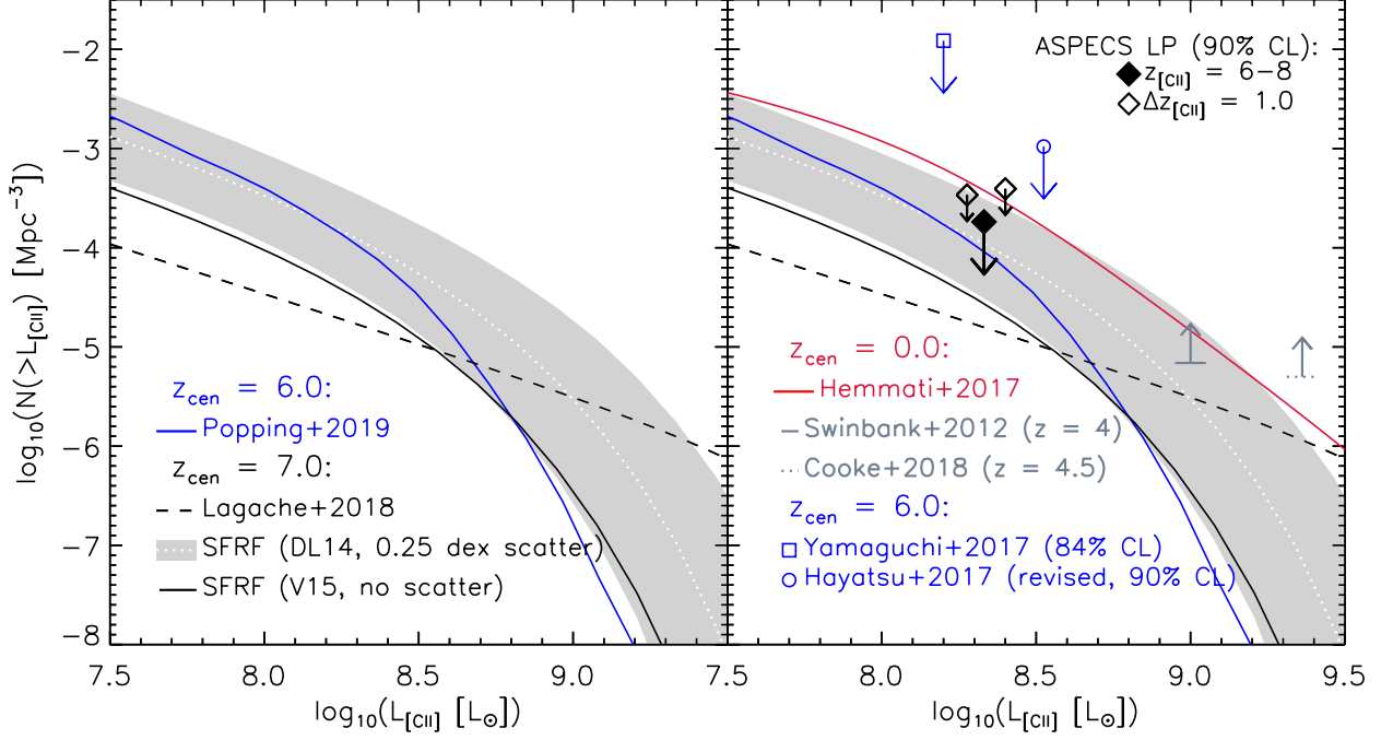
Figure 6. (left:) Theoretical predictions for N(> L_{\text{[CII]}}) vs. L_{\text{[CII]}} at z = 6 (blue curve: Popping et al. (2019)) and z = 7 (white dotted curve: best fit for simulated number densities based on the Smit et al. (2016) SFRF convolved with L_{\text{[CII]}} -SFR relation from the De Looze et al. (2014) HII region/starburst calibration, including a 0.25 dex scatter on L_{\text{[CII]}} -SFR shown as the gray band; black solid curve: same as white dotted curve, except using L_{\text{[CII]}} -SFR relation from Vallini et al. (2015) ( 0.2 Z_{\odot} ); black dashed curve: Lagache et al. (2018)). (right:) Observational constraints on N(> L_{\text{[CII]}}) vs. L_{\text{[CII]}} , with upper limits (90% confidence level) derived from the full ASPECS survey volume covering z = 6-8 (filled black diamond) and the literature at z \sim 6 (Yamaguchi et al. 2017; Hayatsu et al. 2017). The [CII] cumulative number densities measured at z \sim 0 (Hemmati et al. 2017), and lower limits at z \sim 4-5 (Swinbank et al. 2012; Cooke et al. 2018) are plotted as the gray arrows. Theoretical predictions from the left panel are underlaid to facilitate comparison.
