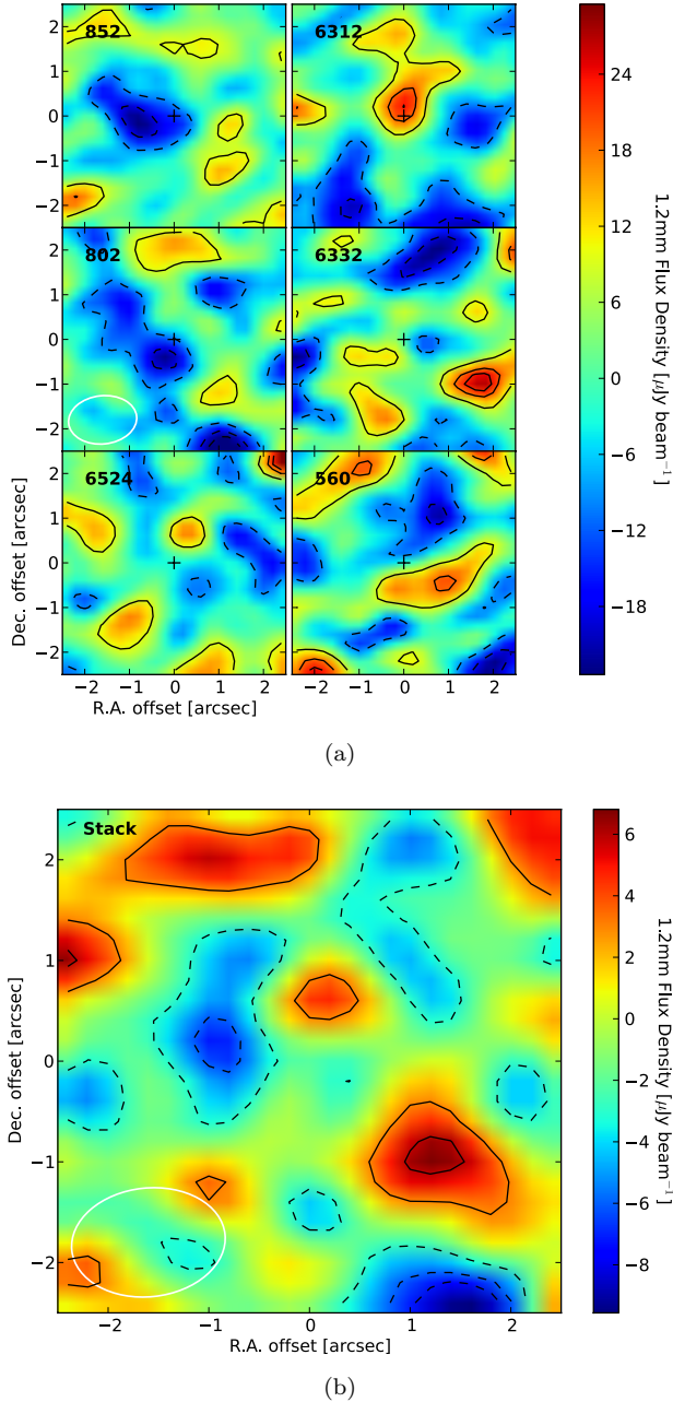
Figure 4. (a): 5'' \times 5'' postage stamps of 1.2 mm continuum images (without PB correction) centered at locations of MUSE LAEs in ASPECS. The LAE position in each cutout is indicated with “+” symbol; refer to Table 1 for sky coordinates. (b): Mean 1.2 mm continuum emission obtained by stacking on the locations of the six MUSE LAEs shown in the lefthand panel. Contours in both panels represent the emission at 1.0\sigma ( = 9.3\mu\text{Jy beam}^{-1} ), 2.0\sigma , and 2.5\sigma levels, with dashed and solid contours corresponding to negative and positive flux densities, respectively. For reference, the synthesized beam is shown as an ellipse in the bottom left corners of the postage stamp for MUSE 802 and the stack.
