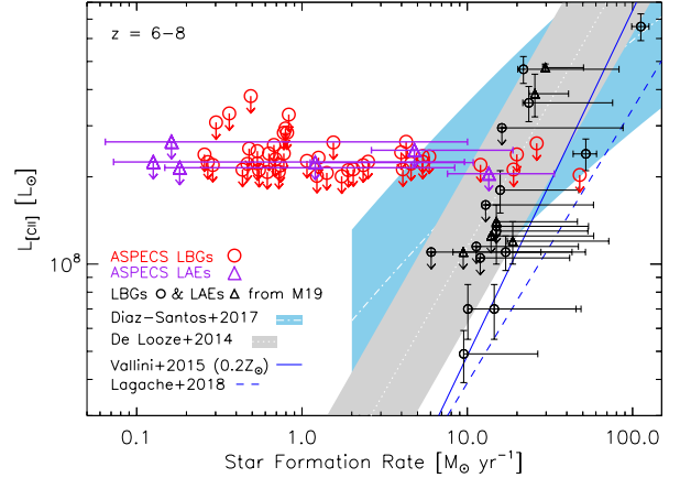
Figure 5. L_{\text{[CII]}} -SFR relation at z > 6 , with data points distinguished by target selection: circle and triangle symbols reflect galaxies initially discovered as LBGs and LAEs, respectively. 5\sigma upper limits on L_{\text{[CII]}} are presented for LBGs (red circles) and MUSE LAEs (purple triangles) within the ASPECS HPBW and redshift coverage. Detections and 5\sigma upper limits from the literature, as compiled by Matthee et al. (2019), are shown for comparison as black symbols. Also shown are the local L_{\text{[CII]}} -SFR relations calibrated by De Looze et al. (2014) for HII region/star-forming systems, including starbursts (dark gray band; 1\sigma dispersion = 0.27 dex), and by Díaz-Santos et al. (2013) for (U)LIRGs (light blue band; 1\sigma ); white dotted lines within each band indicate the best-fit relations for each sample. Theoretical predictions for the L_{\text{[CII]}} -SFR relation at z = 6-7 are plotted from Vallini et al. (2015) and Lagache et al. (2018) (solid and dashed blue line styles, respectively).
