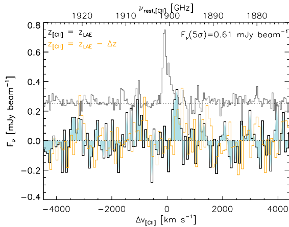
Figure 3. Stacked B6 spectra for the 6 MUSE LAEs in ASPECS, assuming that the [CII] redshift matches exactly the Ly \alpha redshift (blue filled curve) or an empirically derived systemic redshift per (Verhamme et al. 2018) (orange curve). The stacked Ly \alpha spectrum is also shown for comparison (gray curve), with arbitrary flux density normalization. The 5\sigma rms F_\nu(5\sigma) = 0.61 mJy beam ^{-1} reported here refers to the B6 stacked spectrum computed without a velocity offset for the [CII] line.
