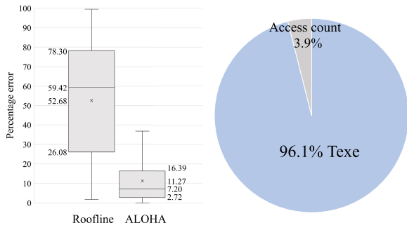
(a) Prediction error distribution for the Roofline and in energy estimation based on ALOHA models. (b) Contributions to the error in energy estimation based on the Roofline model.
