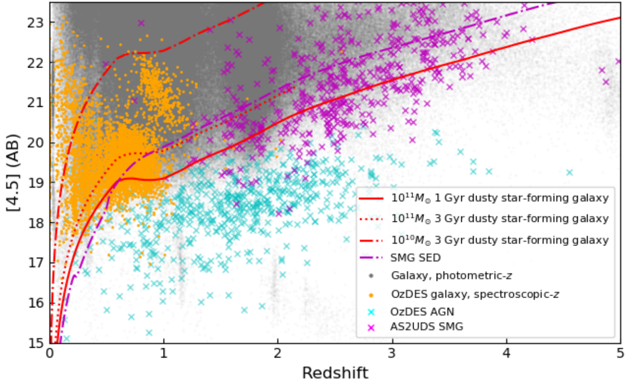
Figure 7. Magnitude versus redshift in [4.5] (symbols as for Figure 6). Also plotted are two instances of the 3 Gyr old dusty star-forming galaxy model in Figure 6 with stellar masses of 10^{10} M_{\odot} and 10^{11} M_{\odot} , and a 1 Gyr dusty galaxy model with 10^{11} M_{\odot} from the same library, along with the composite submm galaxy SED from A2SUDS.
