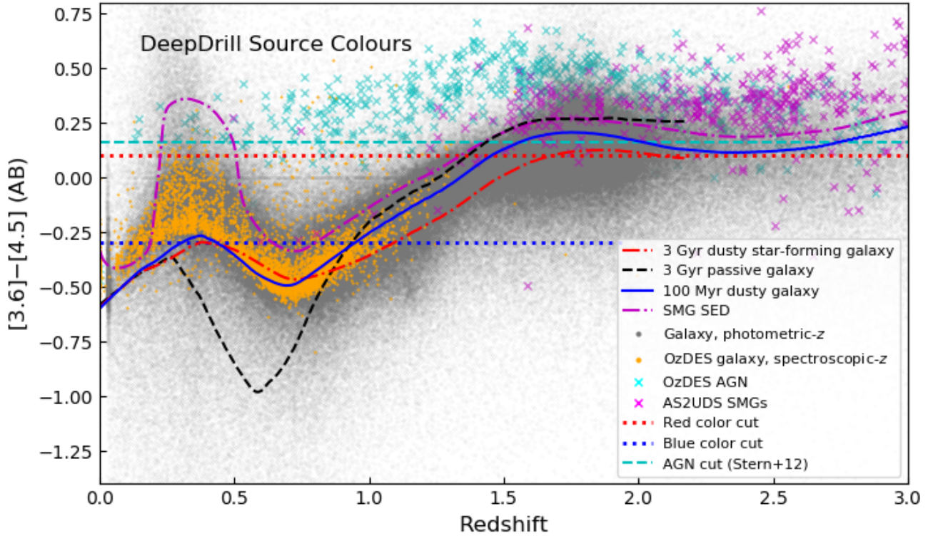
Figure 6. [3.6] - [4.5] colours of galaxies as a function of redshift (cf. Papovich 2008). The grey dots show the galaxies with photometric redshifts in the XMM-LSS field (Krefting et al. 2020), spectroscopic galaxy targets from the OzDES survey (Childress et al. 2017) (OzDES LRG, ClusterGalaxy, RedMaGiC, BrightGalaxy, Emission Line Galaxy and Photo-z types) are shown as orange dots, AGN_monitoring targets from OzDES are shown as cyan crosses, and A2SUDS submm galaxies with photometric redshifts as magenta crosses. The lines indicate various color cuts; the “Blue cut” (blue dotted line) is the line below which the blue population of Figure 8 (d) is selected; “red cut” (red dotted line) the line above which the red population of Figure 8 (d) is selected. We also include the [3.5] - [4.6] color cut of Stern et al. (2012) (“AGN cut”; cyan dashed line), above which candidate AGN dominate in the much shallower WISE survey. Three models based on Maraston (2005) evolutionary synthesis models (see Guarnieri et al. 2019) are shown, a 3 Gyr old dusty star-forming galaxy, a 3 Gyr passive galaxy and a 100 Myr galaxy. (Note that the 3 Gyr models do not extend beyond z = 2.17 , where the age of the Universe is 3 Gyr.) We also plot the composite SED of the A2SUDS submm galaxies from Dudzevičiūtė et al. (2020).
