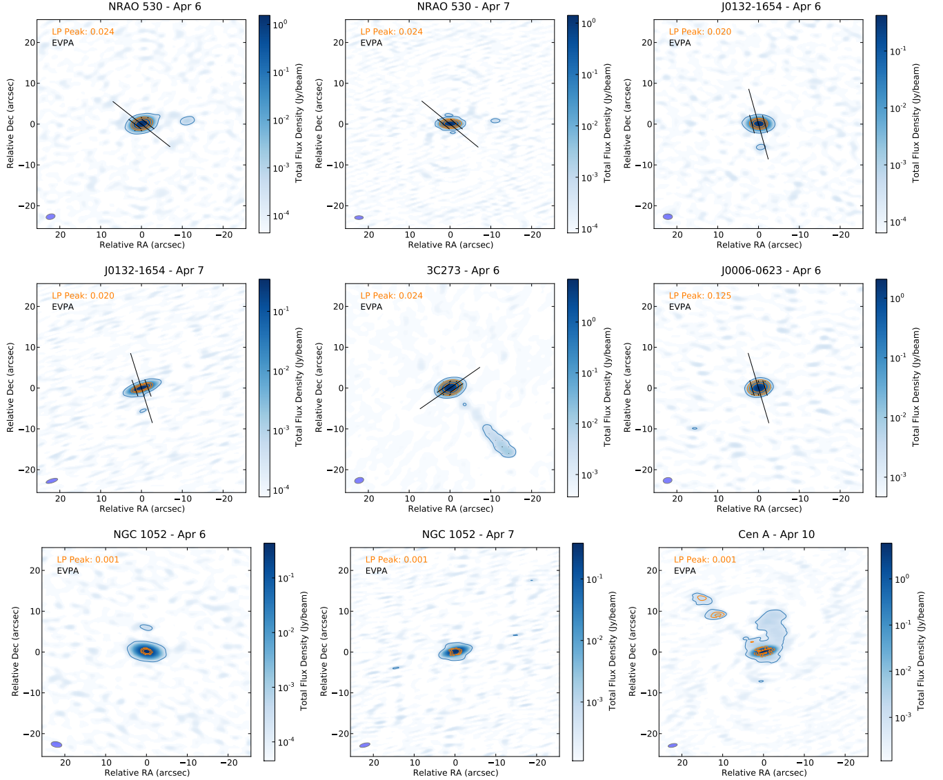
Figure 12. Polarization images of selected AGNs at 1.3 mm (see Figure 2 for a description of the plotted quantities). Note that for NGC 1052 and Cen A no EVPA could be reliably derived owing to their low level of LP. We also note that although we detect polarized flux in Cen A above the image RMS noise cutoff ( 5\sigma ), once the systematic leakage (0.03% of I onto QU ) is added to thermal noise, the LP flux would fall below the 3\sigma detection threshold. Therefore we do not claim detection of polarized emission in Cen A.
