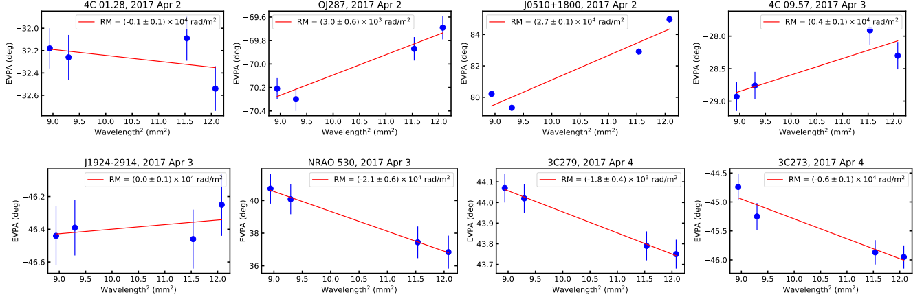
Figure 19. RM fits for the 2017 GMVA targets with EVPA measurements at 3 mm (see Table 1).
