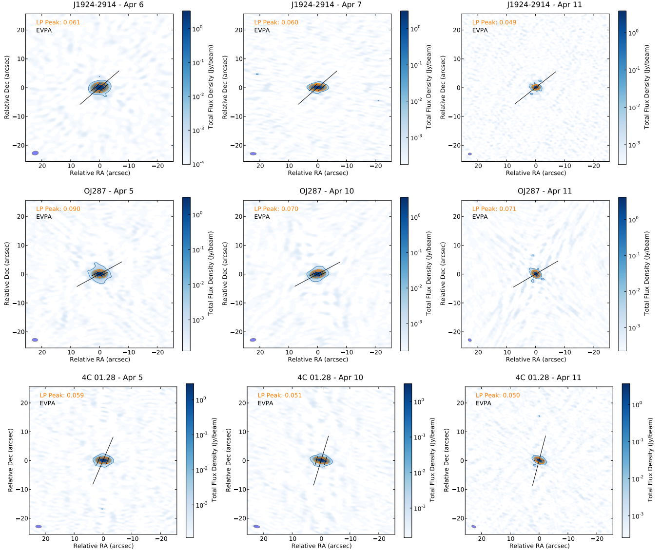
Figure 11. Polarization images of selected AGNs at 1.3 mm (see Figure 2 for a description of the plotted quantities).
