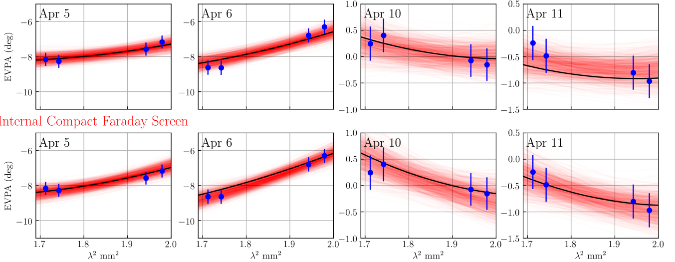
Figure 26. EVPA as a function of \lambda^2 for 10^3 draws from the two-component model posterior of the external (top) and internal (bottom) Faraday screen models. The highest-likelihood models are shown by the black lines. The blue data points are the ALMA measurements (same as Fig. 17).
