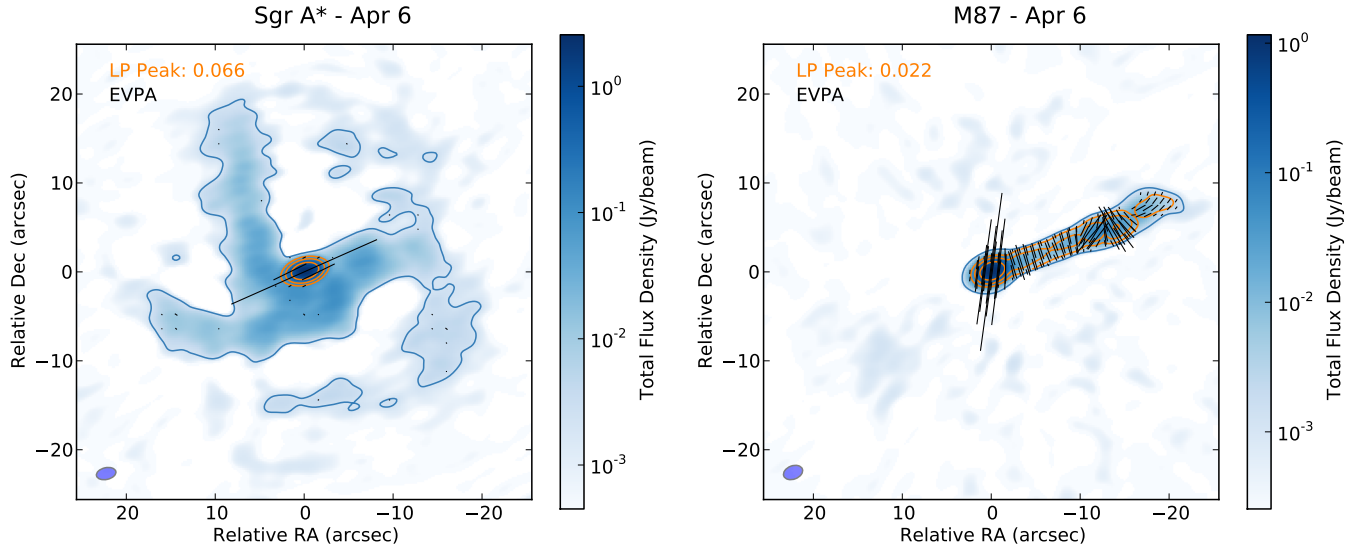
Figure 2. Polarization images of Sgr A* (left panel) and M87 (right panel) at 1.3 mm on Apr 6 2017. The raster image and blue contour show the total intensity emission, the orange contours show the linearly polarized emission, and the black vectors showcase the orientation of the EVPAs (their length is linearly proportional to the polarized flux). The total intensity brightness is plotted using a logarithmic weighting function (starting from the 1\sigma -level), the blue contour corresponds to 5\sigma (where \sigma is the Stokes I map RMS), while the orange contour levels are 5\sigma \times 2^n (where \sigma is the LP map RMS and n=0,1,2,3... up to the peak in the image). The LP fraction at the peak of the compact core is reported in the upper left corner in each panel. The EVPAs are plotted every 8 pixels ( 1''.6 or about 1 per beam) for Sgr A* and every 4 pixels ( 0''.8 or about 2 per beam) for M87 (in order to sample more uniformly the jet). According to the measured RM, the EVPAs towards the compact core should be rotated by -23^\circ (east of north) in Sgr A* and by -16^\circ in M87. The beamsizes (shown as an oval in the lower left corner) are 2''.2 \times 1''.3 (P.A. -77^\circ ) and 2''.2 \times 1''.5 (P.A. -69^\circ ) in the left and right panels, respectively. Note that there are several tiny EVPAs plotted across the mini-spiral, apparently locating regions with polarized flux above the image RMS noise cutoff ( 5\sigma ). The LP and EVPA errors are however dominated by the systematic leakage (0.03% of I onto QU), which is not added to the images. Once these systematic errors are added, the LP flux in those points falls below the 3\sigma measurement threshold. Therefore we do not claim detection of polarized emission outside of the central core in Sgr A*. Besides, only the polarisation within the inner 1/3 of the primary beam is guaranteed by ALMA. The full set of 1.3 mm observations of Sgr A* and M87 are reported in Figures 8 and 9, respectively.
