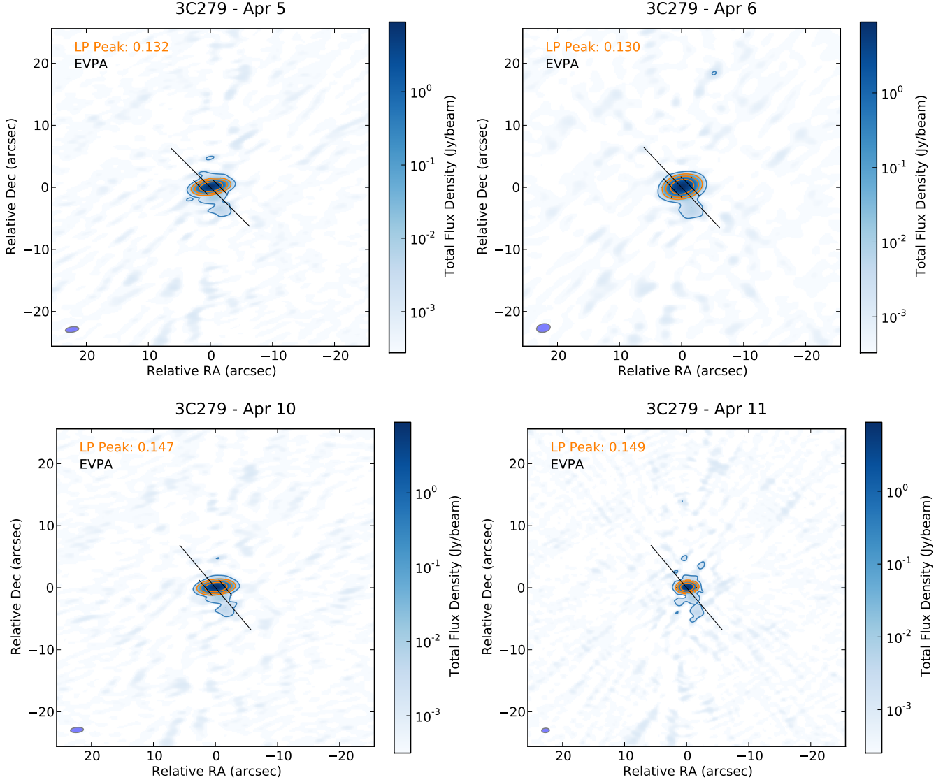
Figure 10. Polarization images of 3C279 at 1.3 mm (see Figure 2 for a description of the plotted quantities).
