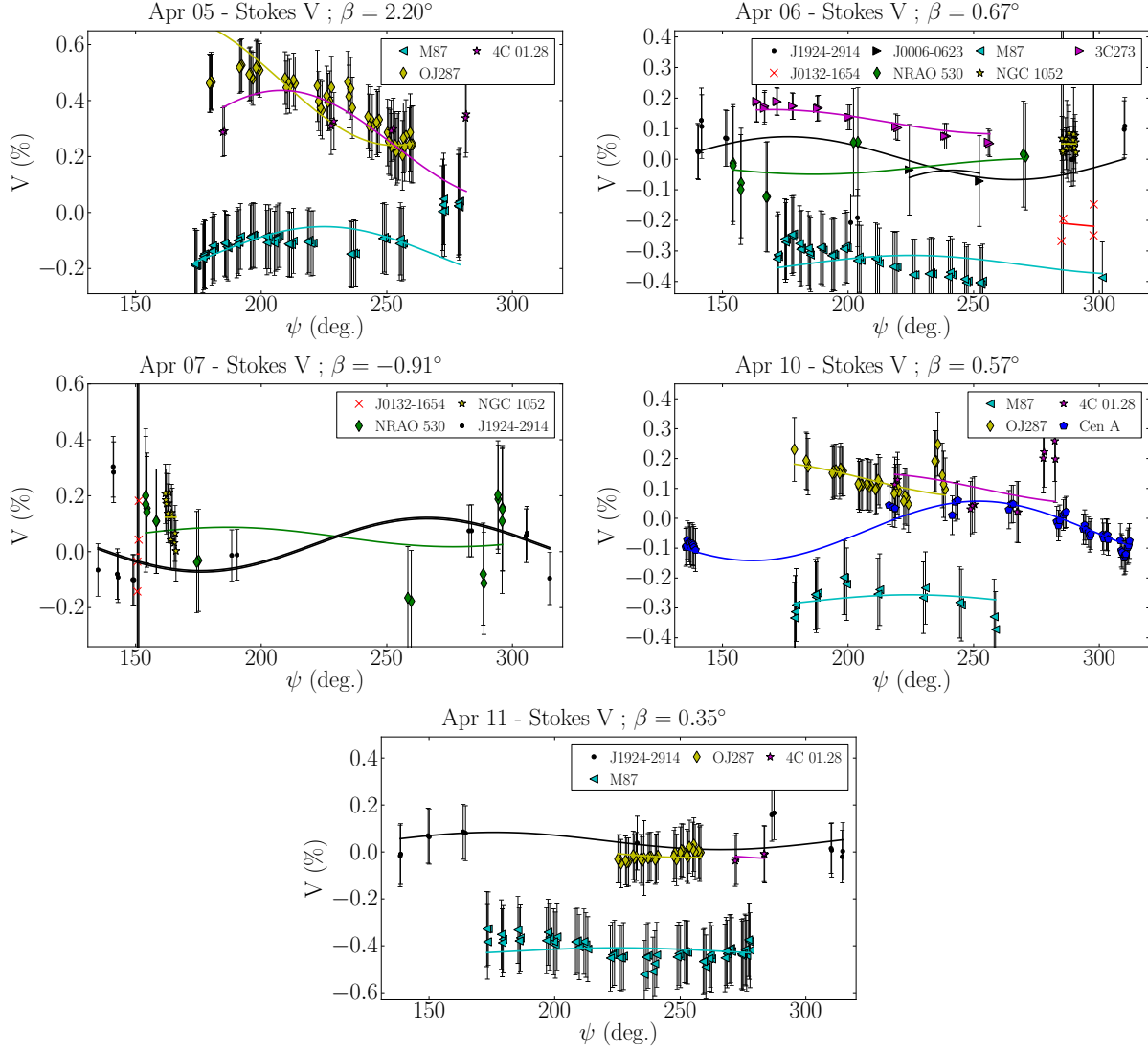
Figure 22. Reconstructed fractional Stokes V of all sources (but 3C 279), as a function of feed angle, during the EHT campaign. Stokes V is computed as the real part of (XY^* - YX^*)/j . Continuum lines show a simplified model based on cross-polarization phase offsets at ALMA, which have been fixed to the \beta values shown on top of each figure. Note that Sgr A* is not plotted because it displays significant intrinsic variability on the timescales (of hours) plotted here (e.g., Bower et al. 2018).
