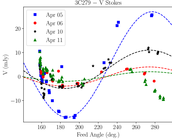
Figure 21. Reconstructed Stokes V of 3C 279 as a function of feed angle, \phi , during the EHT campaign. Stokes V is computed as the real part of (XY^* - YX^*)/j . Dashed lines show the simplified model of Eq. G2, based on cross-polarization phase offset, \beta , of the phased-ALMA reference antenna.
