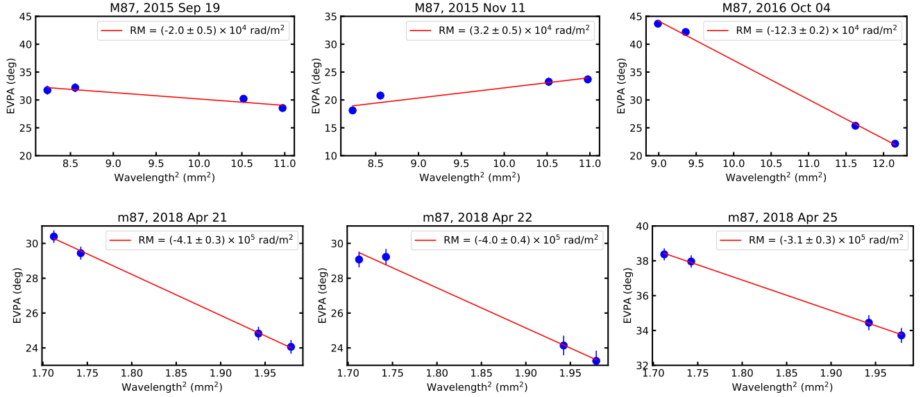
Figure 20. RM of M87 from observations carried out in Sep & Nov 2015 and Oct 2016 at 3 mm (top row) and in Apr 2018 at 1.3 mm (bottom row). Plots in both rows span the same vertical axis range ( 25^\circ and 8^\circ respectively) in order to highlight differences in slope (but note the different EVPA values in different panels).
