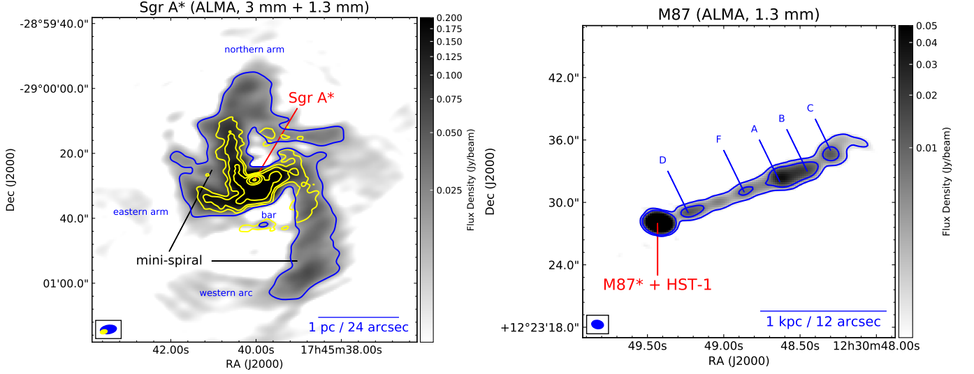
Figure 1. Representative total intensity images. Left panel: Image of Sgr A* at 3 mm on Apr 3 (grey-scale and blue contour) and at 1.3 mm (yellow contours) on Apr 6 2017. The image showcases the well-known “mini-spiral” structure surrounding the central compact core, including the eastern and northern arms, the western arc, and the bar at the center. The contour levels at 1.3 mm are 5\sigma \times 2'' where \sigma = 0.44 \text{ mJy beam}^{-1} and n = 0, 1, 2, 3 \dots up to the peak flux-density; the contour level at 3 mm corresponds to 20\sigma ( \sigma = 0.8 \text{ mJy beam}^{-1} ). The peak flux-density is 2.5 \pm 0.1 ( 2.6 \pm 0.3 ) \text{Jy beam}^{-1} and the integrated flux density across the entire source is 9.9 \pm 0.5 ( 4.9 \pm 0.5 ) Jy at a representative frequency of 93 (221) GHz. The FOV is given by the primary beam in Band 3 ( \sim 60'' ) and 1 pc corresponds to 24'' . The beamsizes are 5''.0 \times 2''.7 (P.A. = -81.1^\circ ) in Band 3 and 2''.2 \times 1''.3 (P.A. = -77.5^\circ ) in Band 6, shown as a blue and yellow ovals, respectively, in the lower left corner. Right panel: Image of M87 at 1.3 mm on Apr 11 2017. The image showcases the structure of the kpc-scale relativistic jet comprised of a bright core at the nucleus and the knots along the jet labeled as D, F, A, B, C; HST-1 is not resolved from the nucleus in these images. The RMS noise level is 0.16 \text{ mJy beam}^{-1} , and the contour levels are a factor of 10 and 40 of the RMS. The peak flux-density is 1.34 \text{ Jy beam}^{-1} and the integrated flux-density is 1.57 \text{ Jy} at a representative frequency of 221 GHz. The FOV is given by the primary beam in Band 6 ( \sim 27'' at 1.3 mm). 1 kpc corresponds to 12'' . This observation was conducted with the most extended array during the VLBI campaign, yielding the highest angular resolution (beam size = 1''.2 \times 0''.8 , P.A. = 79.3^\circ , shown in the lower left corner). In both panels the four observing SPWs (see § 2.1) were used together for imaging. The intensity brightness is plotted using a logarithmic weighting function (starting from the 5\sigma -level), in order to highlight the full extent of both the mini-spiral (in Sgr A*) and the jet (in M87).
