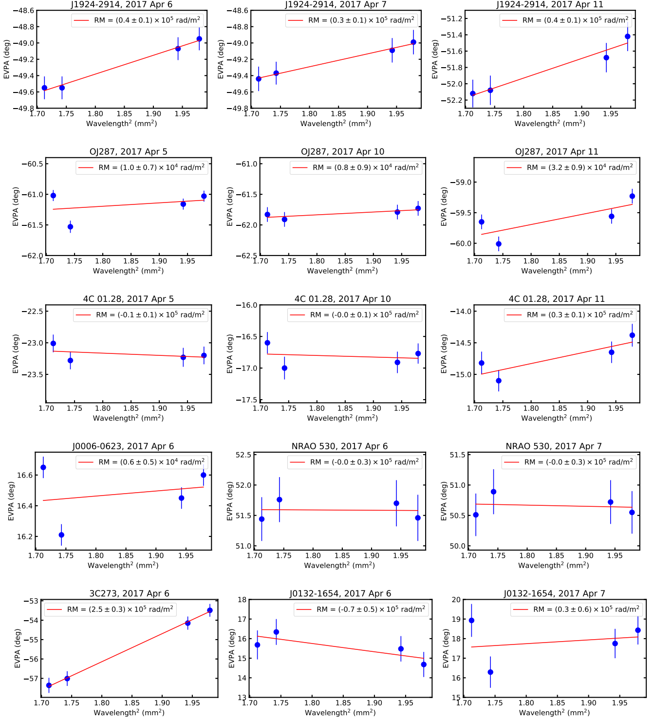
Figure 18. RM fits for remaining 2017 EHT targets with EVPA measurements at 1.3 mm (see Table 2). Plots in each row span the same vertical axis range for the same source in order to highlight differences in slope.
