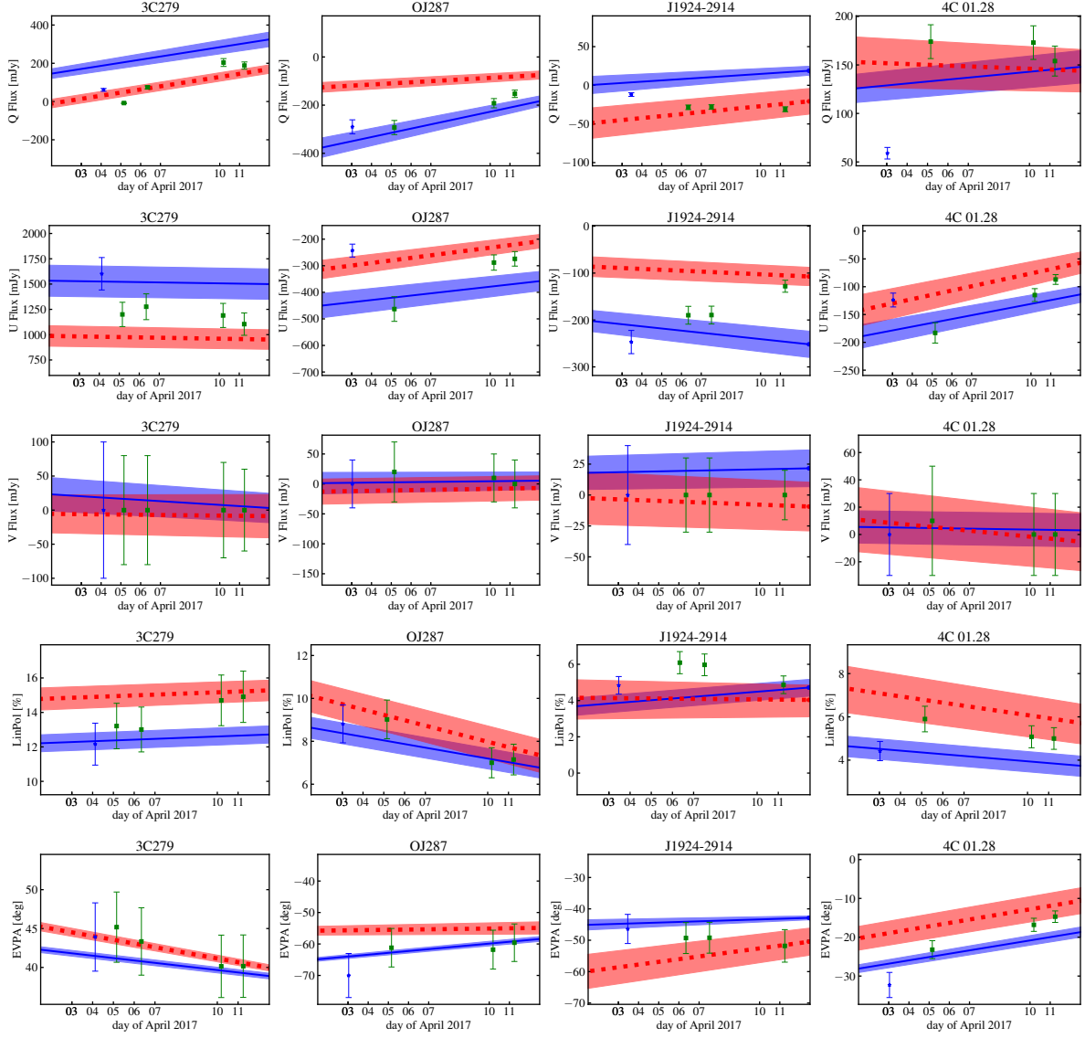
Figure 15. Comparison with time between the polarimetric results obtained for all the sources observed in the ALMA-VLBI campaign and those retrieved from the AMAPOLA polarimetric analysis of Grid Survey data. Each row shows a parameter (from top to bottom: Stokes Q, U, and V, LP, and EVPA) while each column corresponds to a source (from left to right: 3C279, OJ287, J1924-2914, and 4C 01.28; see Figure 16 for more). Only sources with entries in the ALMA archive (close in time to the observations, i.e., between end of March and April 2017) are displayed. The measured flux values during the ALMA-VLBI observations are indicated as data points and corresponding errorbars (blue and green for Band 3 and 6 observations, respectively). The shaded regions indicate AMAPOLA's \pm 1\sigma uncertainty in Band 3 (97.5 GHz; blue shade) and Band 7 (343.4 GHz; red shade), respectively. These are obtained from the ACA GS and their time evolution (lines) are obtained by interpolating between these measurements.
