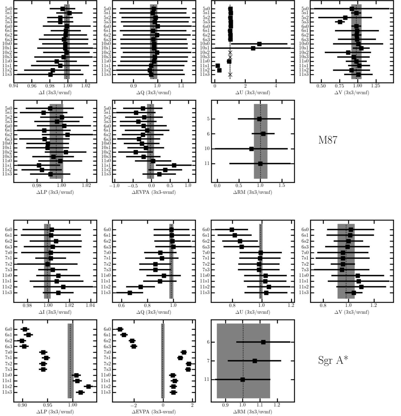
Figure 14. Comparison between image-based and uv -based flux-extraction methods for the two sources with the most prominent extended emission in our sample: M87 (top panels), and Sgr A* (bottom panels). The two methods being compared are: UVMULTIFIT (UVMF) and the sum of the nine central pixels (3x3) of the model image. All parameters are compared via ratios, except for the EVPA (showing the difference in degrees). The errorbar in each data-point is the combination in quadrature of the statistical error from each flux extraction method. The vertical dotted line and the shaded region show the median and MAD from Table 8. The labels in the Y-axis indicate the observing day in April 2017 (5, 6, 7, 10, 11) and the observing SPW (s1, s2, s3, s4); the RM panel shows only the days. Non-detections in the images are indicated with a cross. Note that the plotted uncertainties are not those of individual measurements but ratios or differences between the two methods. Therefore the errors on LP and EVPA for M87 on Apr 10/11 appear comparable to other days despite the large error bars and/or non detections in Stokes U (i.e. the errors in U displayed do not propagate in the LP and EVPA plots).
