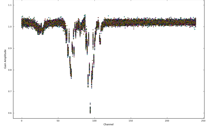
Figure 23. Bandpass for Sgr A* core (after removing instrumental bandpass with the calibrator NRAO 530) for 2017 Apr 07 observations. Only baselines longer than 60-m were used to remove virtually all of the extended arc-second emission. For each channel, every antenna bandpass amplitude is plotted (represented by different colors). All three April observations show virtually the same ‘bandpass’.
