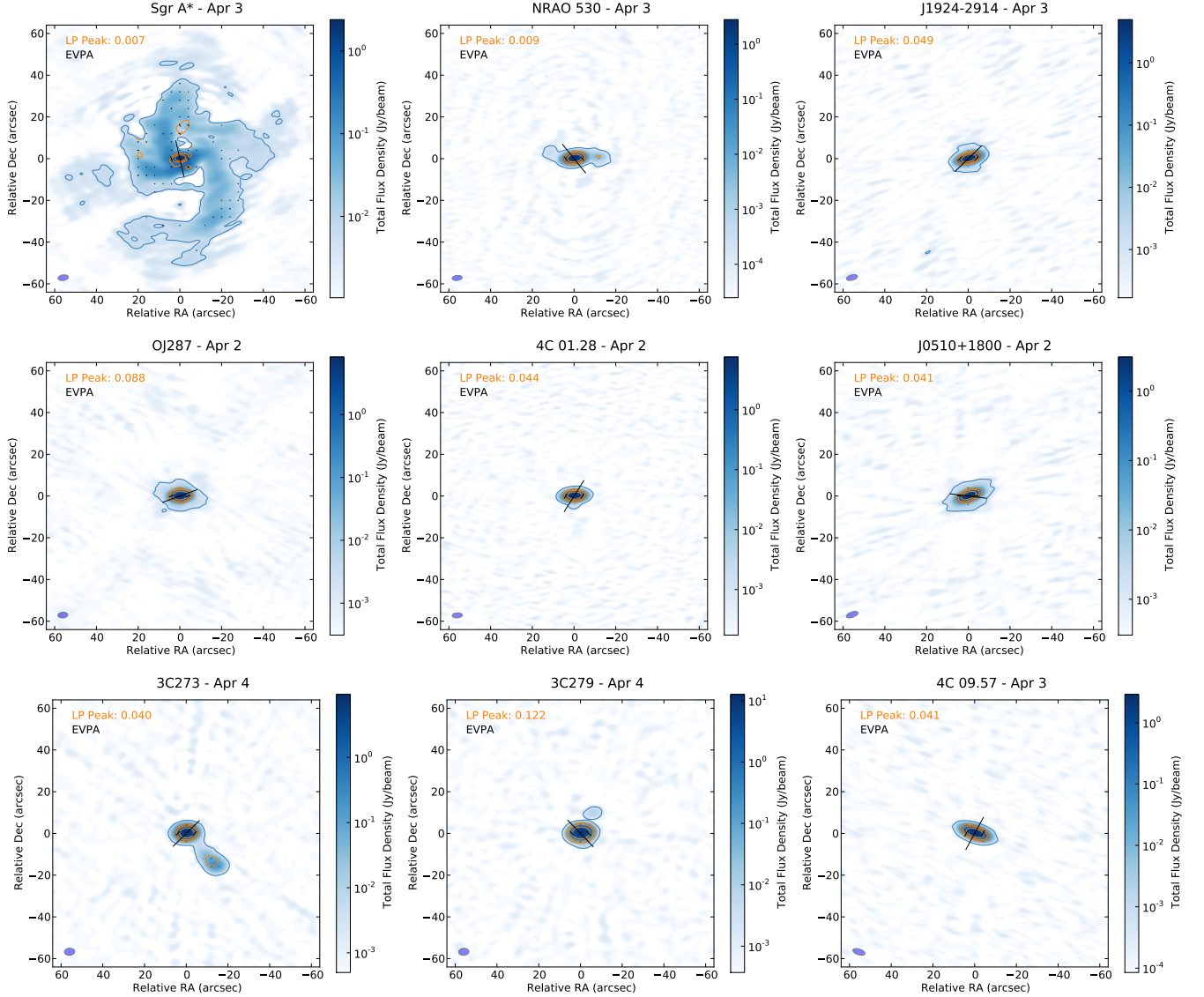
Figure 13. Polarization images of all targets observed at 3 mm (at a central frequency of 93 GHz). The beamsizes are shown as an oval in the lower left corner of each panel (see values reported in table 6). See Figure 2 for a description of the plotted quantities.
