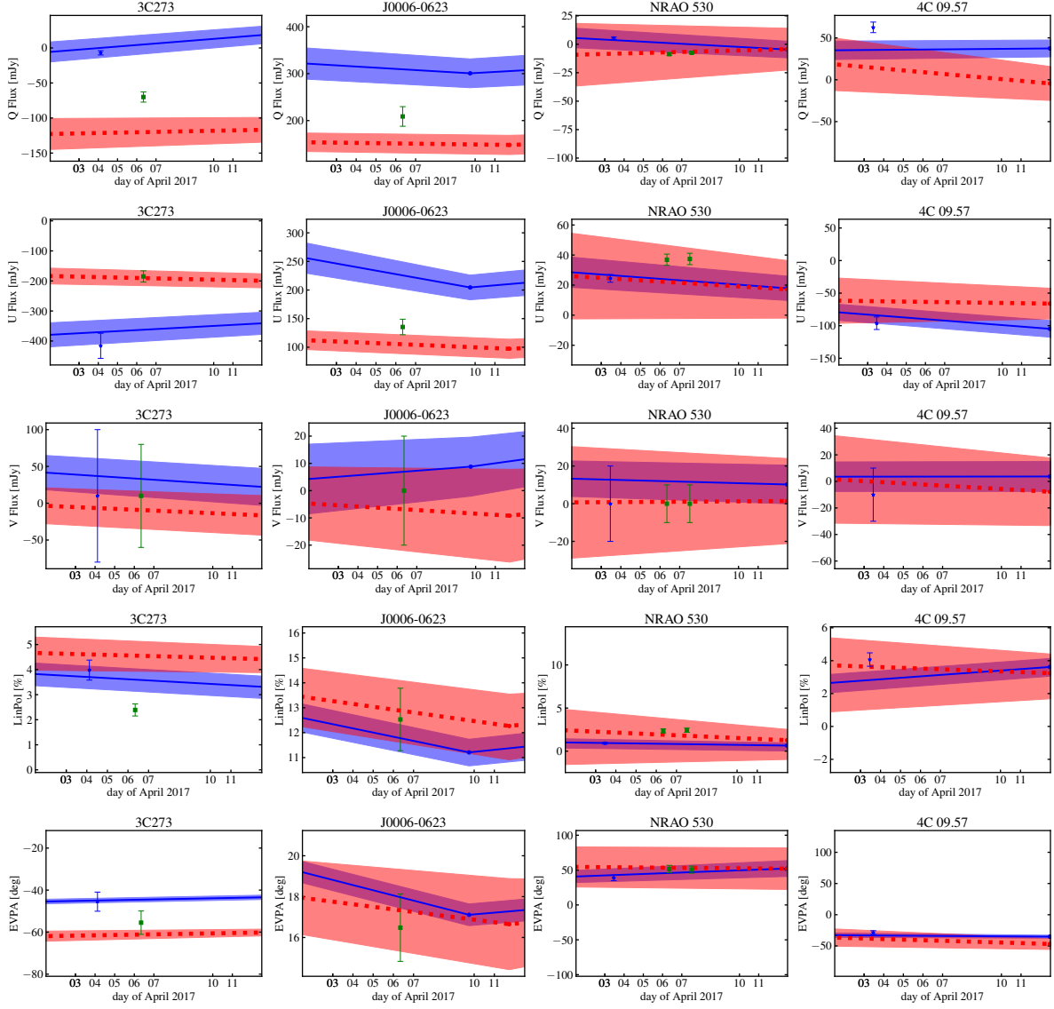
Figure 16. Same as Fig. 15, but for different sources (from left to right: 3C273, J0006-0623, NRAO 530, 4C 09.57). We note that source J0006-0623 was observed on Apr 7 but the calibrated data were of poor quality and were flagged before analysis (see § 2.2).
