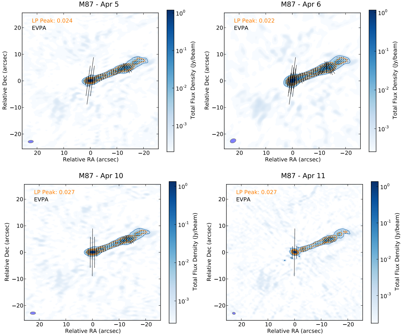
Figure 9. Polarization images of M87 at 1.3 mm (see Figure 2 for a description of the plotted quantities). The apparently different jet structures (in total and polarized intensity) across days are due to different beamsizes (shown as ovals in the lower left corner of each panel; see values reported in Table 7).
