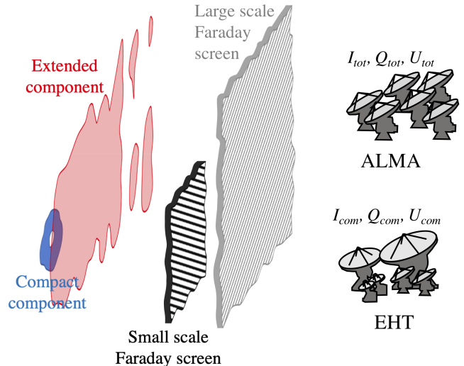
Figure 6. Diagram of the two-component model, comprised of a compact (blue) and extended (red) polarized emission regions with corresponding small-scale and large-scale Faraday screens. The small-screen, which may be external (shown) or internal (not shown) acts only on the compact component, which is observed by the EHT. ALMA observes the combined emission from both components.
