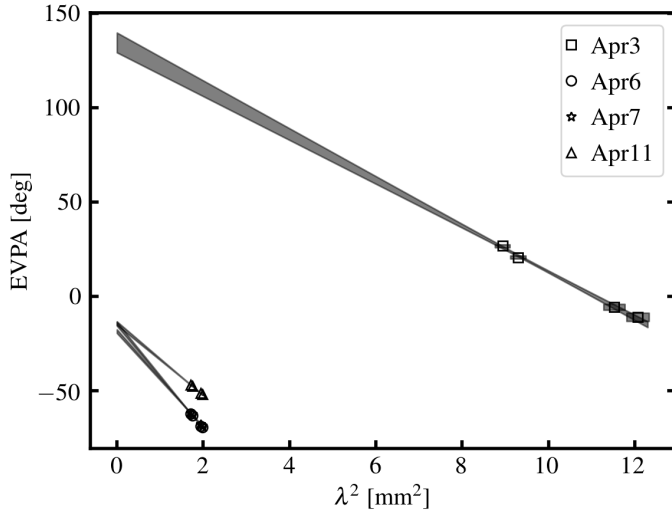
Figure 5. Sgr A* EVPA as a function of \lambda^2 observed in 2017 at 3 mm (Apr 3) and 1.3 mm (Apr 6, 7, 11). Each grey line is a linear fit to the EVPAs measured at the four ALMA Band 3 and Band 6 SPWs, yielding the RM in each epoch, and the extrapolated intercept at the Y-axis is \chi_0 . Note the large offset in \chi_0 between the 3 mm and 1.3 mm bands, despite the consistency of \chi_0 at 1.3 mm across 6 days.
