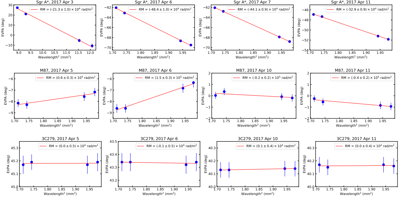
Figure 17. Faraday RM of Sgr A* (upper panels), M87 (middle panels), and 3C 279 (lower panels). The EVPA as a function of wavelength-squared is presented with 1\sigma error bars for each SPW and for each day. The EVPAs are measured in the 1.3 mm band, except for the upper left panel, presenting the EVPAs measured at 3 mm in Sgr A*. The error bars are derived adding in quadrature to the thermal uncertainty of the Q and U maps ( 1\sigma image RMS) a systematic error of 0.03% of Stokes I (error bars for Sgr A* are smaller than the displayed points). The line is a linear fit to the data giving the RM reported inside the box. Plots in each row span the same vertical axis range in degrees in order to highlight differences in slope (the upper left panel is an exception). It is remarkable that Sgr A* showcases a very consistent slope across days, while in M87 the slope appears to change sign. Note also the different EVPA values between Apr 6/7 and Apr 11 in Sgr A* and between Apr 5/6 and Apr 10/11 in M87 and 3C279. The measured RM in 3C 279 (used as polarization calibrator on Apr 5, 6, 10, and 11) is consistent with zero across all days, demonstrating the stability of the polarization measurements on M87 and on Sgr A* on the same days.
