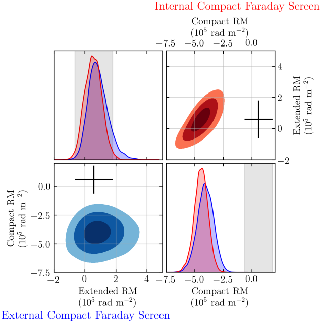
Figure 7. Posteriors implied by the April 5, 6, 10, and 11, 2017 ALMA and EHT observations for the RMs measured on ALMA (extended) and EHT (compact) scales in the two component model when it is assumed that the compact Faraday screen is external (lower left, blue) and internal (upper right, red) to the emission region. Contours are shown for the 50%, 90%, and 99% quantiles. For comparison, the 2\sigma range of April 5, 6, 10, and 11, 2017 ALMA RMs reported in Table 3 are shown by the black crosses and gray bands.
