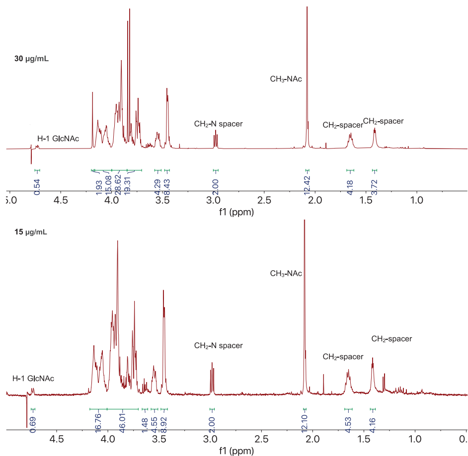
Figure 5. Partial ^1\text{H} NMR spectra of the 30 \mu\text{g/mL} - and 15 \mu\text{g/mL} TarS glycosylation of compound 3 . All spectra were measured in \text{D}_2\text{O} on a 500 MHz NMR at 25^\circ\text{C} .
