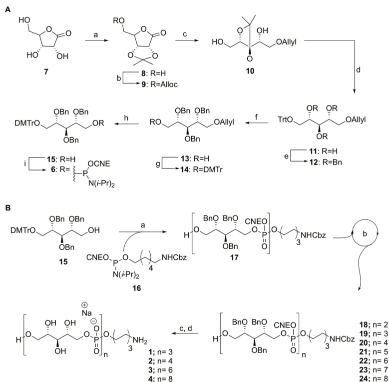
Scheme 1A. Ribitol building block synthesis; Reagents and conditions : a) HCl, acetone, 77%; b) AllocCl, pyridine/ACN, 80%; c) i. Pd(PPh 3 ) 4 , dioxane, reflux, ii. NaBH 4 , THF, 55°C, MeOH, 85%; d) i. AcOH/H 2 O, 50°C, ii. TrtCl, pyridine, 99%; e) BnBr, NaH, THF/DMF 68%; f) AcOH/H 2 O, 80°C, 70%; g) DMTrCl, TEA, DCM, quantitative; h) i. Ir(COD)(Ph 2 MeP) 2 PF 6 , H 2 , THF, ii. I 2 , sat. aq. NaHCO 3 , THF, 79%; i) 2-cyanoethyl- N,N -diisopropylchlorophosphoramidite, DIPEA, DCM, 79%; Scheme 1B. Assembly of aminospacer functionalized RboP WTAs; Reagents and conditions : a) i. DCI, ACN, 16 ; ii. CSO; iii. 3% DCA in DCM, 18 ; 74%, 19 ; 88%, 20 ; 80%, 21 ; 76%, 22 ; 91%, 23 ; 85%, 24 ; 86%; b) i. DCl, ACN, 6 , ii. CSO, iii. 3% DCA in DCM, 18 ; 74%, 19 ; 88%, 20 ; 80%, 21 ; 76%, 22 ; 91%, 23 ; 85%, 24 ; 86%; c) NH 3 (30-33% aqueous solution), dioxane; d) Pd black, H 2 , AcOH, H 2 O/dioxane, 1 : 87%, 2 : 75%, 3 : 87%, 4 : 89%.
