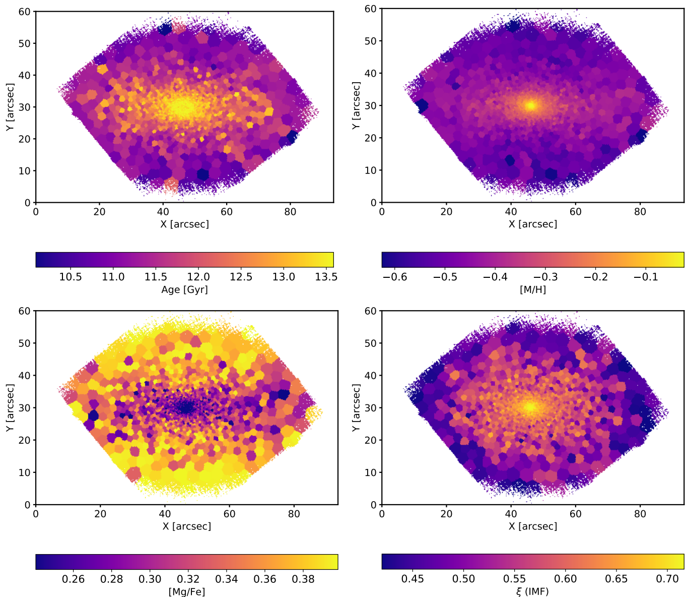
Fig. 2. F3D stellar population maps. From left to right and top to bottom we show the age, metallicity, [Mg/Fe] , and IMF slope maps of FCC 083, a typical ETGs in our sample. Age and metallicity exhibit clear negative gradients, while [Mg/Fe] tends to increase with radius. There is also a clear gradient in the IMF map, becoming steeper in the central regions.
