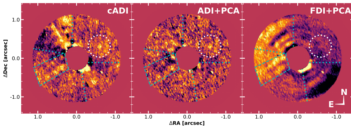
Figure 2. The final post-processed images obtained with MagAO+vAPP, as processed using the cADI (left), ADI+PCA (middle), and FDI+PCA (right) algorithms, and covering a total integration time of 14,160 seconds. The two D-shaped dark holes have been stitched together around their common centre. Residual contamination is visible where the dark holes were joined together in the form of bright and dark regions in the north-east and south-west (segments indicated by blue dotted lines). Regions inside the inner working angle of the vAPP and beyond the outer expanse of the vAPP PSF have been masked. The expected location of the companion from concurrent SPHERE observations (Maire et al. 2018) is indicated by a dotted white circle in each image. HR 2562 B is detected in the cADI and ADI+PCA images, but not in the FDI+PCA image. The non-detection in the FDI+PCA image is due to symmetry-breaking factors such as instrumental ghosts and wind-driven halo, and is discussed in Section 5.2. The characteristic butterfly pattern of wind-driven halo can be seen in the FDI+PCA image as extended bright and dark patches immediately and diagonally either side of the masked inner region. A bright spike caused by instrumental scattered light is indicated in the blue dashed box. The bright patch in the south-west is a persistent detector defect that was not removed during the data reduction process. All three images use an arbitrary logarithmic colour scale.
