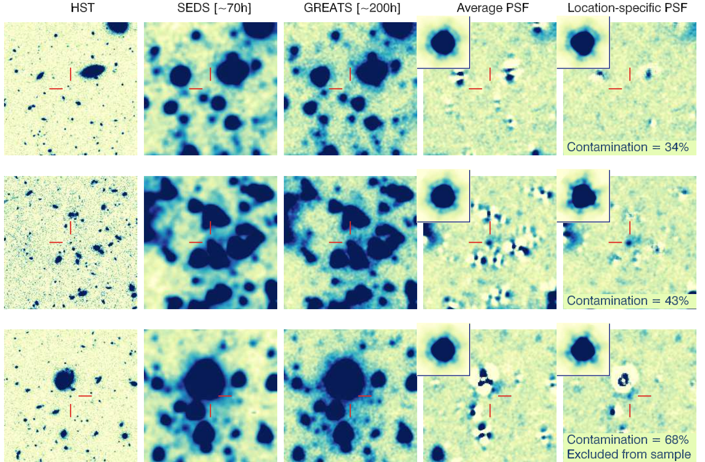
Figure 2. Illustration of our sophisticated procedures for handling the deep IRAC data used in this work. Each row refers to a specific object in the z \sim 7-8 compilation of Bouwens et al. (2015) which constitute our initial sample (top-to-bottom are GSDZ-2460945596, GNWZ-7268117400 and GSDZ-2288549126). Each stamp is \sim 30'' per side and, in each row, they match to the same region of sky. In each stamp, the location of the high- z source corresponds to the intersection of the two red segments. Left to right, columns present the combined image from HST ( J_{125} + JH_{140} + H_{160} ), an image stamp at 3.6\mu\text{m} from SEDS (Ashby et al. 2013a), which corresponds to a nominal coverage depth of \sim 70 hrs (including also the GOODS IRAC data), and the same region in the 200 hrs GREATS 3.6\mu\text{m} mosaic. In the last two columns we present our results subtracting neighbouring sources with MOPHONGO adopting, first, an average PSF and, second, the specific PSF reconstructed at the location of the source, accounting for the orientations of all contributing observations (as first pioneered in Labbé et al. 2015), respectively. The estimated contamination from neighbouring sources is reported at the bottom of the right-most panel. All IRAC stamps share the same flux density cuts. The adopted PSF is shown in the top-left corner of the corresponding stamp. As can clearly be seen in the rightmost column, the combination of increased depth and accurate PSF reconstruction from the location-specific PSF allow us to obtain more robust flux densities in the IRAC bands. The last row shows an object excluded from our final sample because of the large contamination ( > 65\% ) from the very bright neighbouring source which made the photometry more uncertain, even though the removal of the neighbours was reasonably successful.
