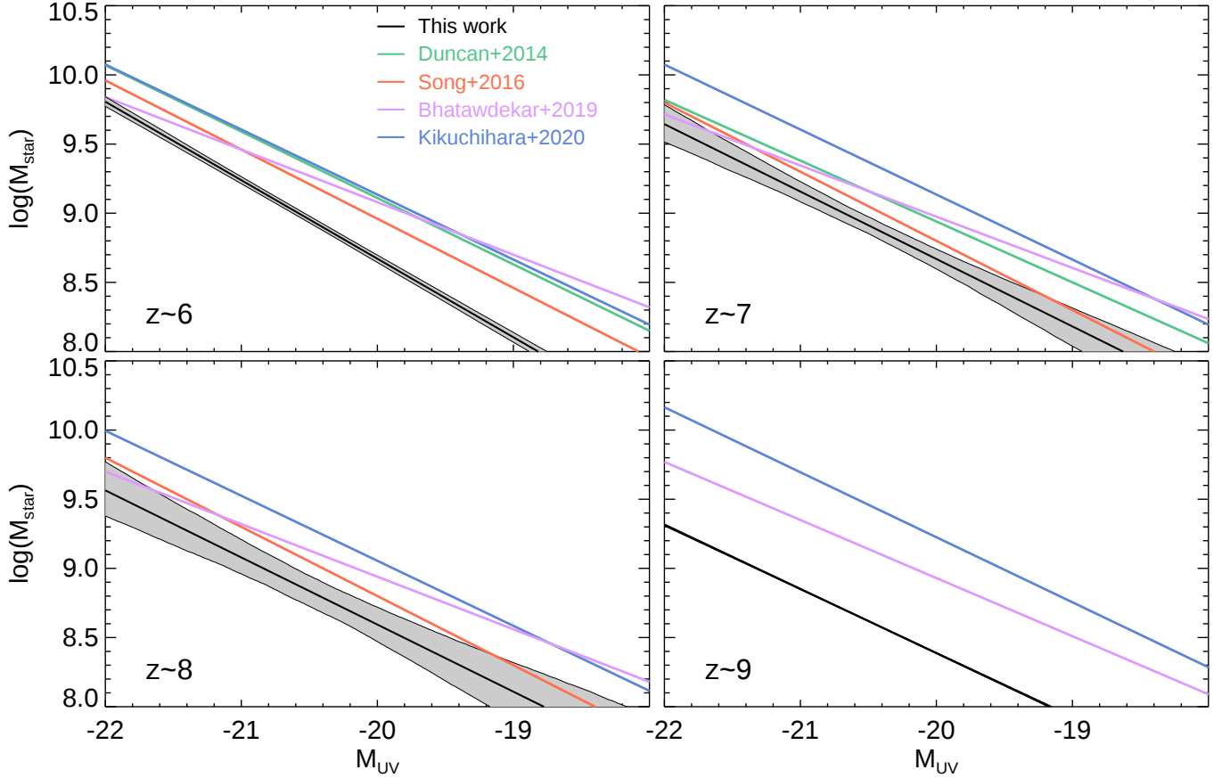
Figure 16. Comparison of our \mathcal{M}_\star - M_{\text{UV}} relation to some of the most recent estimates in the literature, as indicated by the legend in the top-left panel. The grey-shaded areas encompass the 68% confidence interval from our best-fit values. The tight relationship at z \sim 9 is likely a consequence of similar SEDs resulting from our procedure of reconstructing the flux densities in the IRAC bands discussed in Section 3.4.
