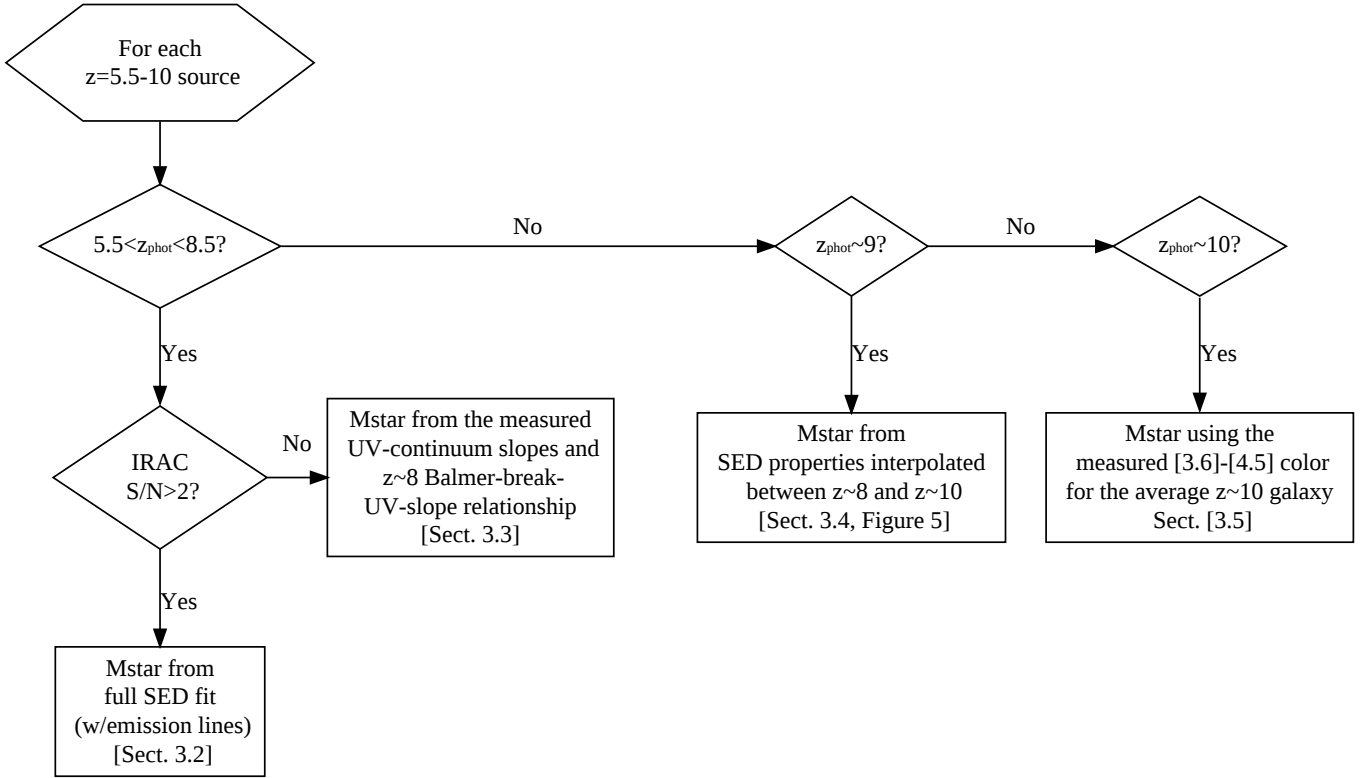
Figure 4. Flow chart summarizing the different procedures followed to estimate the total stellar mass \mathcal{M}_\star of galaxies in our sample depending on the source redshift and the significance of the IRAC detections.
