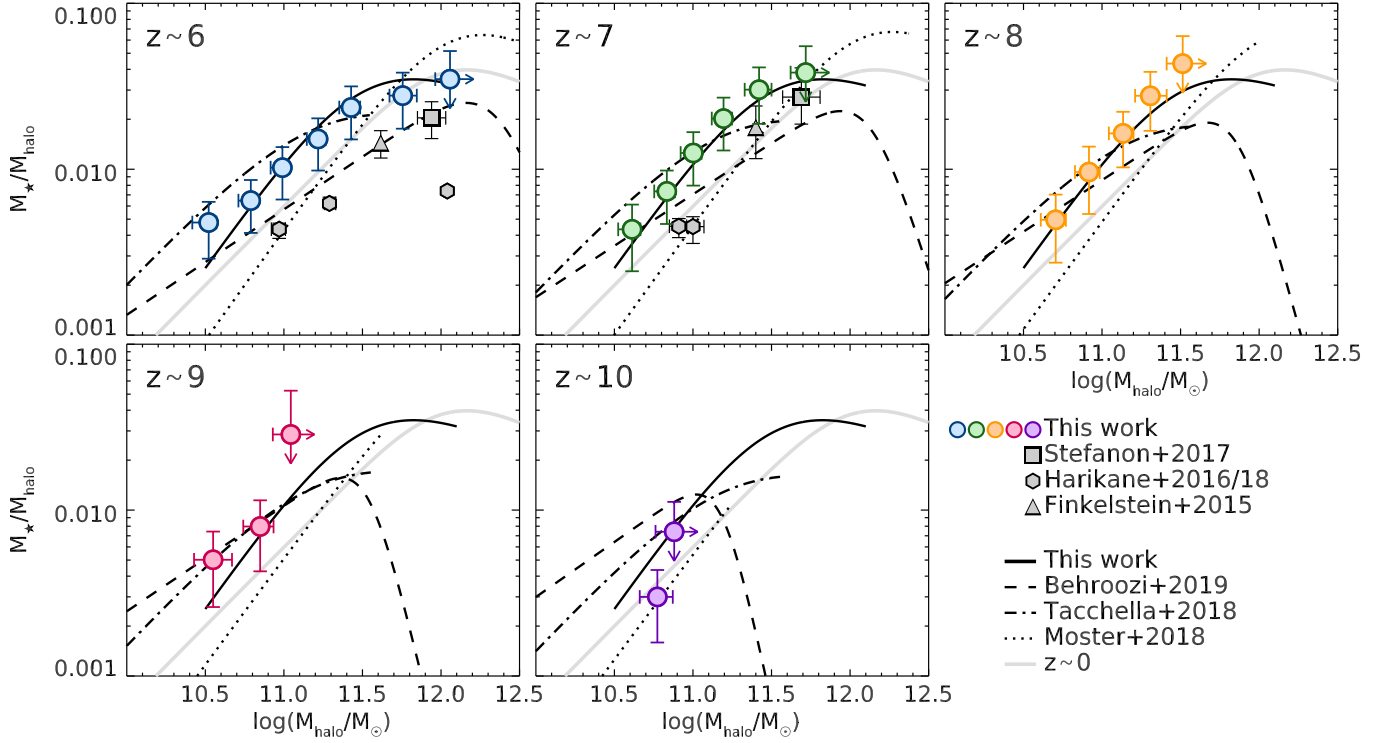
Figure 13. Comparison of the stellar-to-halo mass ratios estimated in this study to previous observational estimates of Finkelstein et al. (2015a), Harikane et al. (2016, 2018) and Stefanon et al. (2017) (symbols as per the bottom-right legend). Also presented is our redshift-independent best-fitting relation, and the redshift-evolving stellar-to-halo mass relations from the semi-analytic model of Behroozi et al. (2019), the moderately evolving SHMR of Moster et al. (2018) and the marginally evolving SHMR from the semi-analytic models of Tacchella et al. (2018) (legend at the bottom right). The grey solid curve corresponds to the z \sim 0 SHMR from Behroozi et al. (2013) that we display as reference. We used the relations derived in Appendix D to convert the halo mass estimates of Finkelstein et al. (2015a) and the curves of Tacchella et al. (2018) from a WMAP7 cosmology into one consistent with that of Planck Collaboration et al. (2016). The solid points with arrows mark those halo mass measurements whose lower uncertainty remained undefined because of the limited range available for v_{\text{acc}} . The broad agreement with the predictions with constant SHMR (see text) provide further support to a non-evolving SHMR in the early universe.
