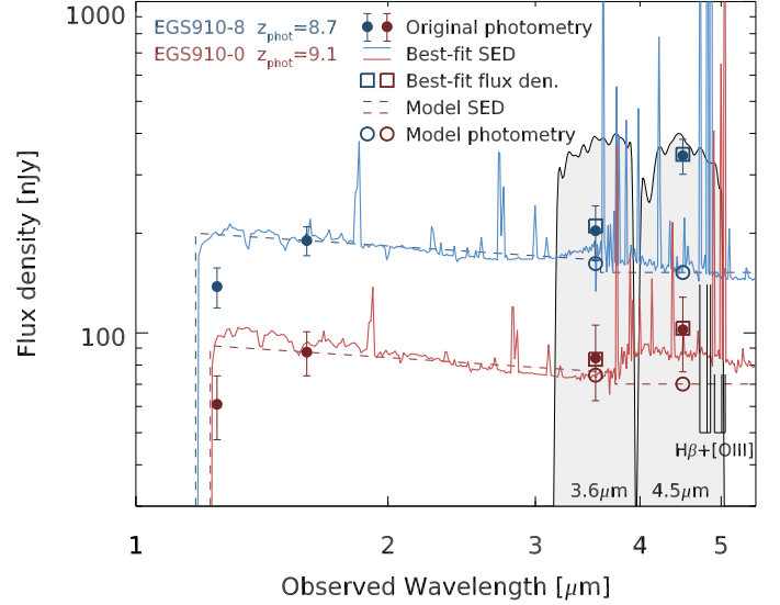
Figure 5. Illustration of the challenges we face in estimating the stellar masses of z \sim 9 sources, given the uncertain position of the Balmer break/jump and [O III]+H \beta emission lines relative to the 3.6 \mu m and 4.5 \mu m bands, and of the procedure we adopted to reduce the associated systematic effects. Presented are two distinct sources in the upper and lower halves of the redshift range of our z \sim 9 sample (EGS910-8 at z_{\text{phot}} \sim 8.7 , and EGS910-0 at z_{\text{phot}} \sim 9.1 - Bouwens et al. 2019 - blue and red, respectively). All flux densities of EGS910-0 were arbitrarily rescaled by a factor 0.7 to improve readability. The original photometric measurements are marked with filled circles, while the corresponding best-fit templates are presented as solid curves; the flux densities in the 3.6 \mu m and 4.5 \mu m bands for the best-fit templates are indicated as open squares. The two sets of vertical lines close to the bottom-right corner indicate the location of H \beta and of the [O III] doublet at the redshifts of the two galaxies. The two filled grey regions correspond to the transmission curves of the IRAC 3.6 \mu m and 4.5 \mu m bands, arbitrarily renormalized. The photometric redshift uncertainties ( \Delta z \sim 0.6-0.8 ) do not allow us to properly estimate the relative contribution of the rest-frame optical light to the observed flux density in the 3.6 \mu m band, and of some among the strongest emission lines (H \beta and [O III]) to the flux densities in the 4.5 \mu m band. These are necessary to constrain the amplitude of the Balmer Break and therefore the age of the stellar population. For each source, we therefore created a model SED (dashed curves), free from nebular lines contribution, interpolating the empirical relationships we derived from observations of z \sim 8 and z \sim 10 galaxies (see main text), and computed the expected flux densities in the IRAC 3.6 \mu m and 4.5 \mu m bands (open circles). We combined the new model photometry with the existing HST measurements to estimate the stellar masses through a new SED fit (see Section 3.4).
