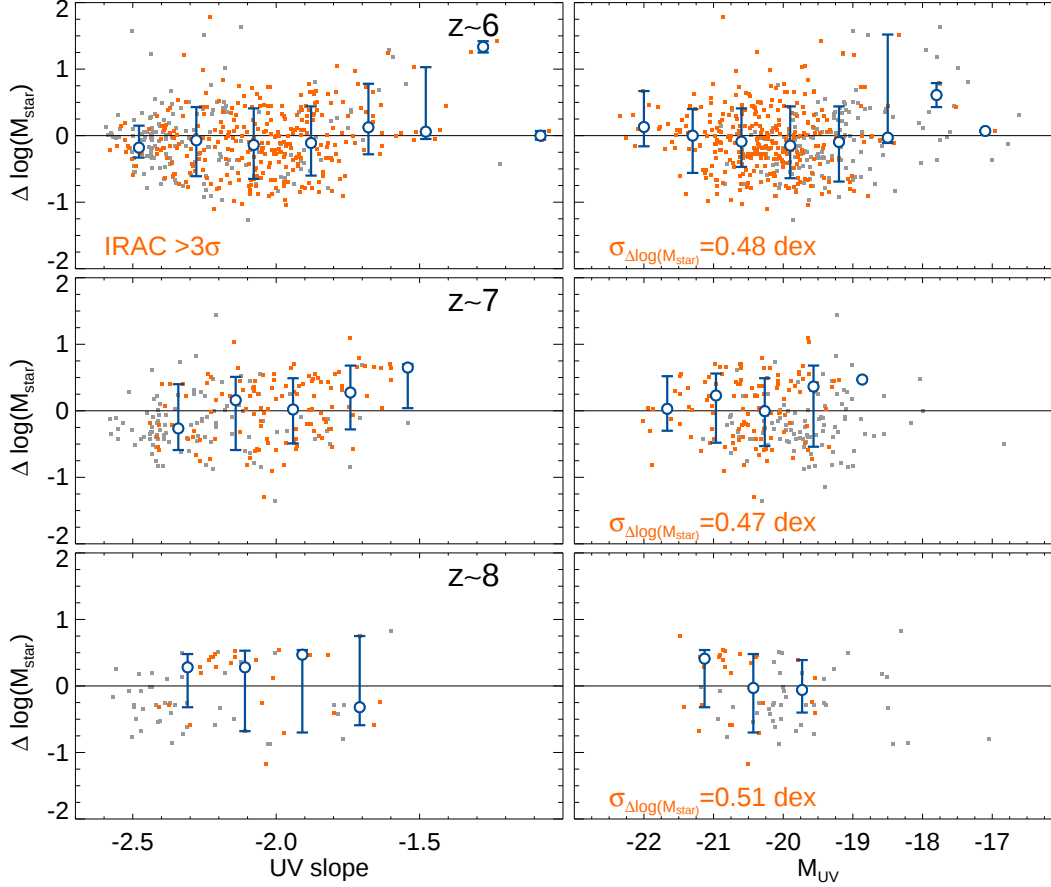
Figure 15. Comparison between the stellar mass measurements obtained with SED templates that included emission by nebular continuum and lines ( \equiv M_{\text{star,full}} ), and those where the rest-frame optical free from emission line contribution is reconstructed using the relation between the H - [3.6] color and the UV slope ( \equiv M_{\text{star,H36}} ) of Stefanon et al. (2021) . Top to bottom, the panels refer to the z \sim 6 , z \sim 7 and z \sim 8 redshift bins. For each redshift bin, the left panel presents \Delta \log(M_{\text{star}}) \equiv \log(M_{\text{star,full}}) - \log(M_{\text{star,H36}}) as a function of the UV slope, while the panels on the right present \Delta \log(M_{\text{star}}) as a function of the UV luminosity M_{\text{UV}} . Grey points correspond to the full sample, while orange points mark those sources with higher significance in the two IRAC bands, as indicated by the label in the top-left panel. Finally, the blue points with error bars correspond to the median and 68% confidence interval of the sources with higher IRAC significance. The relative consistency between our stellar mass estimates made using the full SED information for IRAC-detected sources and estimates made relying on the UV slope information alone (exploiting a relationship we found in Stefanon et al. 2021 ) gives us confidence in using this prescription for sources lacking clear 2\sigma detections with IRAC.
