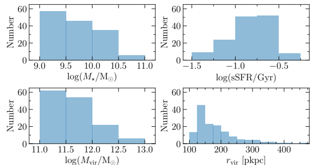
Figure 1. Distributions of stellar mass M_* , specific star formation rate (sSFR), halo virial mass M_{\text{vir}} , and virial radius r_{\text{vir}} of the selected central, star-forming galaxies. The sample consists of 144 star-forming galaxies.
